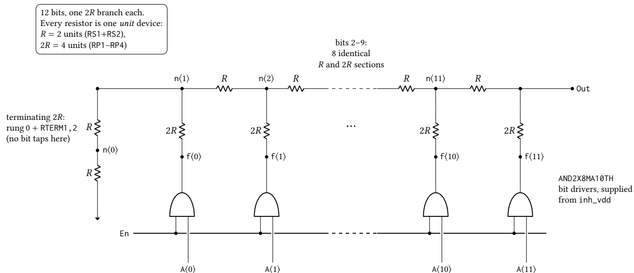
Figure 69: The 12-bit voltage-mode R - 2R ladder of anatop_pixel_dacR2R12 , transcribed from the DacNonlinTB netlist. Bit k drives tap n\langle k+1 \rangle through its own 2R branch, so the twelve taps are n\langle 1 \rangle – n\langle 11 \rangle plus Out , and the MSB branch lands directly on Out at the top of the ladder; n\langle 0 \rangle carries no bit, its rung and RTERM1, 2 together forming the terminating 2R . Bits 2–9 are elided: eight further sections identical to those drawn sit between n\langle 2 \rangle and n\langle 11 \rangle . Every element is the same unit resistor, so the network itself is exact and gives \text{Out} = (\text{code}/4096) V_{\text{ref}} ; the reference is the output high level of the AND2X8MA10TH drivers, which sit in series with each 2R branch and bound the ladder in place of the rails — measured zero scale is 90\ \mu\text{V} above V_{\text{SS}} and full scale 103\ \mu\text{V} below the ideal (4095/4096) V_{\text{ref}} on a 2.5 V rail. Device dimensions are proprietary and are not stated.
