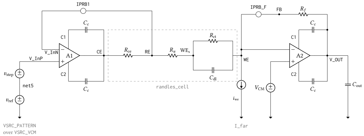
Figure 49: The complete rev-2 potentiostat pixel as simulated, tb_anatop_pixel view PotFbTB : control amplifier A1 drives the counter electrode and closes its loop on the reference electrode, while transimpedance amplifier A2 holds the working electrode at V_{CM} and returns the cell current through R_f to V_{OUT} . Both amplifiers are the same anatop_tia_amp_ab class-AB cell, each with its own external compensation capacitors C_c = 500 fF from pins C1/C2 onto its own output; supplies, En and the shared local bias generator are omitted. IPRB1 and IPRB_F are 0 V current probes inserted only so that stb can break the control loop and the transimpedance loop respectively – they add no impedance and no offset. I_{far} injects the accuracy-truth current with positive i_{we} flowing from the working electrode to ground, so v_{out} = V_{CM} + i_{we} \cdot R_f and the measured current is the probe current in IPRB_F; the opposite source orientation inverts the sign of every accuracy number. Cell elements are R_{ce} = R_u = 1 k \Omega fixed with R_{ct} and C_{dl} swept over the electrode grid, R_f is the programmable feedback resistor (35 k \Omega to 560 k \Omega ), and C_{out} = 5 pF.
