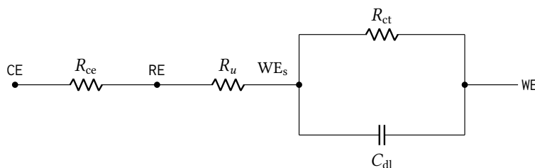
Figure 6: Three-electrode cell model randles_cell, the load the potentiostat actually drives. R_{ce} is the solution resistance from the counter to the reference electrode and R_u the uncompensated resistance from the reference to the working-electrode surface; the interface itself is the charge-transfer resistance R_{ct} in parallel with the double-layer capacitance C_{dl} . Values are given in Table 6. The model is lumped, linear and frequency-independent — no Warburg diffusion term and no potential dependence — so it represents small-signal behaviour about a bias point rather than a full electrochemical response.
