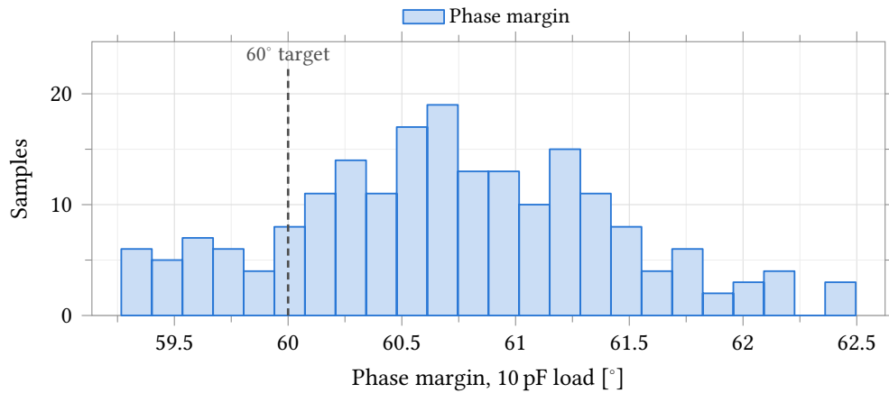
Figure 25: Phase margin driving the 10 pF test load, which is the worst case for this amplifier — a real cell adds resistive loading that lowers the loop gain and raises the margin (Table 16). 29 of 200 samples fall below the 60° target: 85.5 % per channel, 53.4 % across four. The worst is 59.3°, so no sample is near instability; it is the target that is missed.
