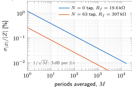
Random term against periods averaged, 11 k \Omega load, 1 kHz
