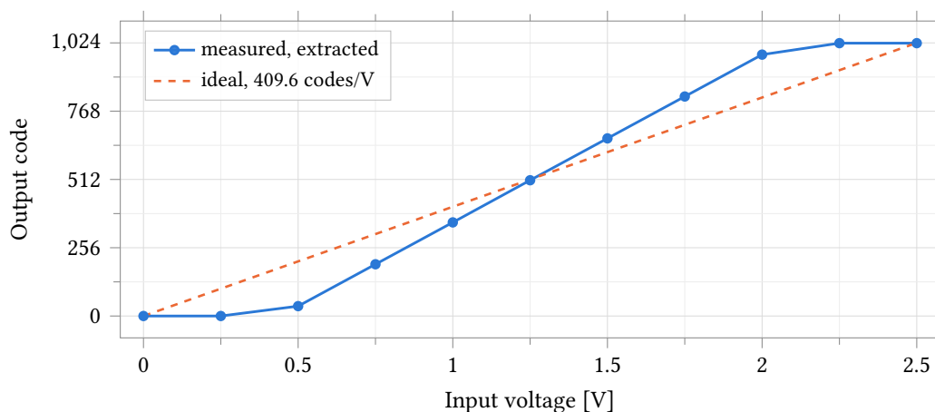
Figure 61: Output code against input voltage for the extracted anatop_pixel_adc, nominal corner, 37 °C, 2.5 V analog and 1.0 V digital supplies, with the ideal 409.6 codes/V line overlaid. The transfer is monotonic and reaches both code limits, but its slope is 628.64 codes/V — 1.535 times ideal — so the flat segments below 0.44 V and above 2.07 V are the code limits, not the ends of the sweep. Markers are the eleven simulated points; the 0.25 V step is 157 codes, so the curve between them is interpolation and carries no linearity information.
