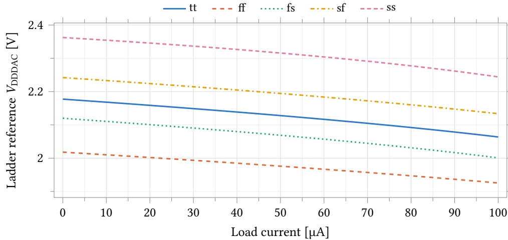
Figure 80: V_{DDAC} against external load current over five process corners, supply block alone, 27 °C at point 1 and 25 °C at points 2–5, ADE default tolerances. There is no feedback loop around the output, so the slope is the block’s own output resistance and the reference falls 92.7 mV to 119.3 mV across the 0 \mu A to 100 \mu A sweep. The curve steepens with load, which is why the chord in Table 86 exceeds the small-signal |Z_{out}| of Table 90. This sweep is an external load only: the ladder is not connected on this bench, and its own code-dependent draw is Figure 74.
