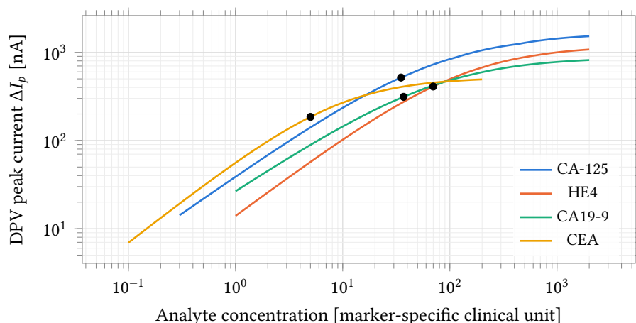
Figure 23: Dose response of the four-reporter panel: published-assay binding curves composed with the current transfer measured from the DPV runs of Figure 22 (11 simulated concentrations per reporter, 560 kΩ tap). Filled circles are the clinical decision points through the same chain: CA-125 35 U/mL → 517 nA, HE4 70 pmol L -1 → 409 nA, CA19-9 37 U/mL → 313 nA, CEA 5 ng mL -1 → 185 nA. The concentration axis carries each marker's own clinical unit; only the current axis is common. The binding model is analytic; the electrode and channel behind the current axis are simulated.
