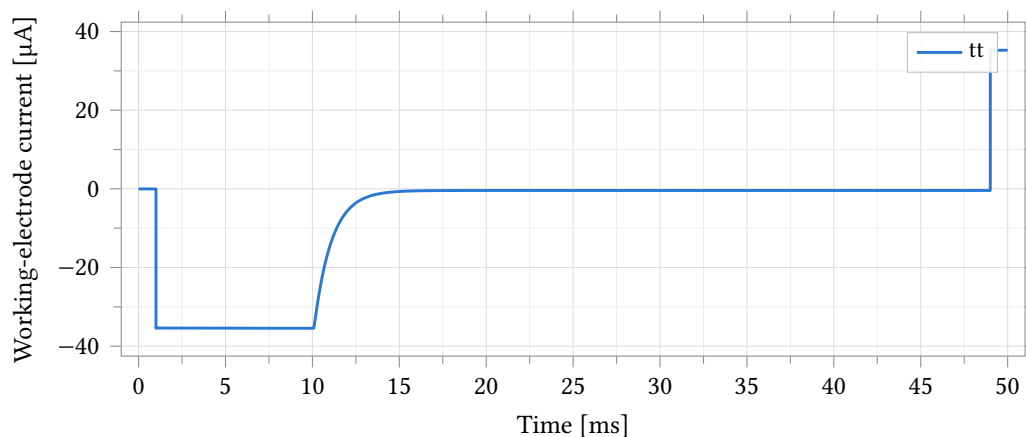
Figure 54: Step response of the working-electrode current to a 400 mV step in the commanded reference potential, typical process point, 37 °C, R_f = 35 \text{ k}\Omega , R_{ct} = 1 \text{ M}\Omega electrode, 1 \mu\text{s} edge. The transient overshoots and briefly rails against the loop's slew-limited edges immediately after the step – by design, the bench exercises the edge rather than a settled operating condition – before settling to the value set by the cell impedance.
