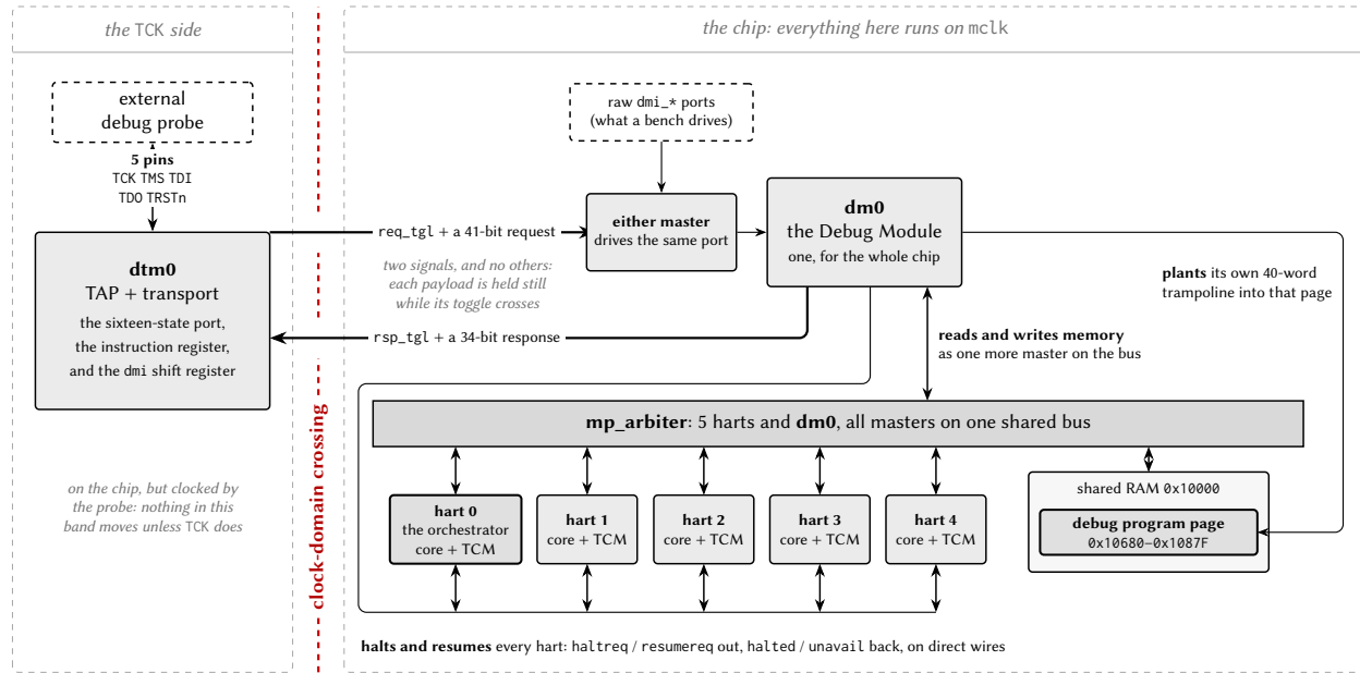
Figure 11: Block diagram of the debug path, from the probe to the harts.
