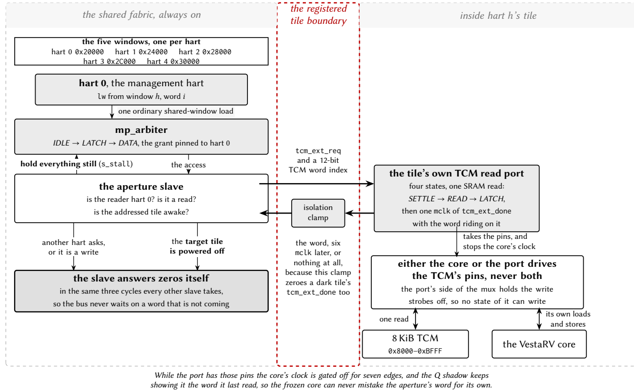
Figure 4: Block diagram of one read through a TCM aperture.
