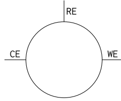
Figure 18: Three-electrode cell model, the load the potentiostat actually drives, shown as the symbol used throughout this chapter. It is a lumped linear network between the counter, reference and working electrodes; its elements and their values are given in Table 12. The model is frequency-independent (no Warburg diffusion term and no potential dependence), so it represents small-signal behaviour about a bias point rather than a full electrochemical response.
