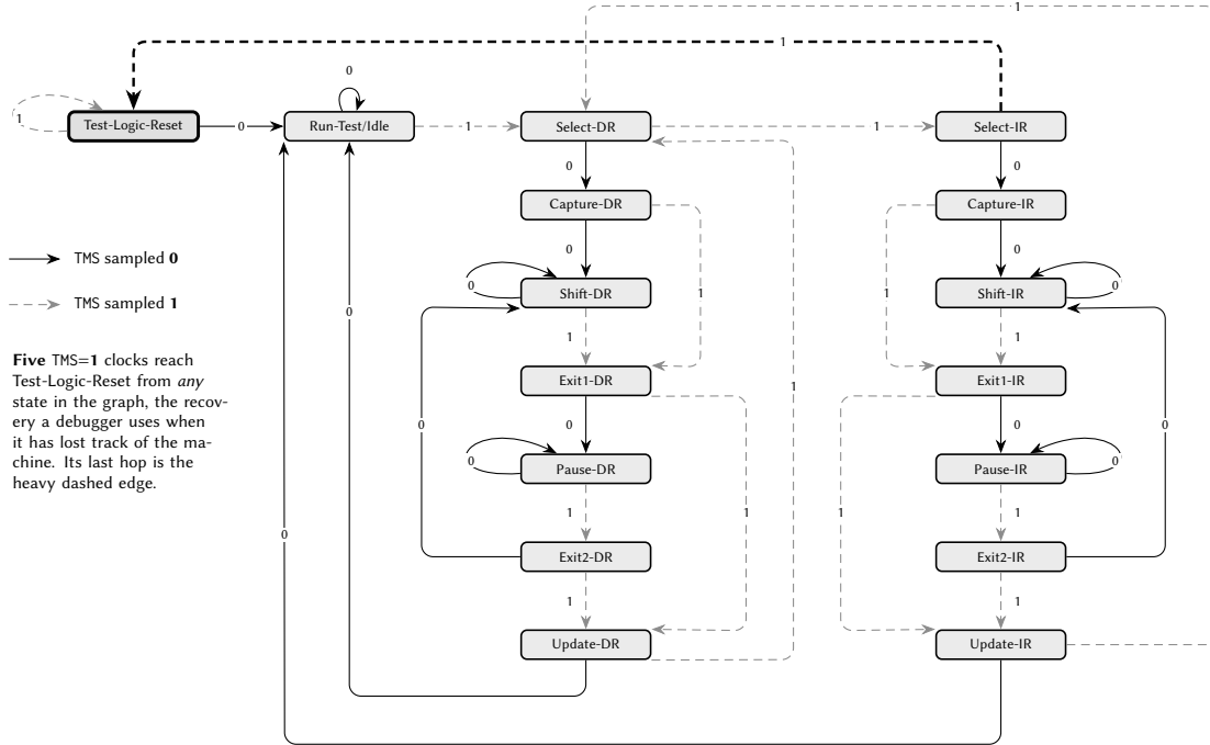
Figure 9: State diagram of the sixteen-state JTAG test access port.
