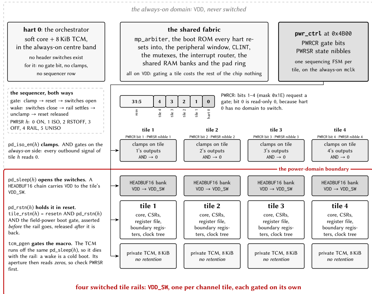
Figure 100: The chip's power domains and what a gate bit does.
