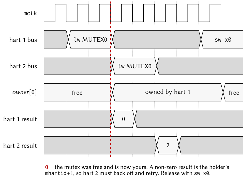
Figure 102: Two harts racing for the same mutex.
