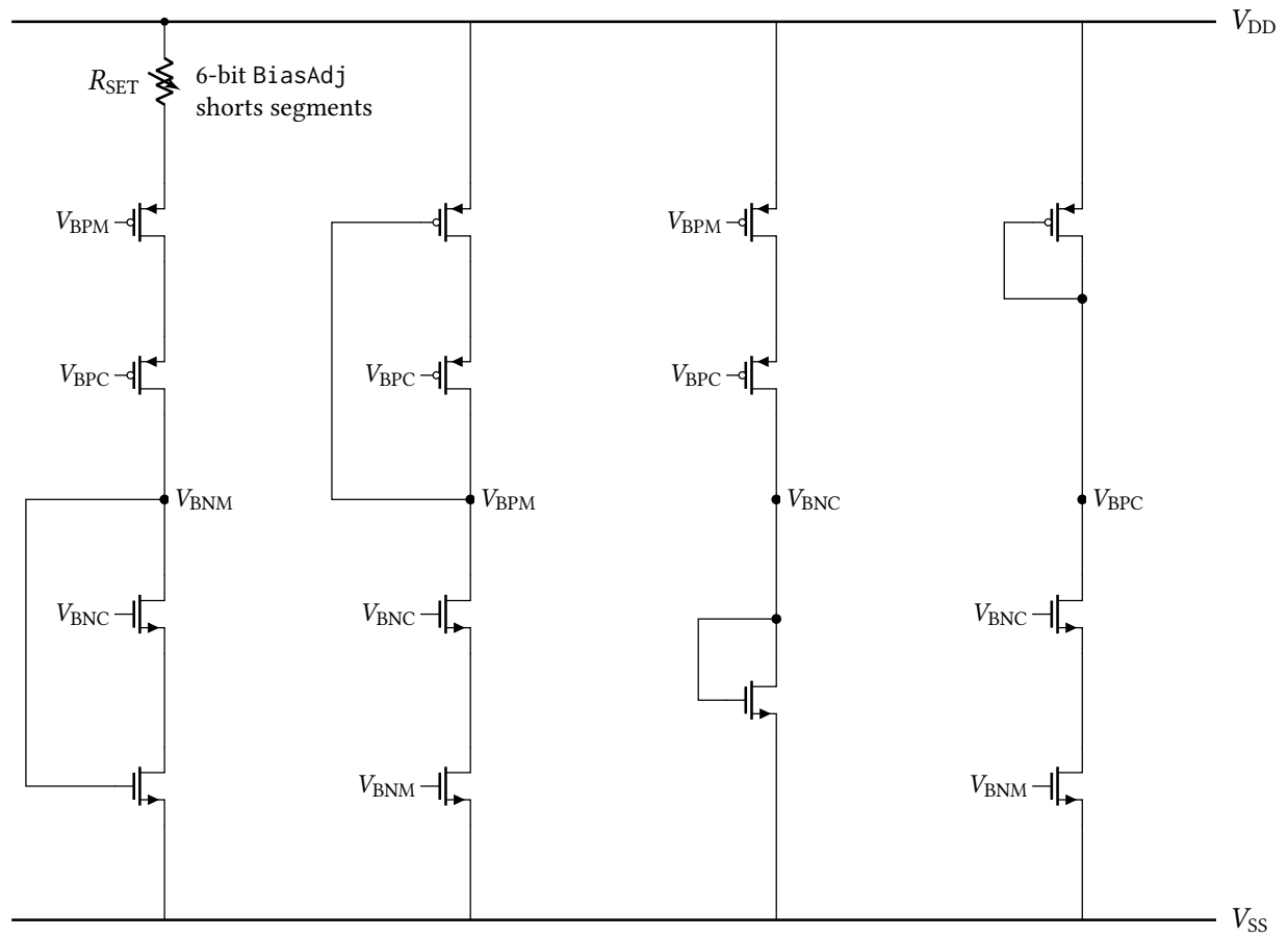
Figure 24: Simplified core of the local wide-swing cascode bias generator, drawn from the anatop_biasgen_local schematic. Four self-biased branches develop the four rails: the reference branch (left) passes the current set by the trimmable resistor R_{SET} , and the remaining branches mirror it to produce V_{BPM} , V_{BNC} and V_{BPC} . Each branch's own self-bias (diode) connection is drawn, from the rail it generates back to the gate it drives in the same branch; the cross-branch gate connections are identified by net name rather than drawn as buses. The enable switches, the decoupling capacitors on each rail and the individual segments of the resistor string are omitted for clarity.
