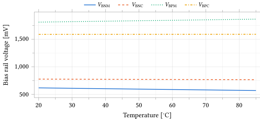
Figure 26: The four local bias rails against temperature at the typical corner. V_{\text{BNM}} and V_{\text{BNC}} are referred to vss!; V_{\text{BPM}} and V_{\text{BPC}} sit near the supply.
