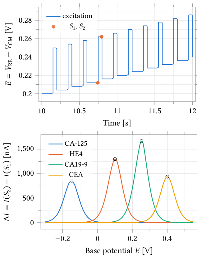
Figure 22: Differential-pulse voltammetry through the rev-2 channel, four-reporter immunoassay panel, one electrode parameter set per reporter ( R_f = 560 \text{ k}\Omega , C_{dl} = 200 \text{ nF} , 37^\circ\text{C} ). Top: a 2 s excerpt of the excitation — 4 mV treads, 50 mV / 50 ms pulses at a 200 ms period, every level quantised to the 14-bit DAC LSB — with the two current-sampling instants 5 ms before each edge. Bottom: the differential current over the full -0.300 \text{ V} to 0.548 \text{ V} scan (213 steps, 42.6 s); peak potential separates the reporters, peak height carries concentration (circles mark the apexes: 855 nA, 1300 nA, 1666 nA and 938 nA). Reporter kinetics as in the cyclic-voltammetry runs; the panel differs from Figure 21 in readout, gain tap and reporter set.
