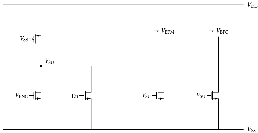
Figure 25: Start-up branch. A gate-grounded, permanently-on weak PMOS pulls V_{SU} up at power-on; while V_{SU} is high it drags V_{BPM} and V_{BPC} down, forcing current into the core and breaking the degenerate zero-current state. Once the core is running, the rising V_{BNC} turns on the left NMOS and collapses V_{SU} , so the branch draws no static current in normal operation, the behaviour visible in the power-up transient of Figure 33. A second device holds V_{SU} low whenever the cell is disabled.
