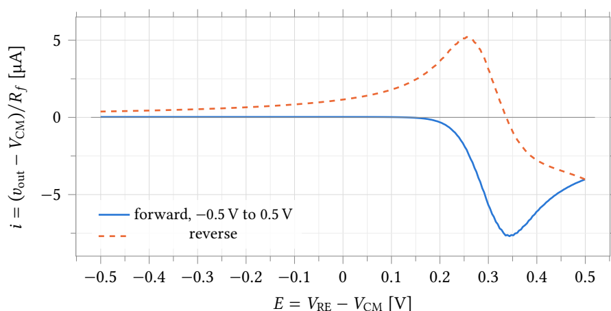
Figure 57: Staircase cyclic voltammogram taken through the complete assembled channel – real 12-bit potential codes, real programmable feedback resistor at N = 3 (37.16 k \Omega measured in the loop) – of the electrode of Section 8.2 at 2 \text{ V s}^{-1} , 37 °C, nominal process point. One point per 4 mV tread, sampled 50 \mu\text{s} before the next code change, so the double-layer charging current has decayed and what remains is faradaic; the sign convention is the measured one of Section 8.5, dv_{\text{out}}/di_{\text{we}} = +R_f , so oxidation reads negative. Peak potentials sit within 0.3 mV and 2.3 mV of the same electrode driven by an ideal source; sampled peak heights are 11.2 % and 13.9 % lower, which is the staircase sampling and not a channel error (Table 67).
