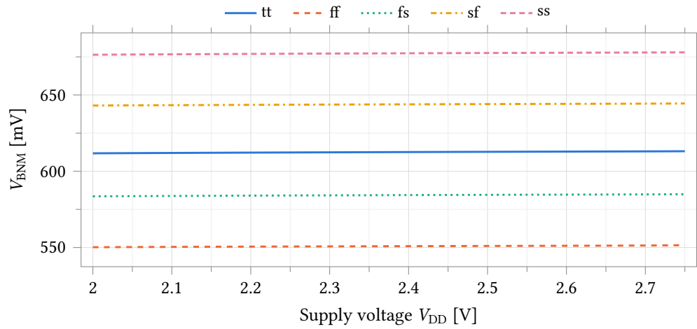
Figure 29: Supply rejection of the NMOS mirror bias: V_{\text{BNM}} against V_{\text{DD}} over all process corners.
