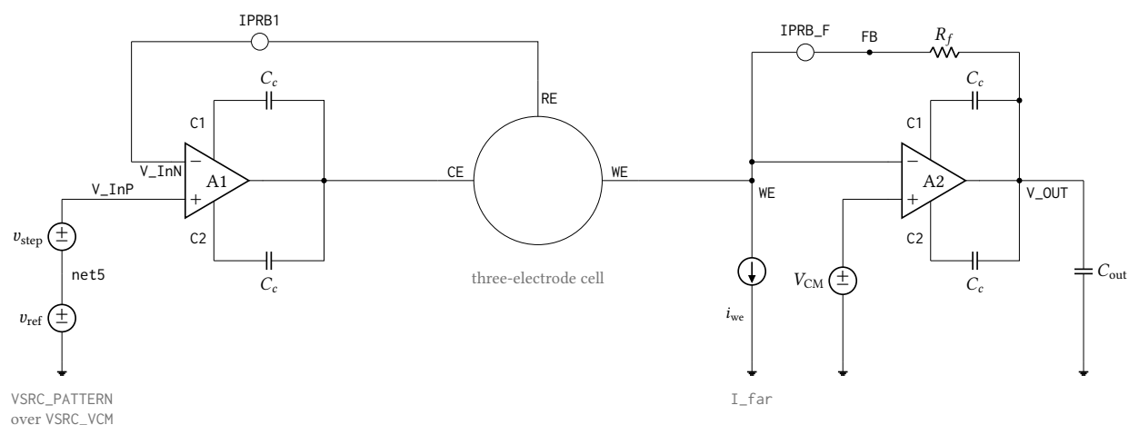
Figure 48: The complete rev-2 potentiostat pixel as simulated, tb_anatop_pixel view PotFbTB: control amplifier A1 drives the counter electrode and closes its loop on the reference electrode, while transimpedance amplifier A2 holds the working electrode at V_{CM} and returns the cell current through R_f to V_{OUT} . Both amplifiers are the same anatop_tia_amp_ab class-AB cell, each with its own external compensation capacitors C_c = 500 fF from pins C1/C2 onto its own output; supplies, En and the shared local bias generator are omitted. IPRB1 and IPRB_F are 0 V current probes inserted only so that stb can break the control loop and the transimpedance loop respectively – they add no impedance and no offset. I_{far} injects the accuracy-truth current with positive i_{we} flowing from the working electrode to ground, so v_{out} = V_{CM} + i_{we} \cdot R_f and the measured current is the probe current in IPRB_F; the opposite source orientation inverts the sign of every accuracy number. Cell elements are R_{ce} = R_u = 1 k \Omega fixed with R_{ct} and C_{dl} swept over the electrode grid, R_f is the programmable feedback resistor (35 k \Omega to 560 k \Omega ), and C_{out} = 5 pF.
