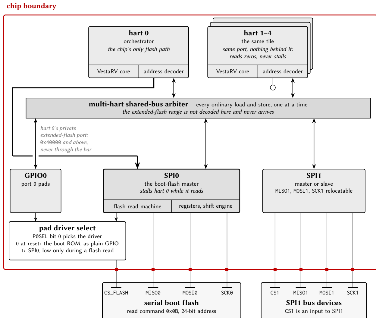
Figure 88: SPI connection diagram: SPI0 and the boot flash.
