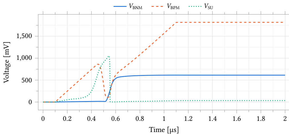
Figure 33: Power-up transient at the typical corner. The start-up node V_{SU} pulls the core out of its zero-current state, after which both mirror rails settle to their steady-state values.
