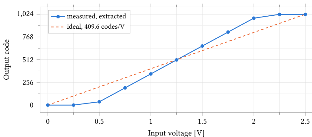
Figure 63: Output code against input voltage for the extracted anatop_pixel_adc, nominal corner, 37 °C, 2.5 V analog and 1.0 V digital supplies, with the ideal 409.6 codes/V line overlaid. The transfer is monotonic and reaches both code limits, but its slope is 628.64 codes/V — 1.535 times ideal — so the flat segments below 0.44 V and above 2.07 V are the code limits, not the ends of the sweep. Markers are the eleven simulated points; the 0.25 V step is 157 codes, so the curve between them is interpolation and carries no linearity information.
