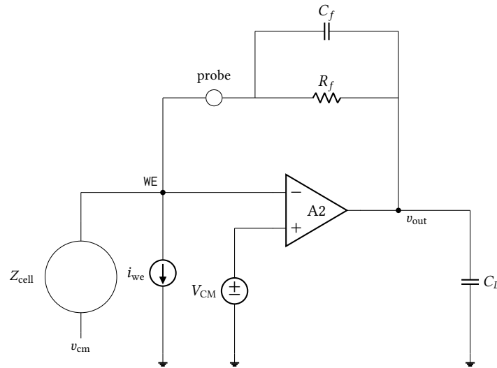
Figure 39: The closed transimpedance loop bench, the only one in this section that closes feedback around the electrode. R_f \parallel C_f returns the output to the working electrode through a current probe, i_{we} is the test source, and Z_{cell} is the Randles cell of Figure 18, returned to v_{cm} . The loop gain, phase margin and crossover are measured through the probe; the DC accuracy, closed-loop transfer and noise figures come from the same wiring.
