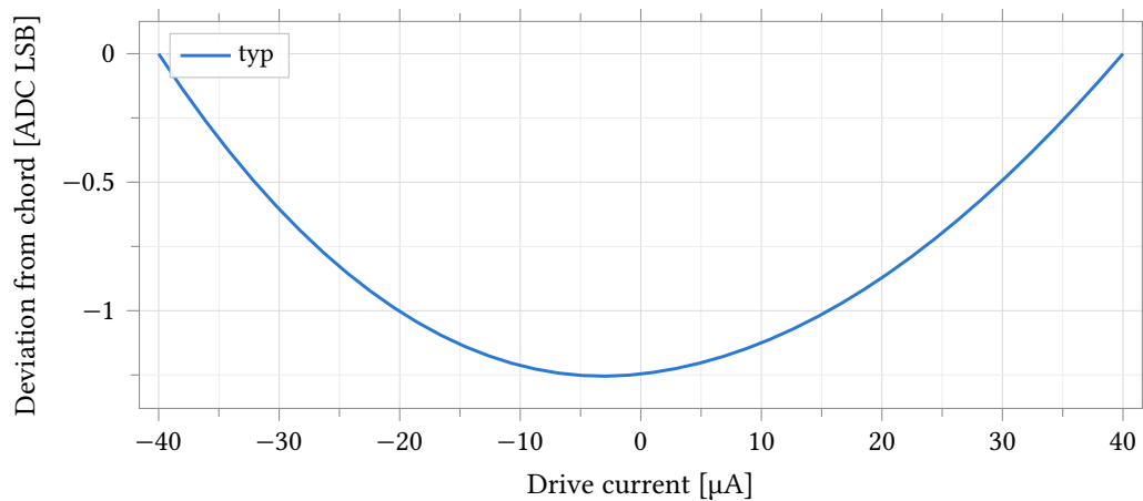
Figure 70: Drive nonlinearity of the bottom code ( N = 0 , R \approx 19.6 k \Omega ): voltage deviation from the endpoint chord over \pm 90 % of full scale ( \pm 40 \mu A), typical corner, expressed in 1.592 mV ADC LSB. All ten bypass gates are closed at this code and carry the full signal current; their on-resistance rises with the terminal's excursion from V_{CM} , so the chord — pinned at the sweep endpoints where that excursion is largest — overestimates the mid-range voltage by up to 1.25 LSB, and the deviation is bowl-shaped with a slight skew from the gates' voltage asymmetry. The same measurement at N = 63 and N = 319 , where the ladder dominates and current is 20–100 \times smaller, stays below 0.004 LSB and is tabulated, not plotted.
