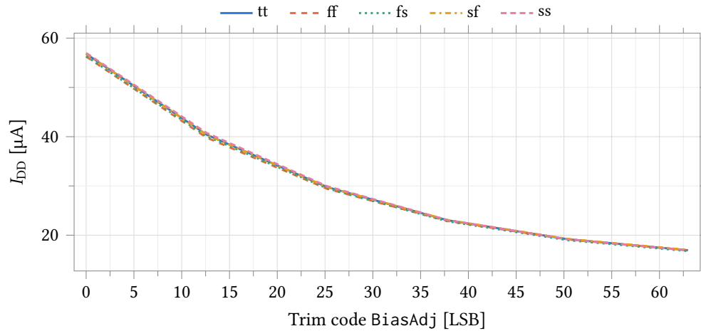
Figure 32: Trim characteristic: quiescent supply current against the BiasAdj word over all process corners, at the same six sampled codes. The current is strongly monotonic in the trim word, falling by a factor of about 3.4 from code 0 to code 63.
