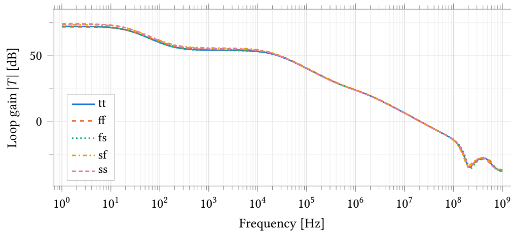
Figure 51: Potentiostat control-loop gain over five process corners, measured through the 0 V probe IPRB1 in the RE feedback path (Figure 48). R_f = 35 \text{ k}\Omega , cell R_{ce} = R_u = 1 \text{ k}\Omega , R_{ct} = 10 \text{ k}\Omega , C_{dl} = 100 \text{ nF} , 2.5 V supply. This is the full loop – A1, A2, both feedback networks and the electrode together – and is not the open-loop amplifier gain of Section 8.4. tt is at 37^\circ\text{C} , the four skew corners at 25^\circ\text{C} .
