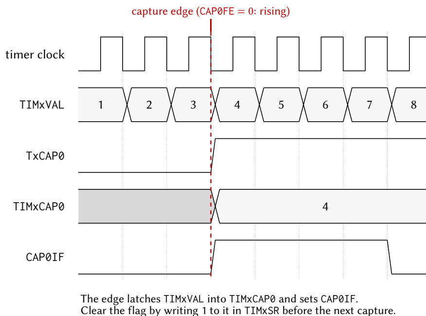
Figure 97: Input capture: an edge on TxCAP0 latches TIMxVAL into TIMxCAP0.
