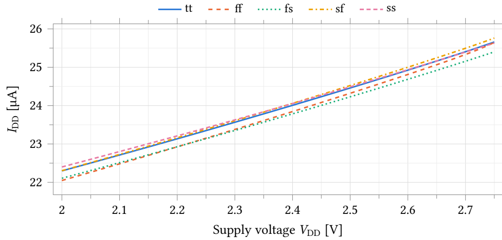
Figure 30: Quiescent supply current against supply voltage over all process corners.
