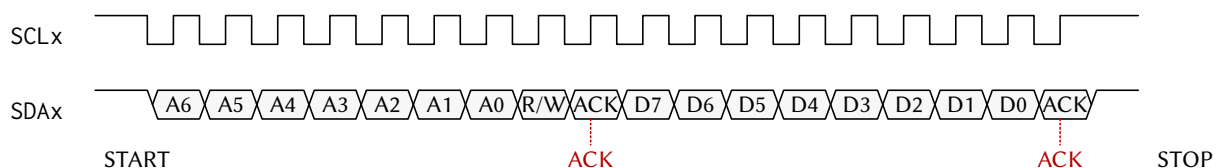
Figure 101: One I2C byte write on the wire: START, address, ACK, data byte, ACK, STOP.
