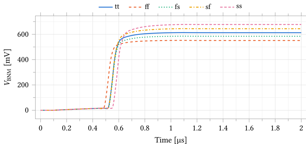
Figure 34: Power-up settling of V_{BNM} over all process corners.
