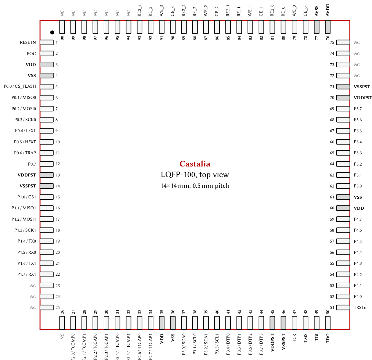
Figure 2: LQFP-100 pinout, top view (14 × 14 mm, 0.5 mm pitch). GPIO pins carry their AF0 function; power-rail pins are shaded.
