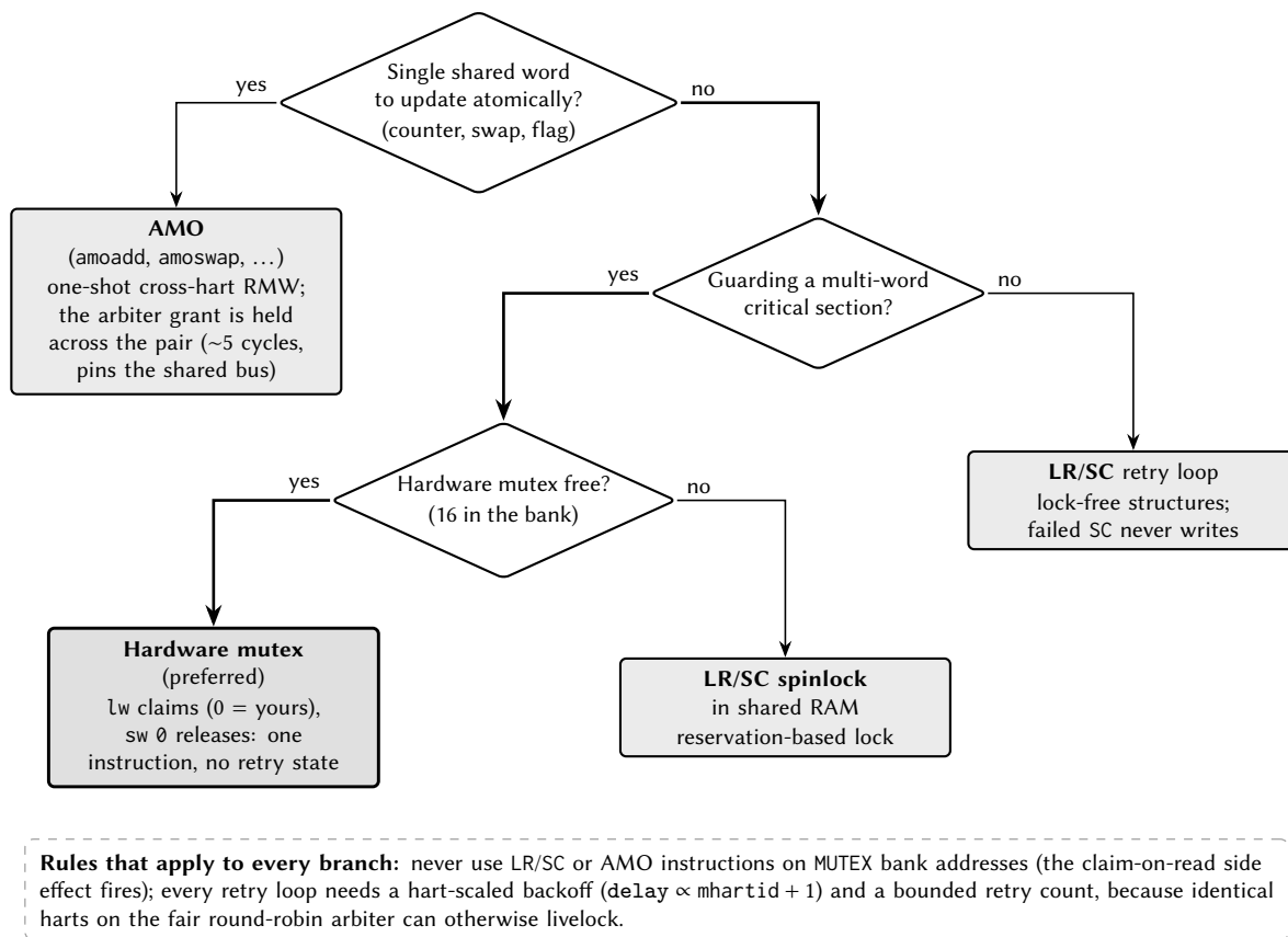
Figure 8: Decision chart for choosing a synchronization primitive.
