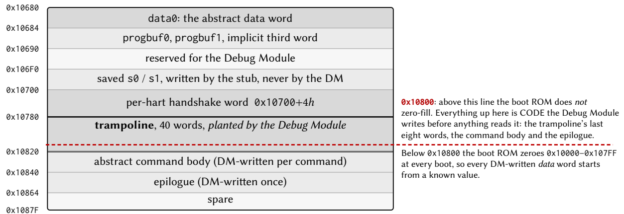
Figure 15: Memory map of the debug program page in shared memory.
