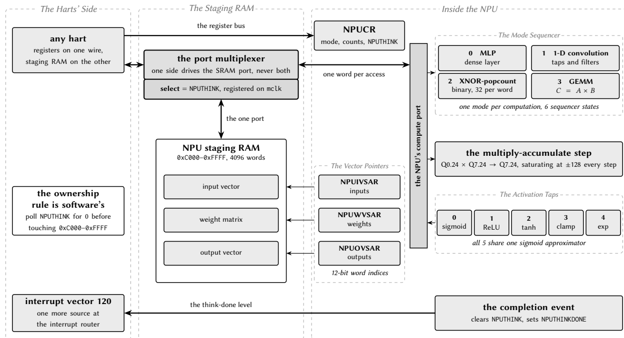
Figure 99: The NPU datapath and the staging RAM it borrows.
