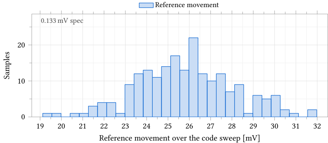
Figure 81: Peak-to-peak movement of the DAC reference V_{dd}DAC across the 4096-code sweep, with the ladder referenced to the on-chip supply block instead of an ideal rail. Process and mismatch , castalia_pm_25 , 200 samples, 25 °C, no external load on V_{dd}DAC . The quarter-LSB budget of 133 \mu V entered on the test sits about 200 times below the data, so it is annotated at the left axis edge rather than drawn and the distribution is not compressed into a single bar; the closest sample misses it by a factor of 144. Meeting it needs the supply's output impedance down by a factor of 193, to about 5 \Omega , against 894 \Omega small-signal (Table 95) and 1133 \Omega as a 0 \mu A to 100 \mu A chord (Table 91).
