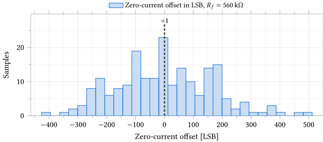
Figure 56: Zero-current output offset at R_f = 560 \text{ k}\Omega , conditions as Figure 55 but at R_{ct} = 10 \text{ k}\Omega (the same stiff electrode as the finite-loop-gain demonstration of Table 55, NOT the 1 \text{ M}\Omega operational electrode of Table 54). Some samples reach the sweep’s output rails (Table 64); the LSB spread here is 14\times wider than at 35 \text{ k}\Omega for the same underlying current offset, since the same offset current is multiplied through a 16\times larger R_f .
