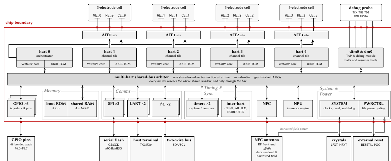
Figure 1: Castalia whole-chip diagram: the masters above one mp_arbiter bus bar, every peripheral on one rank below it, and the package boundary in red.
