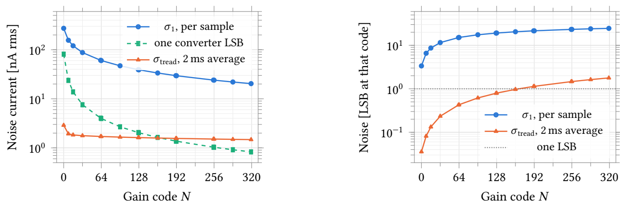
Figure 58: Input-referred current noise of the assembled channel against gain code, at the nominal electrode ( C_{\text{dl}} = 100 \text{ nF} , R_{\text{ct}} = 1 \text{ M}\Omega ), nominal process point, 37^\circ\text{C} , integrated from 0.1 Hz to 10 MHz and referred by the measured in-loop transimpedance. \sigma_1 is one converter sample; \sigma_{\text{tread}} is the average of the 1738 samples taken inside one 2 ms staircase tread, by the exact Dirichlet integral of the same spectrum — not \sigma_1/\sqrt{N} , which the transient-noise measurement of Section 8.6.7 finds wrong by up to 6.7 \times . Left, in current: the averaged floor is 1.5 nA to 2.9 nA and barely moves with gain, while one LSB falls 98 \times , so the two cross at N \approx 165 and every code above it is noise- rather than quantisation-limited. Right, the same referred to the LSB at each code; a single sample is never better than 3.4 LSB, which is why the readout average is part of the specification and not an option. The feedback capacitor does not appear here: it divides output noise and transimpedance by the same factor and leaves the input-referred quantity unchanged to four digits.
