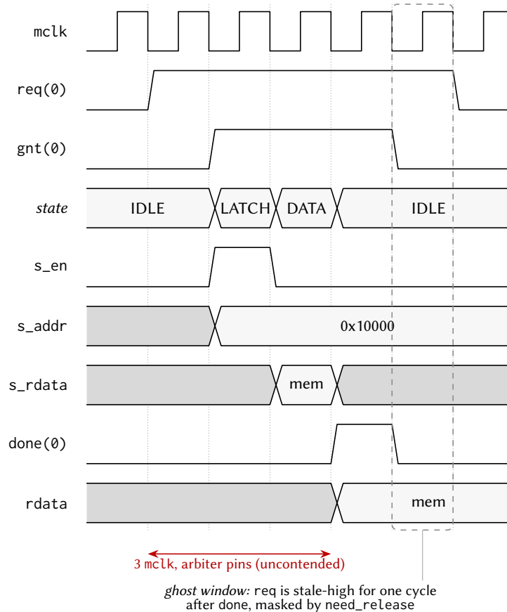
Figure 5: Timing diagram of one uncontended shared-window read at the mp_arbiter pins.
