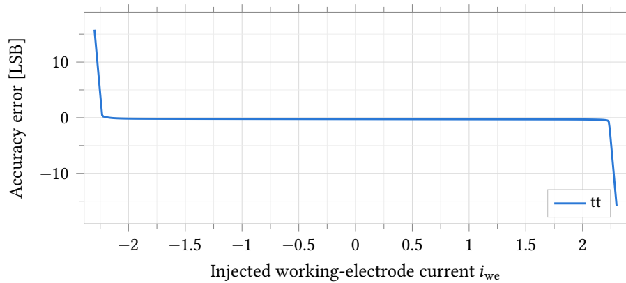
Figure 50: Accuracy error at the operational max-gain point, R_f = 560 \text{ k}\Omega into R_{ct} = 1 \text{ M}\Omega , typical process point, 37^\circ\text{C} . The truth current sweep is \pm 2.3 \mu\text{A} , just beyond the 2.06 \mu\text{A} full-scale current at this gain tap; the crossing at zero is smooth, with no kink, over the full swept range shown.
