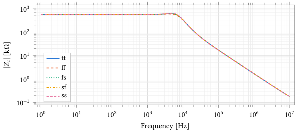
Figure 40: Closed-loop transimpedance magnitude over five process corners, conditions as Figure 41. The AC stimulus is a 1 A current into the working electrode, so the ordinate is transimpedance directly. The feedback resistor is an ideal element here rather than the 16-tap string, which is why the corners separate only near the band edge; the numbers are in Table 37.
