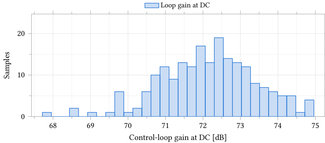
Figure 47: DC gain of the control loop closed around an electrochemical cell. Process and mismatch , 37 °C, 200 samples, cell-drive bench (Figure 45) with a Randles cell of R_{CE} = 1 k \Omega , R_u = 1 k \Omega , R_{ct} = 10 k \Omega , C_{dl} = 1 \mu F, working electrode at 1.25 V, C_L = 5 pF, C_c = 500 fF, 2.5 V supply. The loop is measured through the reference-electrode sense wire and therefore includes the cell, whose 12 k \Omega loads an open-loop output resistance of about 25 k \Omega and is 10 dB below the unity-feedback gain of Table 31. The spread is 7 dB peak to peak and no sample falls below 67 dB. No limit was entered on this output.
