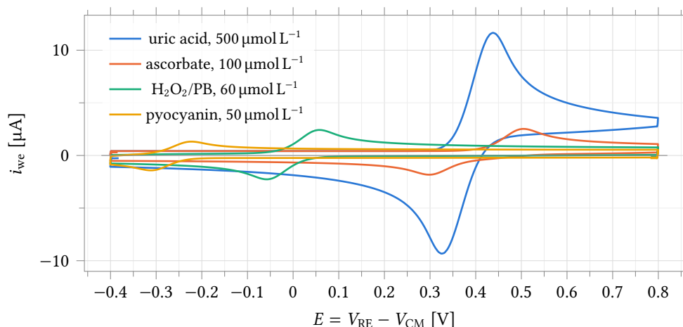
Figure 21: Voltammograms of the four-analyte wound panel through the rev-2 channel, one electrode parameter set per channel, from the cyclic-voltammetry Maestro corner run of Section 8.2 (2 V s -1 , R_f = 35 kΩ, conditions of the in-loop run above). Peak potential identifies the analyte and peak height its concentration; each trace is one full cycle started at that analyte’s non-faradaic vertex. E^{0'} and concentrations are literature-anchored; k^0 is fitted (no measured value exists on carbon for any of the four), and reversal peaks appear for the chemically irreversible couples because following chemistry is not modelled. The two cathodic markers span -1.4 μA to -2.4 μA — unmeasurable by the unidirectional rev-1 front end.
