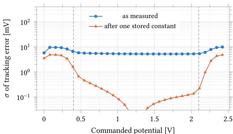
Figure 59: Spread of V_{RE} - V_{PATTERN} against the commanded potential on the assembled channel, 200 samples, process and mismatch, nominal process point, 37 °C: as measured, and after the same sample’s mid-code value is subtracted — the residual one stored per-channel constant leaves behind. That residual is zero at mid-code by construction and falls off the bottom of the axis there. Dashed lines mark the specified 0.4 V to 2.1 V window; interior to it the error is a pure constant to 0.36 mV, while outside it A1’s input pair is leaving its common-mode range and no constant reaches the remainder.
