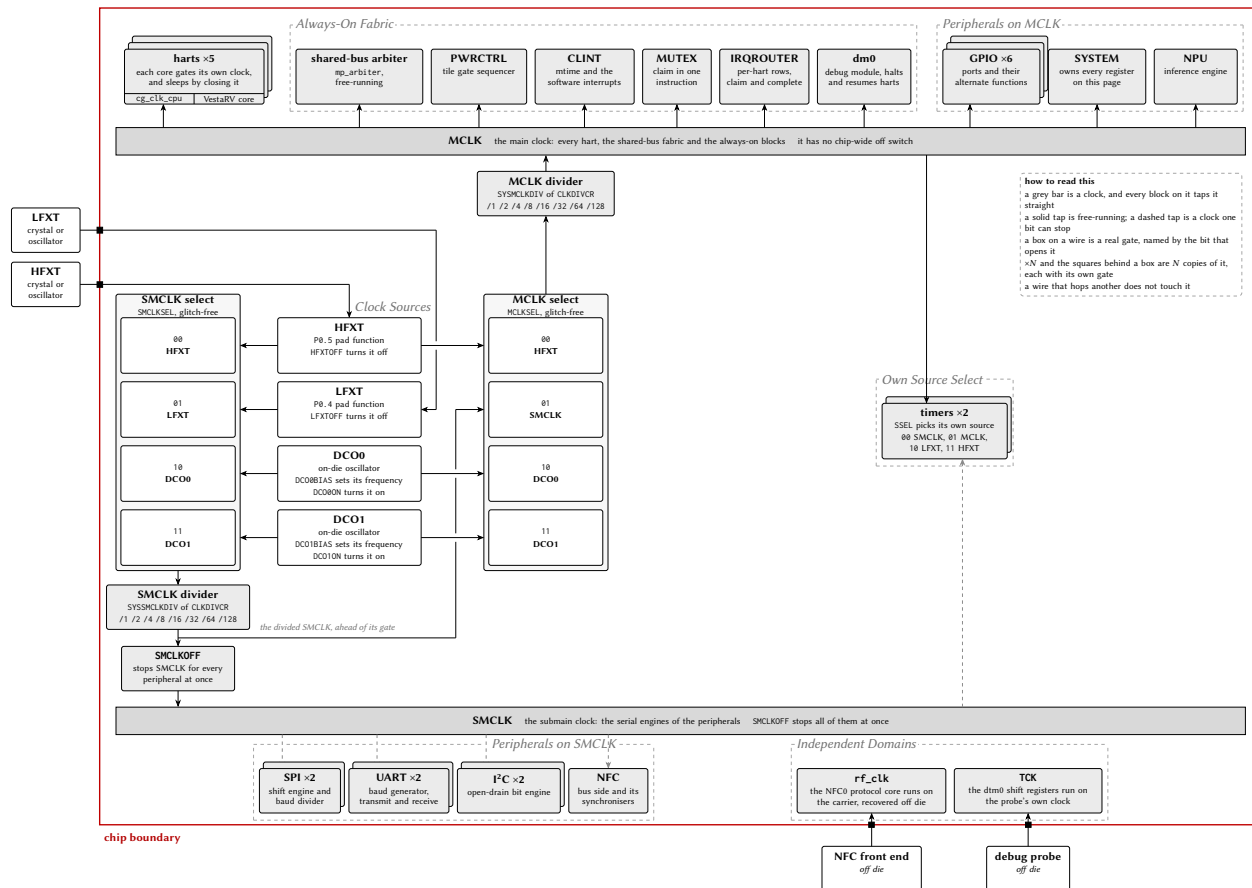
Figure 98: The MCU clock system: sources, the MCLK and SMCLK bars, and the blocks they clock.
