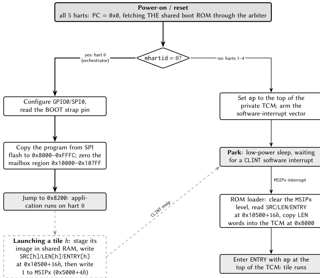
Figure 7: Flow chart of boot and tile loading across the harts.
