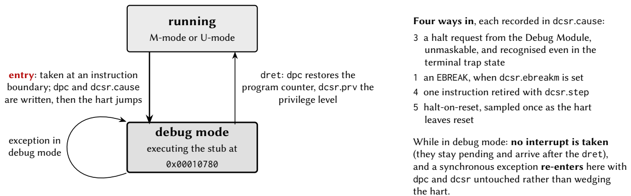
Figure 14: State diagram of debug mode, from the hart’s point of view.
