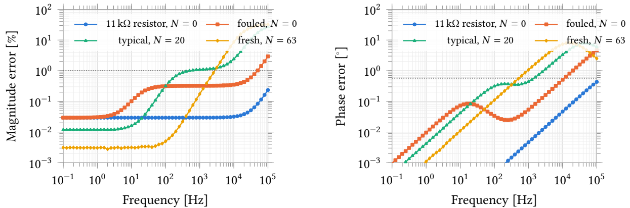
Figure 60: Measured impedance error against frequency — magnitude (left) and phase (right) — for the calibration resistor and the three electrode cases, each at the gain code that ranges it, with the applied potential read at the reference electrode and the current measured. Error is taken against the analytic impedance of the load, so these are the chain’s errors and not the model’s; dotted lines are the 1% and 0.573° gates. Each curve turns up where the electrode’s impedance has collapsed toward R_u = 1\text{ k}\Omega and the noise gain 1 + R_f/|Z| has therefore risen, which is why the highest-gain case is the most accurate below 100 Hz and the first to degrade above 1 kHz. The gate crossings here are not the bandwidth specification: the ratio R_f/|Z| moves with frequency on a real electrode, and the specification comes from the fixed-ratio measurement of Section 8.7.2.
