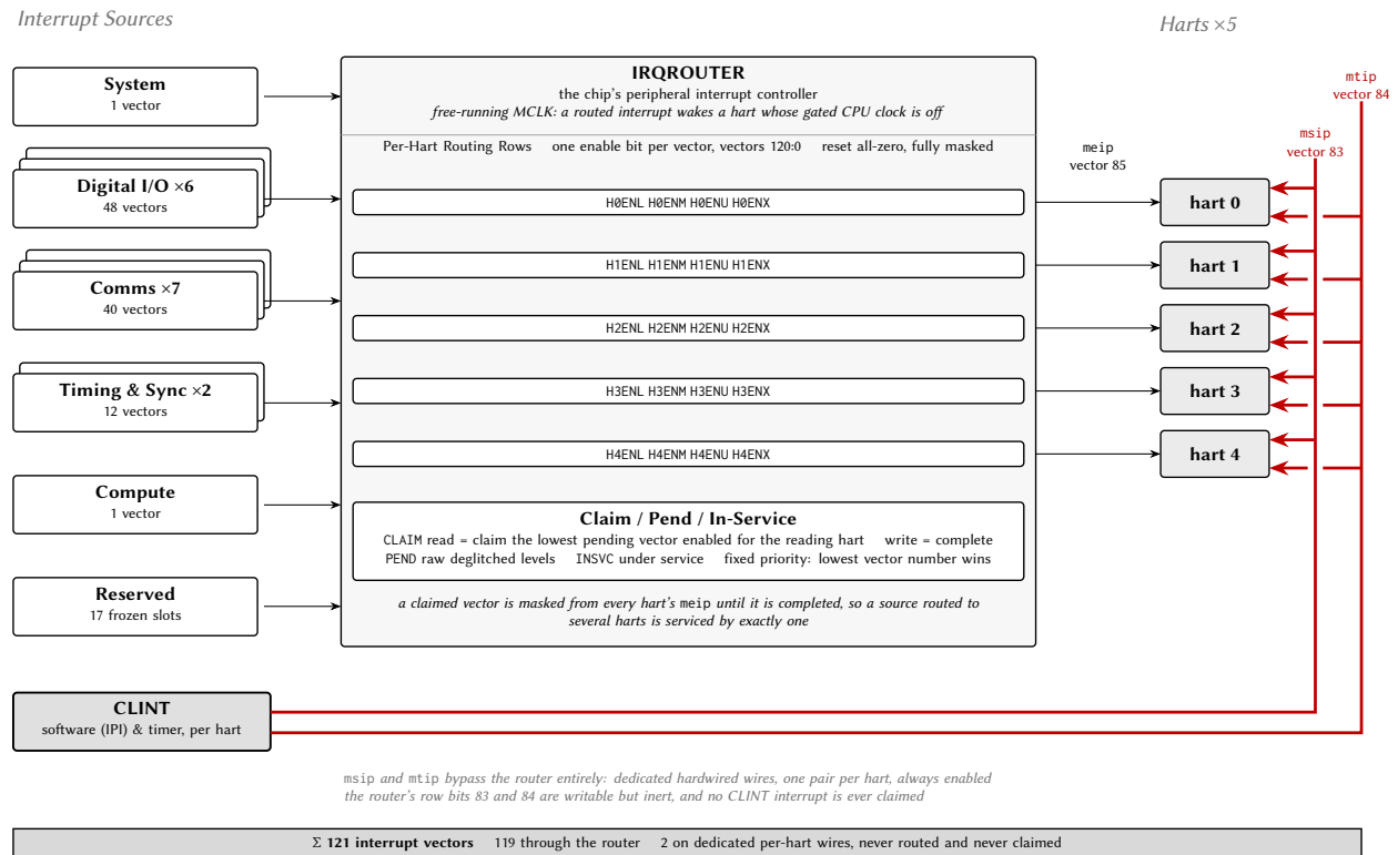
Figure 87: Castalia interrupt fabric: the source types, the IRQROUTER's per-hart rows, and the CLINT rails that bypass it.
