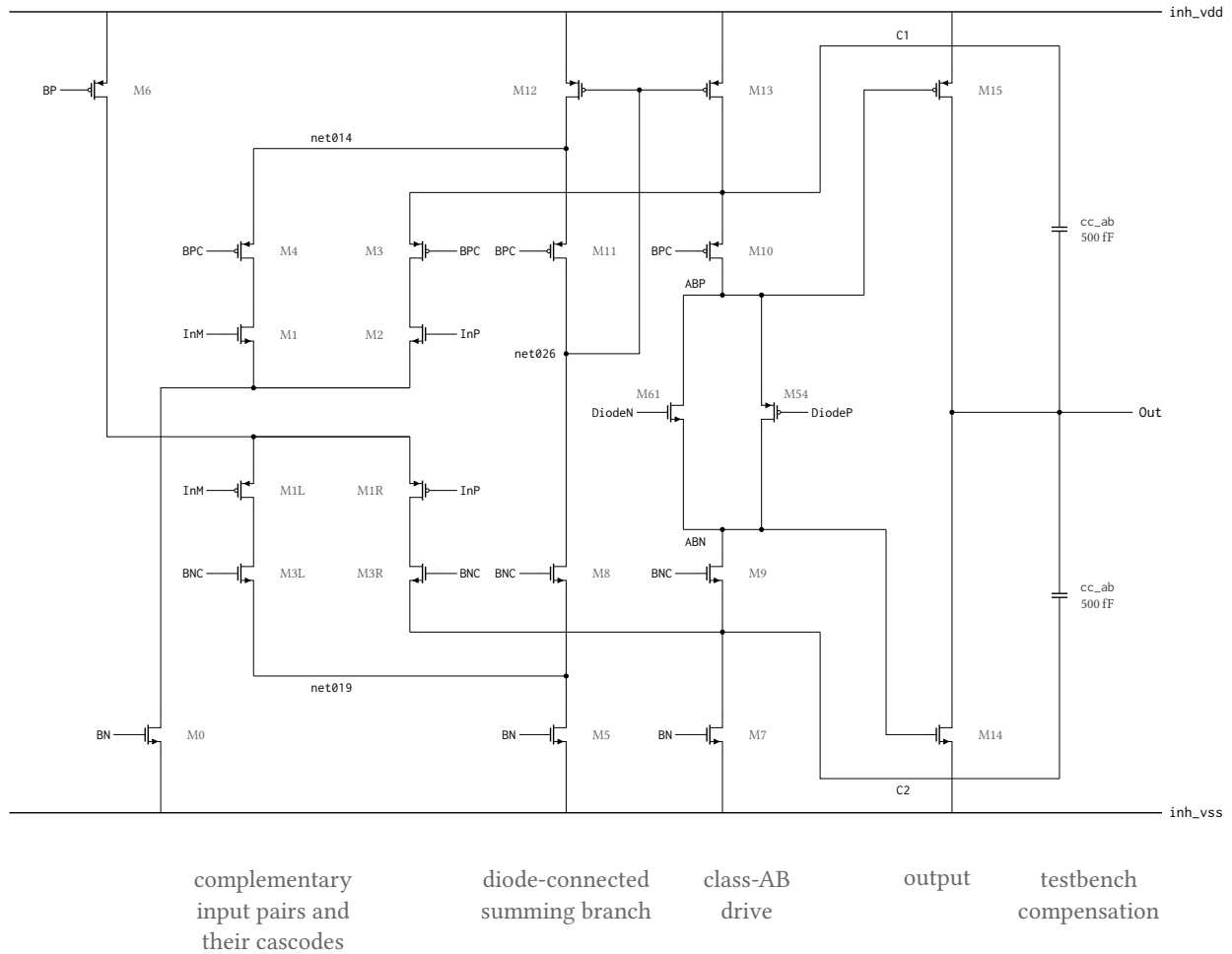
Figure 35: Signal-path topology of the class-AB amplifier anatop_tia_amp_ab , drawn from its netlist. The complementary pairs M1/M2 (NMOS, tail M0) and M1L/M1R (PMOS, tail M6) fold into two cascode branches; the InM side terminates in the diode-connected branch M12–M11–M8–M5, whose summing node net026 sets M13, which restates that current into the InP branch, and the floating pair M54/M61 holds ABP above ABN so both output devices M15 and M14 are actively driven. C1 and C2 are the common source nodes of the PMOS cascodes M10/M3 and of the NMOS cascodes M9/M3R, brought out as pins; the two cc_ab capacitors that return them to Out are testbench components outside the cell, 500 fF per side. Simplified: the enable switch and its four power-down devices, and the bias generator that develops DiodeN/DiodeP, are omitted, so 22 of the cell’s 34 transistors are drawn; BP/BPC/BN/BNC are the enabled forms of the bp!/bpc!/bn!/bnc! globals and device dimensions are not shown. Identically labelled nets are connected; wires crossing without a filled dot are not.
