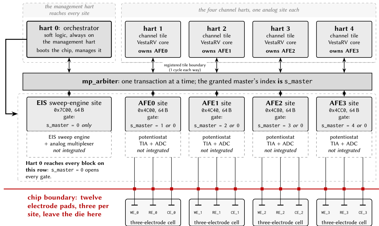
Figure 17: Analog front-end connectivity: each channel hart owns one measurement site, hart 0 opens every gate, and the dashed analog stages are not yet integrated.
