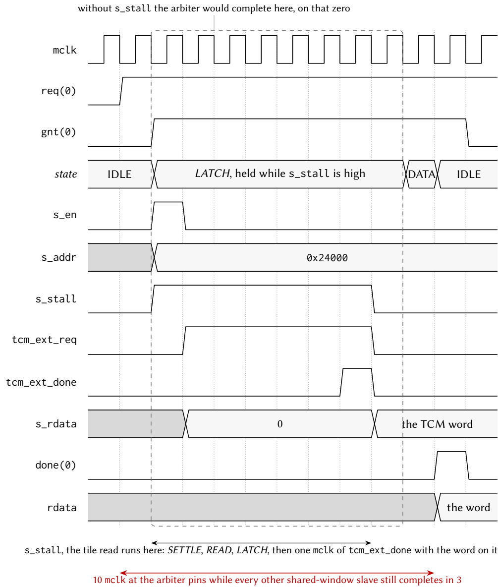
Figure 6: Timing diagram of one stalled shared-window read through a TCM aperture.
