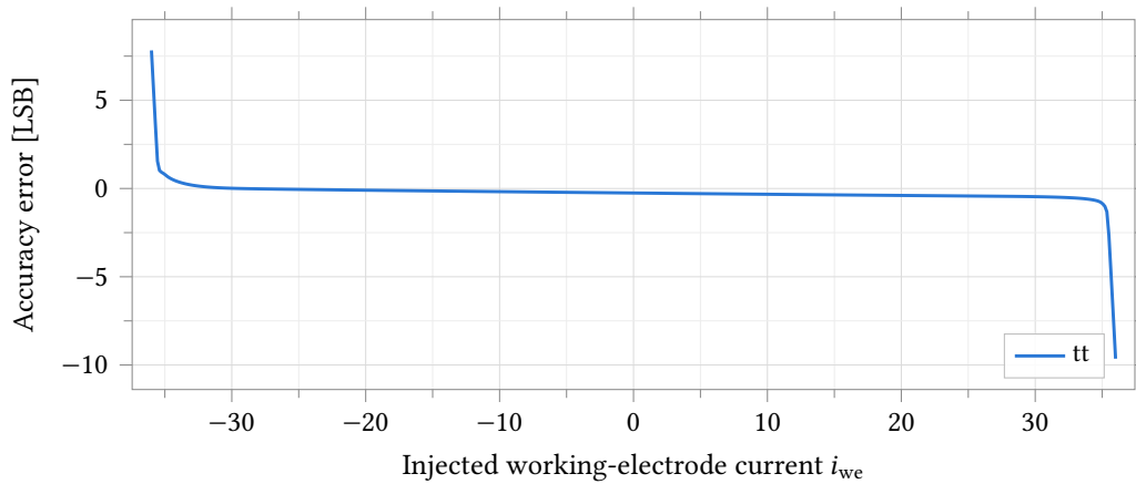
Figure 49: Bipolar accuracy error against injected working-electrode current, R_f = 35\text{ k}\Omega , R_{ct} = 10\text{ k}\Omega electrode, typical process point, 37^\circ\text{C} , full \pm 36\text{ }\mu\text{A} sweep (full scale \pm 33\text{ }\mu\text{A} ). The zero crossing is smooth with no kink or discontinuity between the sourcing and sinking halves of the sweep: the error’s slope through zero is -1/T exactly (Table 53) and the same single anatop_tia_amp_ab TIA feedback path serves both current directions, unlike the rev-1 PMOS-only mirror it replaces.
