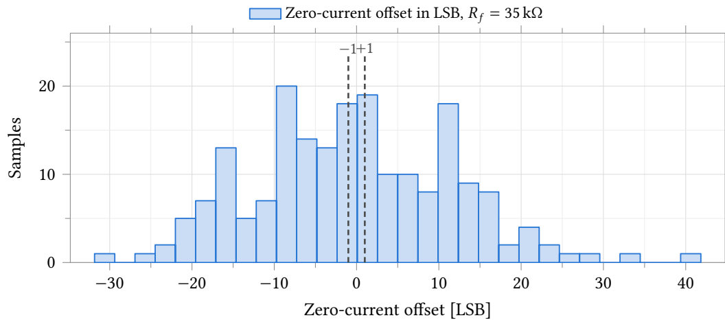
Figure 55: Zero-current output offset at R_f = 35 k \Omega , referred to the 2.441 mV ADC LSB. Mismatch only , 25 °C nominal process, 200 samples, R_{\text{ct}} = 10 k \Omega electrode. The limit shown is the \pm 1 LSB entered on the test in Assembler – comparable in kind across the four gain taps but mechanically harder to meet as R_f rises, since the underlying offset is closer to gain-independent in current (Table 64). Statistics are in Table 64.
