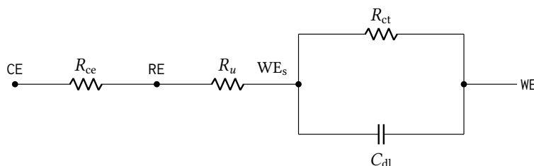
Figure 19: Three-electrode cell model, the load the potentiostat actually drives. R_{ce} is the solution resistance from the counter to the reference electrode and R_u the uncompensated resistance from the reference to the working-electrode surface; the interface itself is the charge-transfer resistance R_{ct} in parallel with the double-layer capacitance C_{dl} . Values are given in Table 12. The model is lumped, linear and frequency-independent (no Warburg diffusion term and no potential dependence), so it represents small-signal behaviour about a bias point rather than a full electrochemical response.
