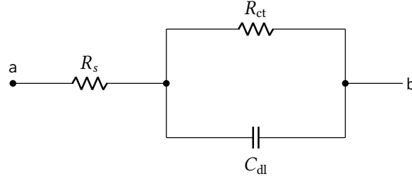
Figure 20: Single electrode–electrolyte interface: a series solution resistance R_s ahead of the same charge-transfer and double-layer pair as Figure 19, presented as a two-terminal element. Values are given in Table 12; they describe a much smaller double layer and a much larger charge-transfer resistance than the three-electrode cell. None of the benches reported in this chapter uses it.
