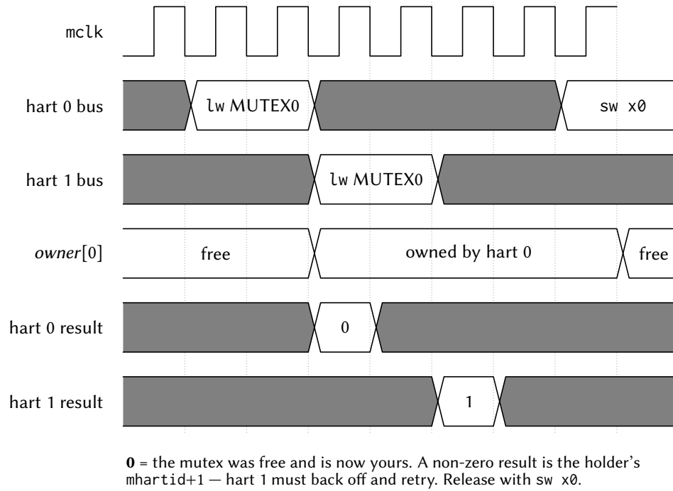
Figure 51: Two harts racing for the same mutex. The arbiter serializes the two claim reads, so the return-old-and-claim happens atomically with no retry loop: hart 0 reads 0 and thereby owns the mutex, and hart 1 reads hart 0's marker and must back off.
