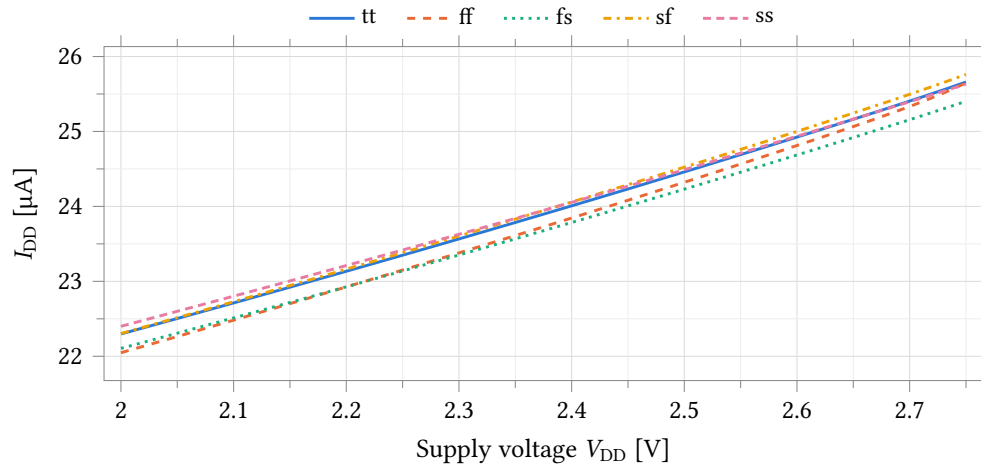
Figure 14: Quiescent supply current against supply voltage over all process corners.
