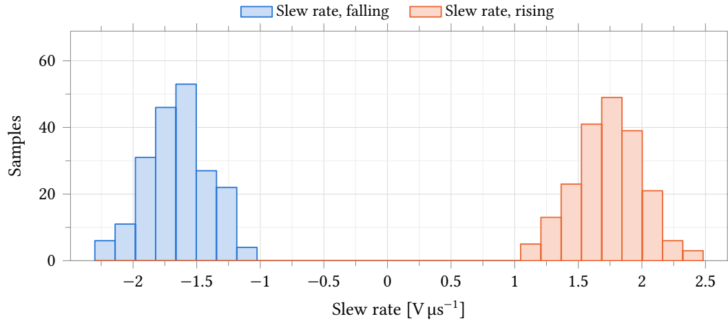
Figure 26: Slew rate on both edges of a 1 V step into 10 pF. Rising and falling averages are 1.74 \text{ V } \mu\text{s}^{-1} and 1.65 \text{ V } \mu\text{s}^{-1} , a 5 % imbalance: the tail current is steered into one input device and mirrored to the output, so the slewing current is equal in both directions by construction.
