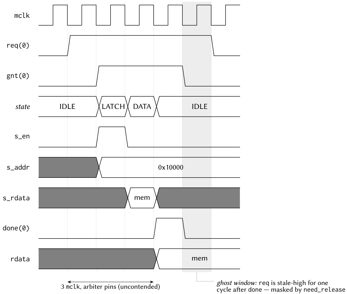
Figure 3: One uncontended shared-window read, at the mp_arbiter pins. The arbiter walks IDLE → LATCH → DATA : the transaction is presented to the slave for one cycle, the synchronous slave returns data the following cycle, and done and rdata are registered together at the edge leaving DATA — three mclk from an observed req . The hart itself sees about two cycles more, one in each direction across the registered tile boundary. In the shaded cycle the master's req is still high although its transaction is over; the arbiter masks that stale request until it is observed low, which is what stops a completed access from being served twice.
