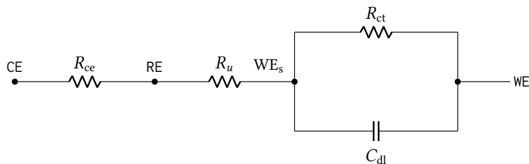
Figure 6: Three-electrode cell model randles_cell , the load the potentiostat actually drives. R_{ce} is the solution resistance from the counter to the reference electrode and R_u the uncompensated resistance from the reference to the working-electrode surface; the interface itself is the charge-transfer resistance R_{ct} in parallel with the double-layer capacitance C_{dl} . Values are given in Table 8. The model is lumped, linear and frequency-independent — no Warburg diffusion term and no potential dependence — so it represents small-signal behaviour about a bias point rather than a full electrochemical response.
