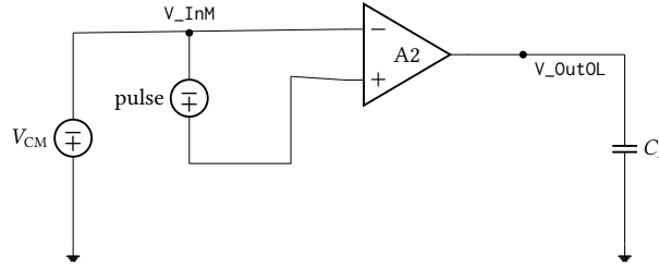
Figure 30: Open-loop slew testbench, SlewOpenLoopTB. The inverting input is held at V_{CM} and a floating pulse source drives the pair differentially rail to rail, into C_L = 5 pF. With no feedback the output is driven hard in both directions, so the slew rates of Table 30 are open-loop full-swing values and bound the closed-loop settling rate rather than equalling it.
