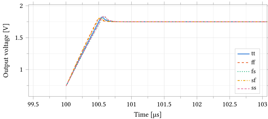
Figure 38: Rising edge of a 1 V step ( v_{cm} \pm 0.5 V) in unity feedback into 5 pF, over the five corners; the window is 3.5 \mu s around the edge at 100 \mu s, and the falling edge at 1.1 ms lies outside it. The output slews for about 0.4 \mu s, overshoots once by 5.0 % to 9.0 % of the step and recovers without ringing — slew recovery, not small-signal ringing, as the 88° phase margin predicts.
