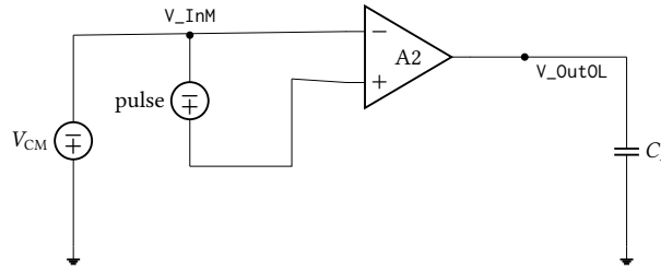
Figure 33: Open-loop slew testbench, SlewOpenLoopTB. The inverting input is held at V_{CM} and a floating pulse source drives the pair differentially rail to rail, into C_L = 5 pF. With no feedback the output is driven hard in both directions, so the slew rates of Table 30 are open-loop full-swing values and bound the closed-loop settling rate rather than equalling it.
