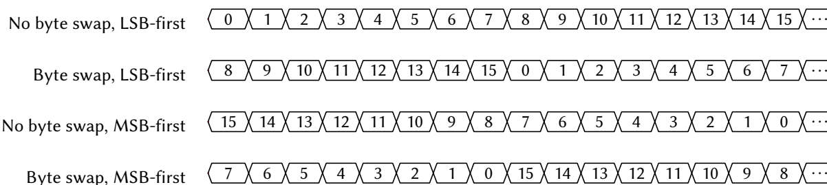
Figure 45: SPI Bit Ordering (16-bit transfer)
