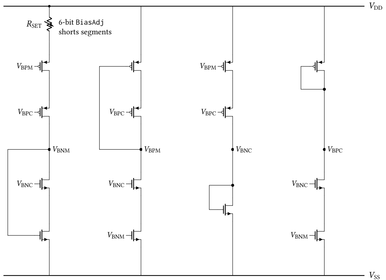
Figure 11: Simplified core of the local wide-swing cascode bias generator, drawn from the anatop_biasgen_local schematic. Four self-biased branches develop the four rails: the reference branch (left) passes the current set by the trimmable resistor R_{\text{SET}} , and the remaining branches mirror it to produce V_{\text{BPM}} , V_{\text{BNC}} and V_{\text{BPC}} . Each branch's own self-bias (diode) connection is drawn, from the rail it generates back to the gate it drives in the same branch; the cross-branch gate connections are identified by net name rather than drawn as buses. The enable switches, the decoupling capacitors on each rail and the individual segments of the resistor string are omitted for clarity.
