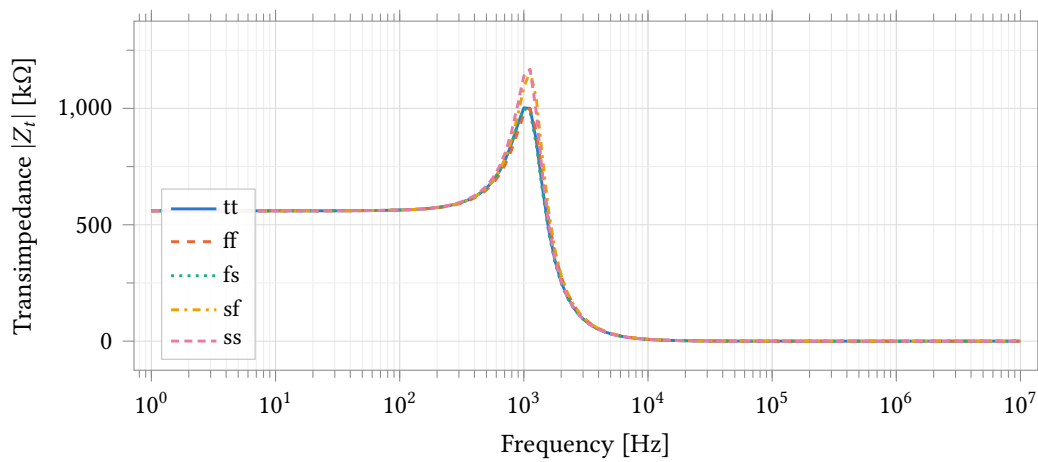
Figure 39: Transimpedance |Z_t| against frequency over the five corners, at maximum gain ( R_f = 560 kΩ) with 1 μF of double-layer capacitance at the working electrode. Flat at 560 kΩ to about 200 Hz, it peaks to 1.00 MΩ to 1.17 MΩ near 1 kHz. The peak is a marginally stable loop caused by C_{dl} rolling the feedback factor off from 0.28 Hz, not by the amplifier.
