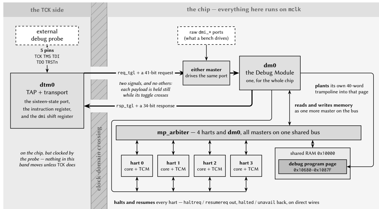
Figure 8: The debug path, from the probe to a hart, in a configuration built with debug support. The transport and the Debug Module sit in different clock domains , and the wall between them is crossed by exactly two signals — one toggle each way, each carrying a payload that is held still while its toggle is in flight. Everything to the right of that wall is ordinary chip fabric, and the one Debug Module reaches it in three ways: it halts and resumes the harts over direct wires, it reads and writes memory as one more master on the same arbiter the harts use, and it plants its own trampoline into the debug program page. The count of hart tiles follows this configuration.
