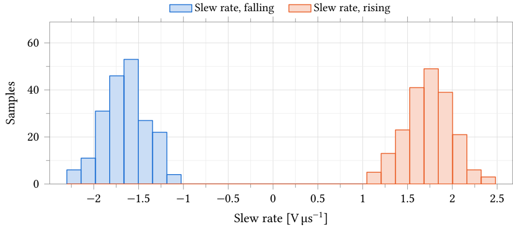
Figure 29: Slew rate on both edges of a 1 V step into 10 pF. Rising and falling averages are 1.74 \text{ V } \mu\text{s}^{-1} and 1.65 \text{ V } \mu\text{s}^{-1} , a 5 % imbalance: the tail current is steered into one input device and mirrored to the output, so the slewing current is equal in both directions by construction.
