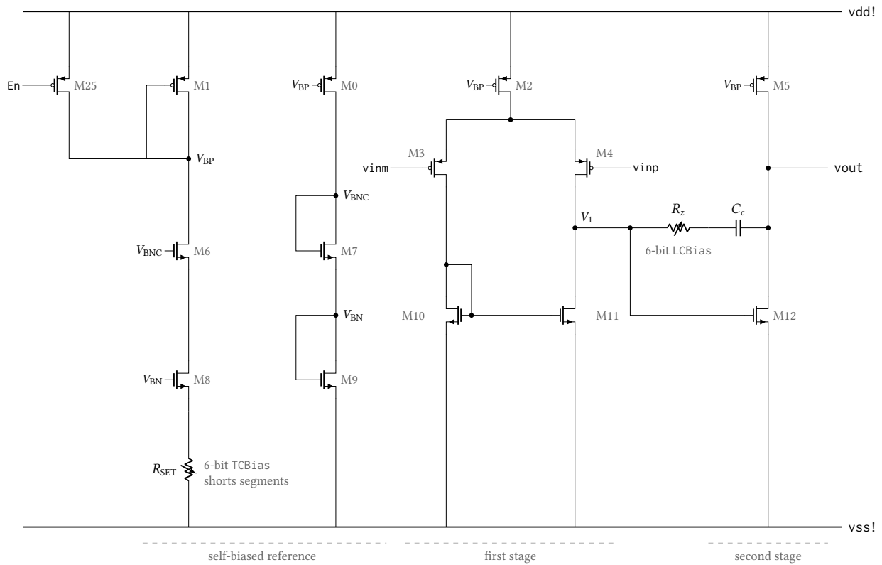
Figure 30: Simplified core of the transimpedance amplifier anatop_tiaamp , drawn from its netlist. First stage: PMOS pair M3/M4 on tail source M2 with NMOS current-mirror load M10/M11, output at V_1 ; second stage: common-source driver M12 with PMOS current-source load M5. The Miller branch R_z - C_c runs from V_1 to v_{out} , with M12's gate taken ahead of R_z ; C_c measures 1.00 pF. Being class A, the second stage sources the fixed current in M5 and sinks whatever M12 pulls — the asymmetry of Table 29. R_{SET} and R_z are each drawn as one trimmable resistor; both are segmented poly ladders with an NMOS shunt switch per trim bit. Device dimensions are omitted.
