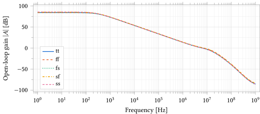
Figure 34: Open-loop gain over the five process corners, by stb through the feedback probe with the amplifier in unity feedback and a 5 pF load. Miller compensation gives a single-pole roll-off from 290 Hz to a 6.2 MHz to 7.6 MHz crossover. This is the amplifier alone; the loop that closes around the electrode is not this well behaved (Figure 39).
