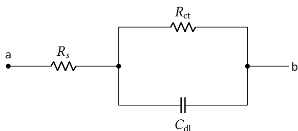
Figure 10: Single electrode–electrolyte interface, randles_electrode : a series solution resistance R_s ahead of the same charge-transfer and double-layer pair as Figure 9, presented as a two-terminal element. Values are given in Table 8; they describe a much smaller double layer and a much larger charge-transfer resistance than the three-electrode cell. None of the benches reported in this chapter uses it.
