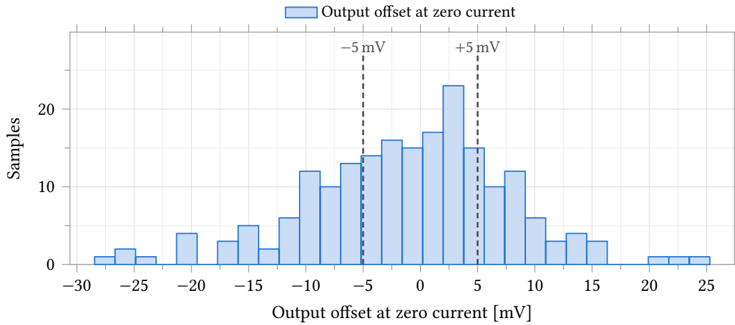
Figure 40: Output offset at zero electrode current, referred to v_{cm} . Process and mismatch , 37°C, 200 samples, R_f = 560 \text{ k}\Omega , C_f = 22 \text{ pF} , C_L = 5 \text{ pF} , C_c = 500 \text{ fF} , BiasAdj = 37, 2.5 V. The rules are the \pm 5 \text{ mV} limits entered on the test. \sigma = 8.91 \text{ mV} (sample deviation, as in every table of this section); 96 of 200 samples lie within the limits, 5.3 % across four independent channels. Statistics are in Table 34.
