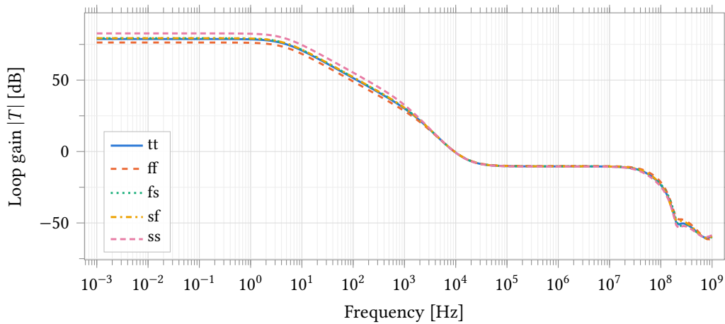
Figure 39: Transimpedance loop gain over five process corners, measured through a probe in series with the feedback network (Figure 36). R_f = 560 \text{ k}\Omega , C_f = 22 \text{ pF} , C_L = 5 \text{ pF} , C_c = 500 \text{ fF} , \text{BiasAdj} = 37 , 2.5 \text{ V} , Randles electrode with R_s = 100 \Omega , R_{ct} = 1 \text{ M}\Omega , C_{dl} = 100 \text{ nF} . tt is at 37^\circ\text{C} , the four skew corners at 25^\circ\text{C} . This is the loop around the amplifier, the feedback network and the electrode together, not the amplifier's own gain; the two are tabulated separately in Tables 30 and 31.
