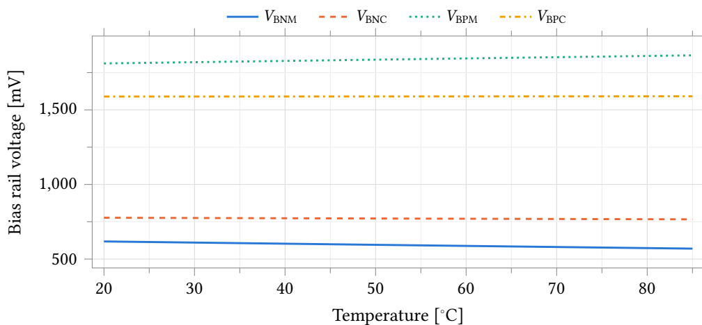
Figure 17: The four local bias rails against temperature at the typical corner. V_{\text{BNM}} and V_{\text{BNC}} are referred to vss!; V_{\text{BPM}} and V_{\text{BPC}} sit near the supply.
