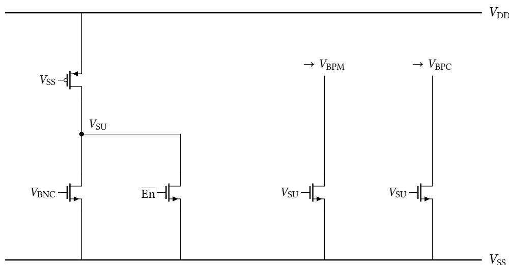
Figure 16: Start-up branch. A gate-grounded, permanently-on weak PMOS pulls V_{\text{SU}} up at power-on: while V_{\text{SU}} is high it drags V_{\text{BPM}} and V_{\text{BPC}} down, forcing current into the core and breaking the degenerate zero-current state. Once the core is running, the rising V_{\text{BNC}} turns on the left NMOS and collapses V_{\text{SU}} , so the branch draws no static current in normal operation, the behaviour visible in the power-up transient of Figure 24. A second device holds V_{\text{SU}} low whenever the cell is disabled.
