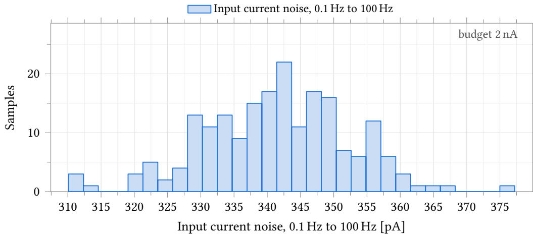
Figure 42: Input-referred current noise integrated 0.1 Hz to 100 Hz, conditions as Figure 40. Output noise divided by R_f , from a noise analysis that runs 0.1 Hz to 10 kHz at 20 points per decade. The 2 nA budget entered on the test is about six times the measured value and is annotated at the axis edge rather than drawn, so that the 310 pA to 377 pA spread stays legible. The figure scales inversely with the selected gain tap.
