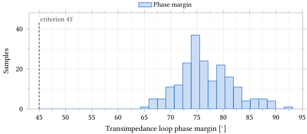
Figure 41: Phase margin of the transimpedance loop, conditions as Figure 40. The loop is measured through the feedback probe of Figure 36 and includes the amplifier, the feedback network and the Randles electrode ( R_s = 100 \Omega , R_{ct} = 1 \text{ M}\Omega , C_{dl} = 100 \text{ nF} ). All 200 samples clear the 45^\circ criterion, minimum 64.7^\circ . The distribution is right-skewed, so percentiles and the extreme sample are quoted in Table 36 rather than \pm 3\sigma .
