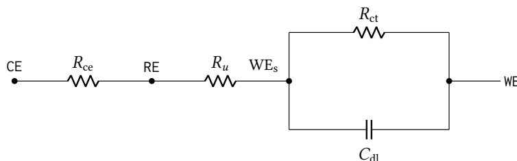
Figure 13: Three-electrode cell model randles_cell, the load the potentiostat actually drives. R_{ce} is the solution resistance from the counter to the reference electrode and R_u the uncompensated resistance from the reference to the working-electrode surface; the interface itself is the charge-transfer resistance R_{ct} in parallel with the double-layer capacitance C_{dl} . Values are given in Table 10. The model is lumped, linear and frequency-independent (no Warburg diffusion term and no potential dependence), so it represents small-signal behaviour about a bias point rather than a full electrochemical response.
