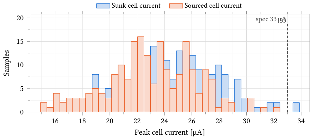
Figure 30: Peak current delivered into the cell, sinking and sourcing, over 200 process-and-mismatch samples. The two distributions overlap almost completely: mean source/sink imbalance is 6.4 %. Absolute drive falls short: 23.0 \mu\text{A} sourcing and 24.4 \mu\text{A} sinking against a 33 \mu\text{A} target, reached by 2 of 400 measurements. Roughly 1 V of headroom is left unused at each rail (Table 21), so the limit is current, not swing.
