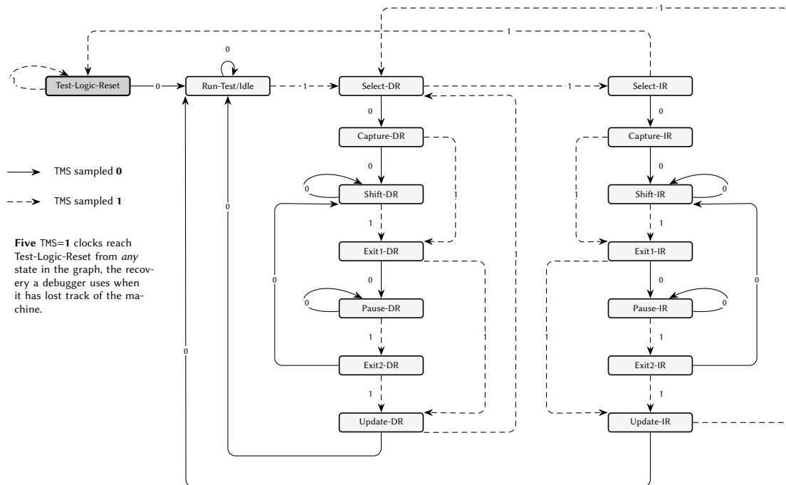
Figure 9: The sixteen-state JTAG test access port. Solid arrows are taken when TMS is sampled low, dashed when it is sampled high. The two lobes hanging below Select-DR and Select-IR are the same seven states drawn as mirror images of one another, one scanning a data register and one the instruction register. Note that five consecutive high samples reach Test-Logic-Reset from every state in the graph, which is the recovery a debugger uses when it does not know where the machine is.
