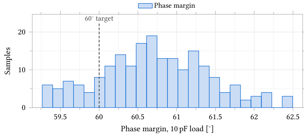
Figure 32: Phase margin driving the 10 pF test load. A cell load adds resistive loading that lowers the loop gain and raises the margin (Table 20). 171 of 200 samples meet the 60° design target: 85.5 % per channel, 53.4 % across four. Minimum sample 59.3°.
