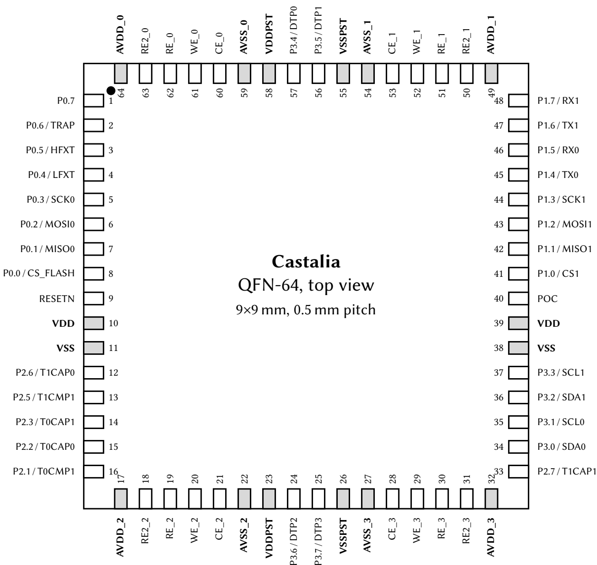
Figure 3: QFN-64 pinout, top view (9 × 9 mm, 0.5 mm pitch). Each pin is labeled with its pad name and, for GPIO pins, its AF0 (reset-selected) alternate function; power-rail pins are shaded and bold. The full per-pin alternate-function matrix is in Table 5.
