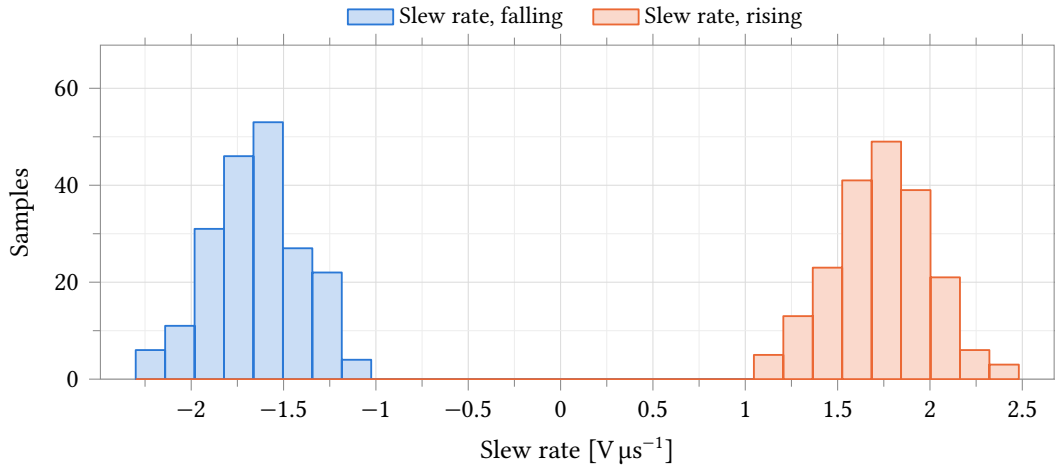
Figure 33: Slew rate on both edges of a 1 V step into 10 pF. Rising and falling averages are 1.74 \text{V } \mu\text{s}^{-1} and 1.65 \text{V } \mu\text{s}^{-1} , a 5 % imbalance: the tail current is steered into one input device and mirrored to the output, so the slewing current is equal in both directions by construction.
