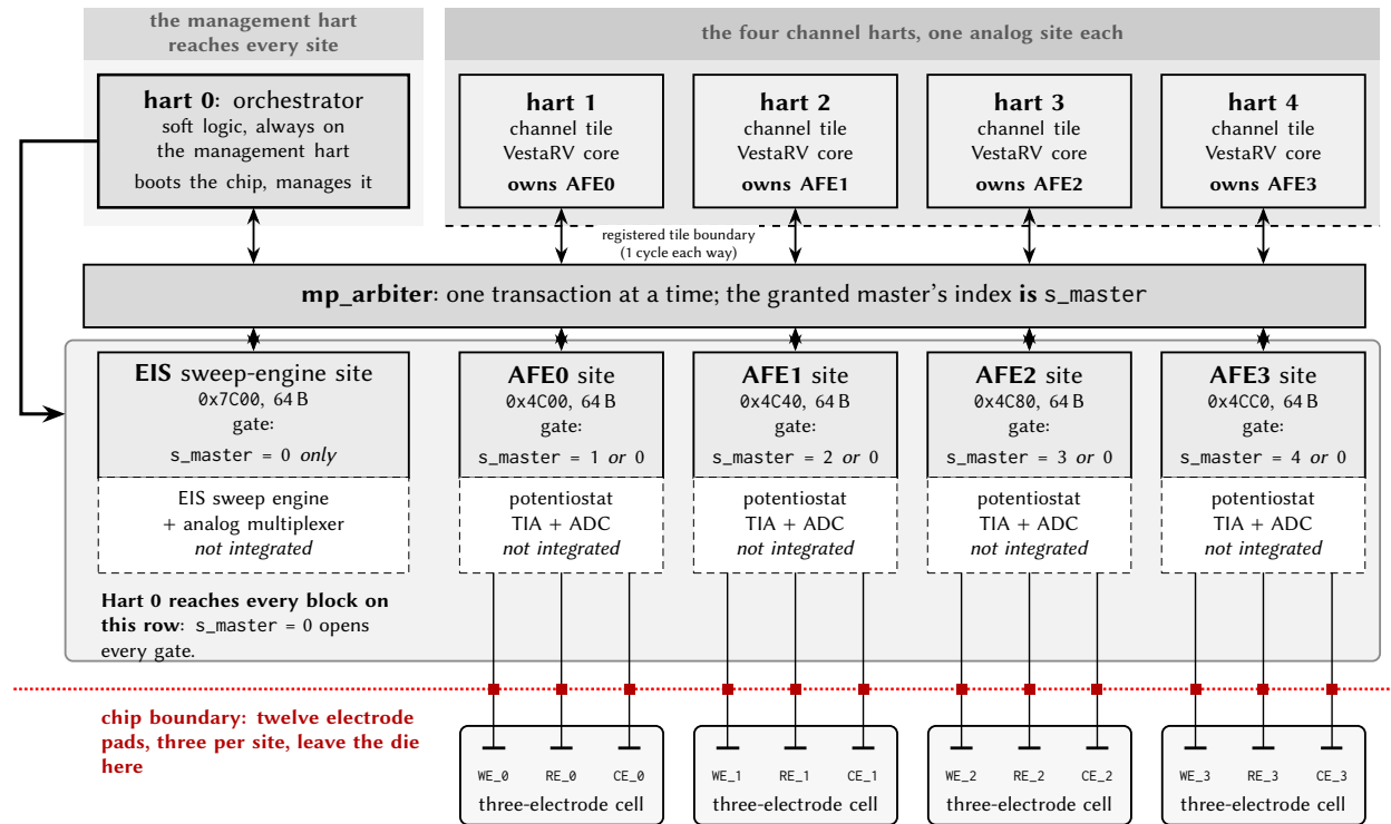
Figure 12: Analog front-end connectivity: who reaches which site, and what leaves the die. Each channel hart owns exactly one measurement site and reaches no other; hart 0, the orchestrator, opens every gate in the row, because the gate compares the arbiter’s granted-master index against a single owner and against 0. The analog stages are drawn dashed because they are not yet integrated: what the chip carries today is the digital register site in front of each one (and the pads behind them). Each site brings out a three-electrode cell: WE the working electrode, RE the reference, CE the counter. A fourth pad per site, RE 2h , is bonded as well and is not drawn: it is the second sense electrode of the optional four-terminal (Kelvin) configuration.
