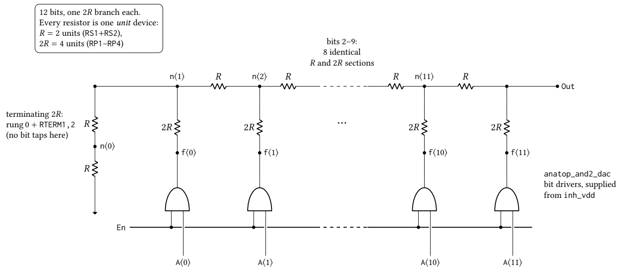
Figure 24.51: The 12-bit voltage-mode R – 2R ladder of anatot_pixel_dacR2R12 , transcribed from the DacNonLinTB netlist. Bit k drives tap n(k+1) through its own 2R branch, so the twelve taps are n(1) – n(11) plus Out, and the MSB branch lands directly on Out at the top of the ladder; n(0) carries no bit, its rung and R_{TERM1,2} together forming the terminating 2R . Bits 2–9 are elided: eight further sections identical to those drawn sit between n(2) and n(11) . Every element is the same unit resistor, so the network itself is exact and gives \text{Out} = (\text{code}/4096) V_{\text{ref}} ; the reference is the output high level of the anatot_and2_dac drivers, which sit in series with each 2R branch and bound the ladder in place of the rails: measured zero scale is 20 nV above V_{\text{SS}} and full scale 1.2 \mu\text{V} below the ideal (4095/4096) V_{\text{ref}} on a 2.5 V rail. Device dimensions are proprietary and are not stated.
