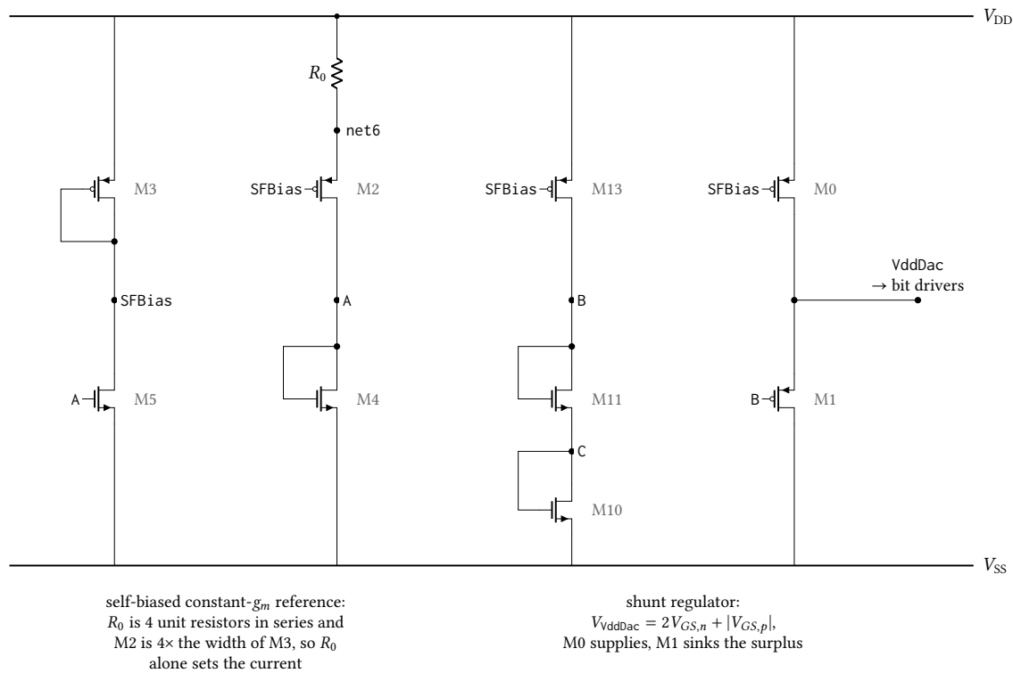
Figure 24.56: Core of anatop_pixel_dac_psu , the shunt regulator that generates the VddDac rail the ladder uses as its reference, transcribed from the LoadRegTB netlist. The self-biased constant- g_m reference on the left sets SFBias ; M_{13} drives that current through the stacked diodes M_{11} and M_{10} to hold B two gate-source voltages above V_{\text{SS}} , and M_1 sinks whatever of M_0 's current the ladder leaves, clamping VddDac one PMOS gate-source voltage above B : 2.177 V unloaded from a 2.5 V rail. There is no error amplifier, so load regulation is set by M_1 's g_m alone. The five start-up and enable devices (the weak pull-up and its two kick devices on SU , the shutdown pull-up on SFBias and the En inverter) are omitted; none carries current once the loop is running. Device dimensions are proprietary and are not stated.
