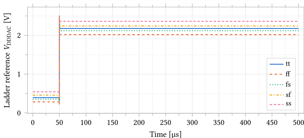
Figure 84: V_{DDDAC} against time over five process corners, PSUStartupTB: En rises at 50 \mu\text{s} into a 500 \mu\text{s} window at zero external load, 27 °C at point 1 and 25 °C at points 2–5. With En low the node sits at 0.28 V to 0.54 V; at the 1 ns enable edge the pass device is driven hard on and the node is pulled to the 2.5 V supply rail for 64 ns to 100 ns before falling back. It reaches the zero-load DC value of Table 82 to within 140 \mu\text{V} at every corner and holds it to the end of the window. No settling-time or overshoot figure of merit is published from this bench: the design variable t_{\text{win}} sets both the En pulse width and the settlingTime evaluation window, so the two cannot be specified independently.
