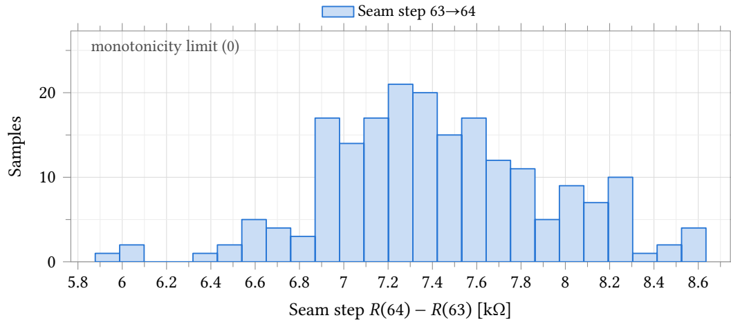
Figure 69: Per-sample step across the first thermometer seam (code 63 to 64: one 64-unit segment switches in while all six binary segments switch out), the code transition most exposed to mismatch. Mismatch only , model section castalia_pm_25 , nominal process, 200 samples, seed 12345, low-discrepancy sampling, 25 °C. Mean 7.42 kΩ, \sigma = 504 \Omega , worst sample 5.88 kΩ – 14.7 \sigma above the monotonicity limit at zero, so no realistic mismatch closes the seam.
