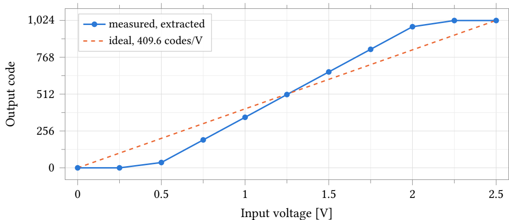
Figure 62: Output code against input voltage for the extracted anatot_pixel_adc , nominal corner, 37 °C, 2.5 V analog and 1.0 V digital supplies, with the ideal 409.6 codes/V line overlaid. The transfer is monotonic and reaches both code limits, but its slope is 628.64 codes/V — 1.535 times ideal — so the flat segments below 0.44 V and above 2.07 V are the code limits, not the ends of the sweep. Markers are the eleven simulated points; the 0.25 V step is 157 codes, so the curve between them is interpolation and carries no linearity information.
