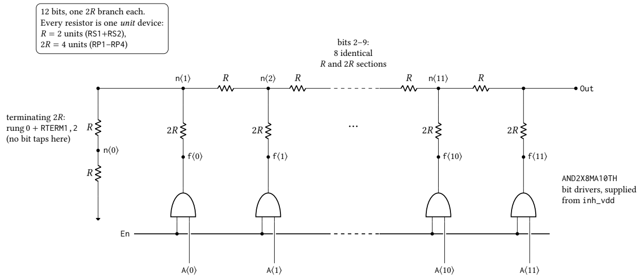
Figure 71: The 12-bit voltage-mode R-2R ladder of anatop_pixel_dacR2R12 , transcribed from the DacNonLinTB netlist. Bit k drives tap n\langle k+1 \rangle through its own 2R branch, so the twelve taps are n\langle 1 \rangle – n\langle 11 \rangle plus Out , and the MSB branch lands directly on Out at the top of the ladder; n\langle 0 \rangle carries no bit, its rung and RTERM1,2 together forming the terminating 2R . Bits 2–9 are elided: eight further sections identical to those drawn sit between n\langle 2 \rangle and n\langle 11 \rangle . Every element is the same unit resistor, so the network itself is exact and gives \text{Out} = (\text{code}/4096) V_{\text{ref}} ; the reference is the output high level of the AND2X8MA10TH drivers, which sit in series with each 2R branch and bound the ladder in place of the rails — measured zero scale is 90 \mu\text{V} above V_{\text{SS}} and full scale 103 \mu\text{V} below the ideal (4095/4096) V_{\text{ref}} on a 2.5 V rail. Device dimensions are proprietary and are not stated.
