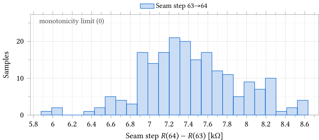
Figure 70: Per-sample step across the first thermometer seam (code 63 to 64: one 64-unit segment switches in while all six binary segments switch out), the code transition most exposed to mismatch. Mismatch only , model section castalia_pm_25 , nominal process, 200 samples, seed 12345, low-discrepancy sampling, 25 °C. Mean 7.42 k \Omega , \sigma = 504 \Omega , worst sample 5.88 k \Omega – 14.7\sigma above the monotonicity limit at zero, so no realistic mismatch closes the seam.
