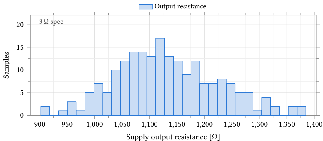
Figure 82: Output resistance of the DAC supply block, taken as the chord \Delta V / \Delta I over a 0 \mu\text{A} to 100 \mu\text{A} load sweep on V_{\text{DDDAC}} . Process and mismatch , castalia_pm_25, 200 samples, 27^\circ\text{C} . The 3 \Omega limit entered on the test is two orders of magnitude below the data and is annotated at the left axis edge rather than drawn; no sample meets it. This is not a second defect: the reference movement of Figure 80 is this impedance multiplied by the ladder's own code-dependent reference current.
