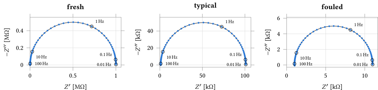
Figure 58: Nyquist arcs of the three electrode models measured by the channel itself (dots, all 143 of them) against the analytic impedance of the load (line), 0.01 Hz to 100 kHz at 20 points per decade, gain code 0, nominal process point, 37 °C, with the applied potential read at the reference electrode and the current measured; rings mark the decades 0.01 Hz, 0.1 Hz, 1 Hz, 10 Hz and 100 Hz. The three panels have independent scales — the loads span 1 MΩ, 100 kΩ and 10 kΩ — and each has equal axes, so a semicircle reads as a semicircle and a departure from a circle is a measurement and not an aspect ratio. The plotting grid is no longer the limit: the chord polygon through the plotted points departs the true arc by 0.165 % of the arc radius, against 0.651 % at the archived ten points per decade and an instrument error of 0.30 %. Agreement is within 0.44 % of magnitude and 1.03° of phase below 20 kHz on all three loads, rising to 2.94 % and 4.67° at 100 kHz. A small-signal analysis has no dynamic-range limit, which the readout does: gain code 0 covers 236 Ω to 150.9 kΩ, so the fresh arm above 151 kΩ would be taken at gain code 20 in firmware.
