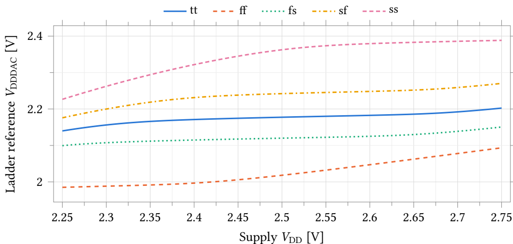
Figure 83: V_{\text{DDDAC}} against the supply, swept 2.25 \text{ V} to 2.75 \text{ V} , over five process corners at zero external load, 27^\circ\text{C} at point 1 and 25^\circ\text{C} at points 2–5. The slope is the line regulation tabulated in Table 87; it is not constant across the sweep, so the tabulated value is the chord between the two endpoints. The corner spread of the reference itself, 344 \text{ mV} at nominal supply, is larger than anything the supply sweep produces.
