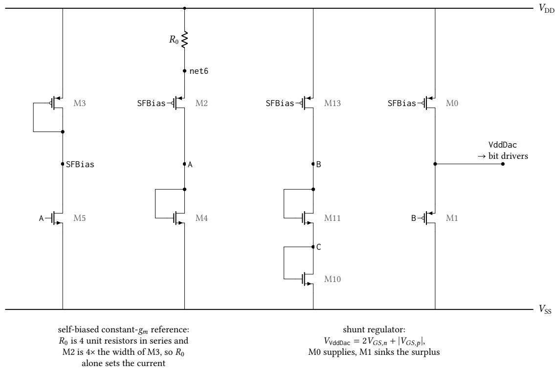
Figure 74: Core of an atop_pixel_dac_psu , the shunt regulator that generates the VddDac rail the ladder uses as its reference, transcribed from the LoadRegTB netlist. The self-biased constant- g_m reference on the left sets SFBias ; M_{13} drives that current through the stacked diodes M_{11} and M_{10} to hold B two gate-source voltages above V_{SS} , and M_1 sinks whatever of M_0 's current the ladder leaves, clamping VddDac one PMOS gate-source voltage above B : 2.177 V unloaded from a 2.5 V rail. There is no error amplifier, so load regulation is set by M_1 's g_m alone. The five start-up and enable devices — the weak pull-up and its two kick devices on SU , the shutdown pull-up on SFBias and the En inverter — are omitted; none carries current once the loop is running. Device dimensions are proprietary and are not stated.
