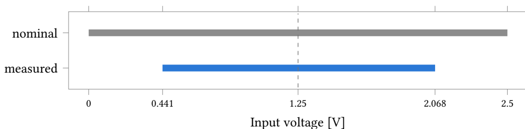
Figure 64: Usable input window of the converter against the nominal 0 V to 2.5 V supply span. The measured window runs 0.441 V to 2.068 V, 1.627 V wide, so 34.9\% of the nominal span is unreachable — 0.441 V at the bottom and 0.432 V at the top, near enough symmetric about the 1.25 V common mode (dashed). Outside that window the output sits at a code rail, so a transimpedance swing wider than \pm 0.81 V about V_{CM} is truncated rather than digitised.
