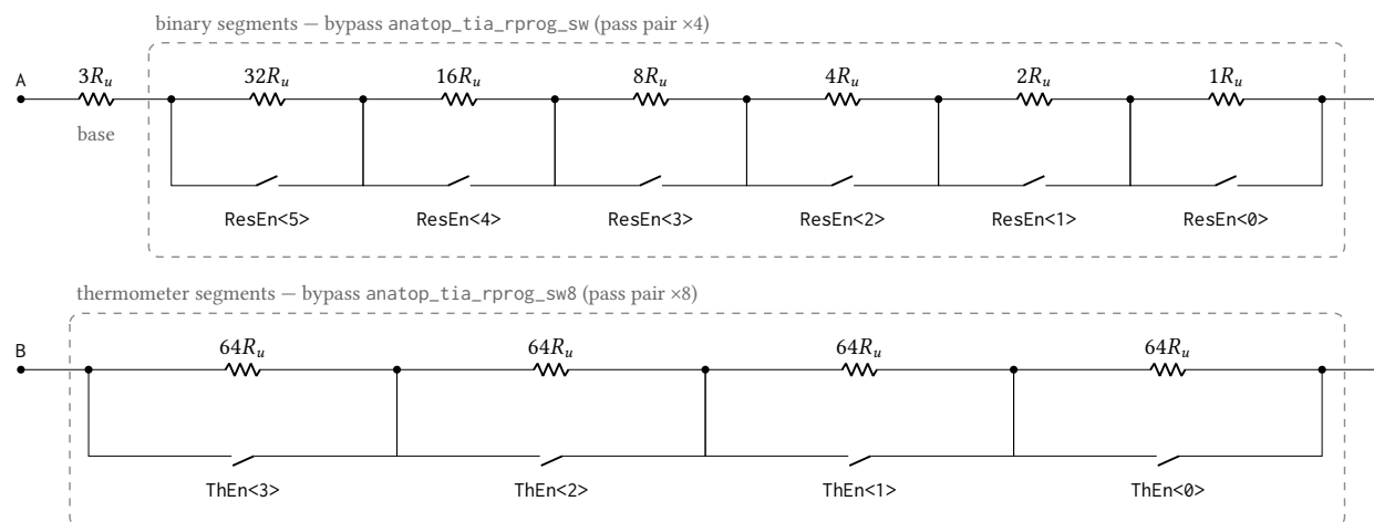
Figure 66: Segment and bypass-switch structure of anatop_tia_rprog, transcribed from the executed spec-run netlist. The unit R_u is one series poly resistor; from terminal A the chain runs through the never-switched three-unit base, the six binary-weighted segments of 32 down to 1 unit, and the four identical 64-unit thermometer segments to terminal B. Each switched segment is shunted by a CMOS transmission gate with a local inverter: the control pin EnBar is the ResEn/ThEn bit itself and drives the PMOS pass gate directly and the NMOS pass gate through the inverter, so a bit at 1 turns both pass devices off and inserts the segment. The pass pair has multiplicity 4 in the binary switch ( _sw ) and 8 in the thermometer switch ( _sw8 ), which halves the thermometer gates' on-resistance where up to six binary gates close at a seam. Three grounded dummy units accompany the 322 active units for matching.
