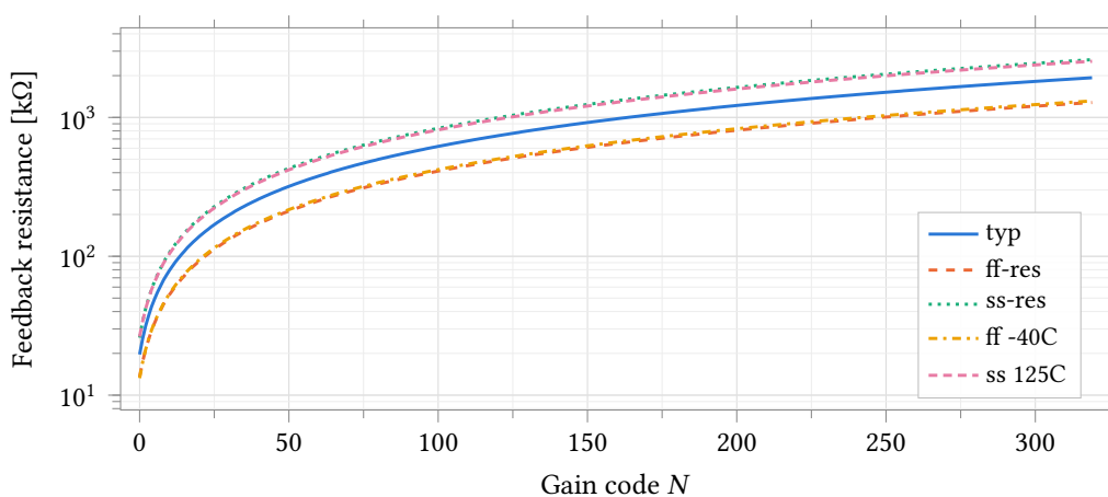
Figure 67: Measured resistance against gain code at all five corners, 500 nA forced through the A–B terminals with B held at V_{CM} = 1.25 V. The law is R = 18 \text{ k}\Omega + 6 \text{ k}\Omega \cdot N with N the binary value of ResEn<5:0> plus 64 per set ThEn<3:0> thermometer bit; every corner is strictly monotonic over all 320 codes, including the four thermometer seams. The corner families move the absolute value by -33 to +35 %, which is the poly sheet-resistance tolerance and must be absorbed by gain calibration, not by code choice.
