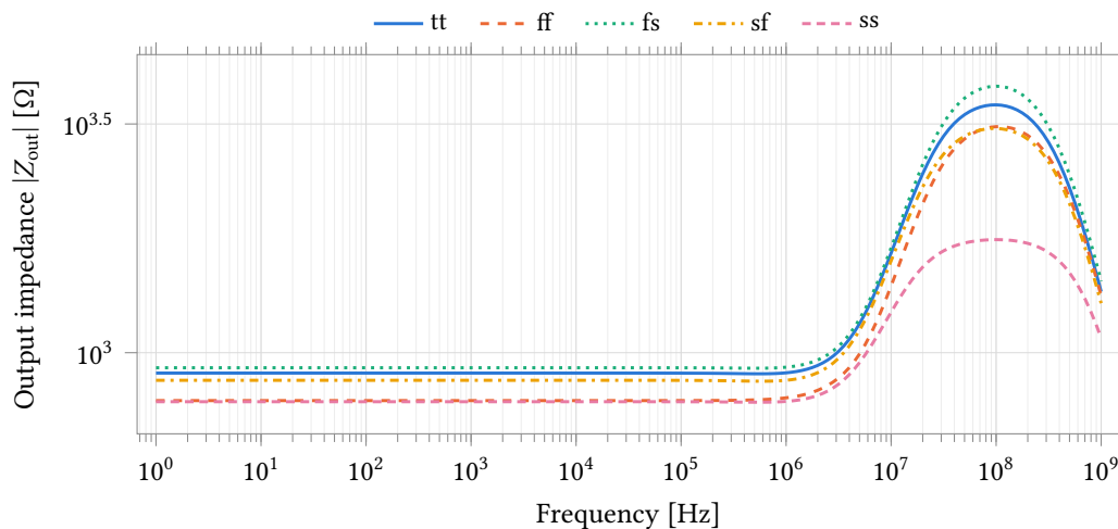
Figure 83: Magnitude of the supply block’s output impedance against frequency over five process corners, 27 °C at point 1 and 25 °C at points 2–5. The AC load source carries unit magnitude, so |V_{DDDAC}| is the impedance in ohms. It is flat at 781 Ω to 927 Ω from 1 Hz to 100 kHz and peaks at 1.8 kΩ to 3.8 kΩ near 100 MHz. This is the small-signal impedance at zero load; the large-signal chord over the 0 μA to 100 μA sweep is 18 % to 51 % higher (Table 86).
