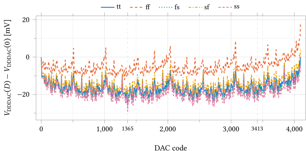
Figure 74: Ladder reference V_{DDAC} referred to its value at code 0, against DAC code, over five process corners, DacWPSUTB at 25 °C with the external load current set to zero. The ladder is the only load on the supply block and its current is code-dependent, so the reference the ladder divides moves 25.7 mV to 29.6 mV peak-to-peak with no external load at all; the absolute levels, which differ by 357 mV across corners, are Table 80. The two marked codes are alternating-bit patterns: 1365 = 0b010101010101 is the global minimum at four of the five corners (1317 at ff), and 3413 = 1365 + 2048 droops 23.4 mV at 2.5× the code weight and therefore sets the worst raw INL of Figure 75. Reference droop times code accounts for −36.9 of the −37.1 LSB measured there, so the raw nonlinearity of the delivered block is reference modulation and not a ladder error.
