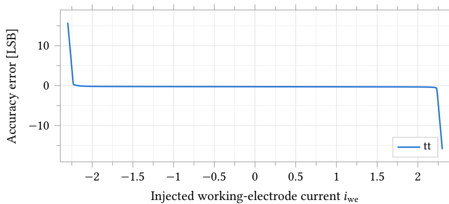
Figure 51: Accuracy error at the operational max-gain point, R_f = 560\text{ k}\Omega into R_{ct} = 1\text{ M}\Omega , typical process point, 37\text{ }^\circ\text{C} . The truth current sweep is \pm 2.3\text{ }\mu\text{A} , just beyond the 2.06\text{ }\mu\text{A} full-scale current at this gain tap; the crossing at zero is smooth, with no kink, over the full swept range shown. The error axis is referred to the nominal 2.441\text{ mV} step; the converter's measured step is 1.591\text{ mV} (Table 68), so multiply by 1.535 to read it as converter codes.
