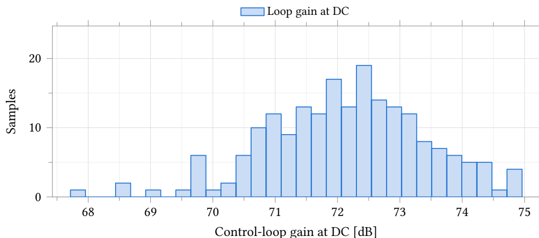
Figure 48: DC gain of the control loop closed around an electrochemical cell. Process and mismatch , 37 °C, 200 samples, cell-drive bench (Figure 46) with a Randles cell of R_{CE} = 1 \text{ k}\Omega , R_u = 1 \text{ k}\Omega , R_{ct} = 10 \text{ k}\Omega , C_{dl} = 1 \text{ }\mu\text{F} , working electrode at 1.25 V, C_L = 5 \text{ pF} , C_c = 500 \text{ fF} , 2.5 V supply. The loop is measured through the reference-electrode sense wire and therefore includes the cell, whose 12 k \Omega loads an open-loop output resistance of about 25 k \Omega and is 10 dB below the unity-feedback gain of Table 31. The spread is 7 dB peak to peak and no sample falls below 67 dB. No limit was entered on this output.
