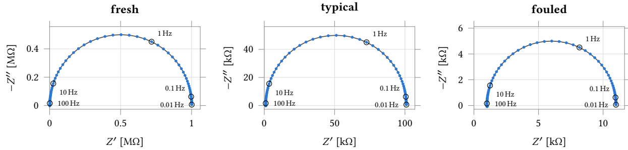
Figure 58: Nyquist arcs of the three electrode models measured by the channel itself (dots, all 143) against the analytic impedance of the load (line), 0.01 Hz to 100 kHz at 20 points per decade, gain code 0, nominal process point, 37 °C, with the applied potential read at the reference electrode and the current at the transimpedance output; rings mark the decades 0.01 Hz, 0.1 Hz, 1 Hz, 10 Hz and 100 Hz. The three panels have independent scales — 1 MΩ, 100 kΩ and 10 kΩ — and each has equal axes, so a departure from a circle is a measurement and not an aspect ratio. The plotting grid is not the limit: the chord polygon through the plotted points departs the true arc by 0.165 % of the arc radius, against 0.651 % at ten points per decade and an instrument error of 0.30 %. Agreement is within 0.44 % of magnitude and 1.03° of phase below 20 kHz on all three loads, rising to 2.94 % and 4.67° at 100 kHz. A small-signal analysis has no dynamic-range limit, which the readout does: gain code 0 covers 236 Ω to 150.9 kΩ, so the fresh arm above 151 kΩ would be taken at gain code 20 in firmware.
