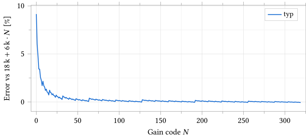
Figure 67: Typical-corner deviation from the ideal code law. The +9.2 % at N = 0 is the series resistance of the ten closed bypass switches (1.65 k \Omega , about 165 \Omega each), which decays as 1/R once real ladder segments dominate; by N = 319 the error is -0.063 %. The ripple is the carry structure: at each binary carry and at each thermometer seam the set of closed switches changes, so the R_{on} term steps while the ladder term is exact.
