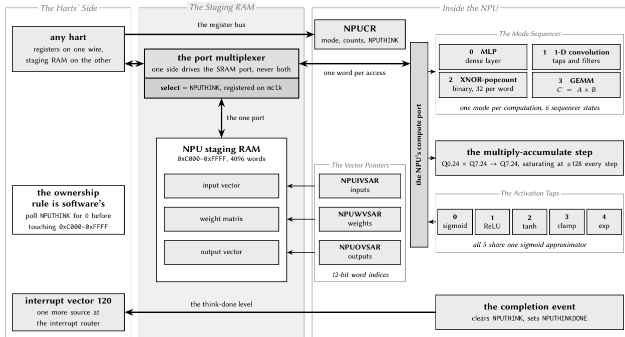
Figure 97: The NPU datapath, and the staging RAM it borrows. The picture draws the shape; this caption carries the contracts. The staging RAM is one 16 KiB single-port SRAM macro, so the whole middle band is about which side of it is driving that one port. The multiplexer's select is NPUTHINK re-clocked on the free-running chip clock, which is why the port changes hands a full cycle after a hart's start write lands and a full cycle after the engine's completion pulse: a hart's in-flight access can never be cut in half by the switch. What the hardware does not do is stop a hart reaching into the window while the engine has it — no hart is put to sleep, the access completes at the arbiter in the ordinary three cycles, and what comes back is whatever the SRAM is holding for the engine — which is why the rule in the left band is software's and the poll on NPUTHINK is the whole of it. NPUIVSAR, NPUWVSAR and NPUOVSAR are word indices into that one array, not addresses of three separate memories; firmware places and sizes all three, and the sequencer bounds-checks none of it, so an oversized working set wraps and corrupts its neighbours. Behind the port there is one engine: one mode per computation, latched into run shadows at the NPUTHINK edge, with mode codes 4–7 running as mode 0; one multiply-accumulate step that rounds to nearest and saturates on every single step rather than once at the end; and one piecewise-quadratic sigmoid approximator that all five activation taps are shift-and-add wrappers around, with activation codes 5–7 reading as sigmoid and \text{NPUAEN} = 0 writing the raw accumulator whatever \text{NPUACTF} says. The completion pulse does three things at once — it clears NPUTHINK, which is what hands the port back one clock edge later; it sets the sticky, write-1-to-clear NPUTHINKDONE in NPUSR; and the interrupt is the level of that flag gated by NPUTDIE, on the free-running clock.
