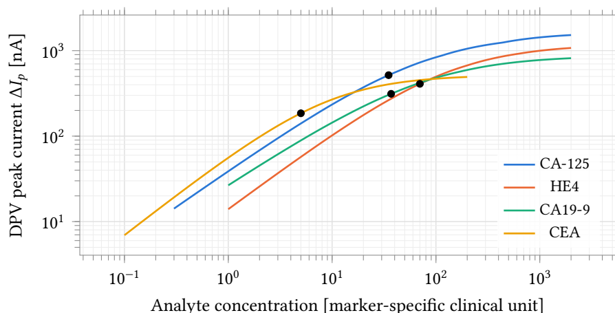
Figure 24: Dose response of the four-reporter panel: published-assay binding curves composed with the current transfer measured from the DPV runs of Figure 23 (11 simulated concentrations per reporter, 560 kΩ tap). Filled circles are the clinical decision points through the same chain: CA-125 35 U/mL → 517 nA, HE4 70 pmol L -1 → 409 nA, CA19-9 37 U/mL → 313 nA, CEA 5 ng mL -1 → 185 nA. The concentration axis carries each marker's own clinical unit; only the current axis is common. The binding model is analytic; the electrode and channel behind the current axis are simulated.
