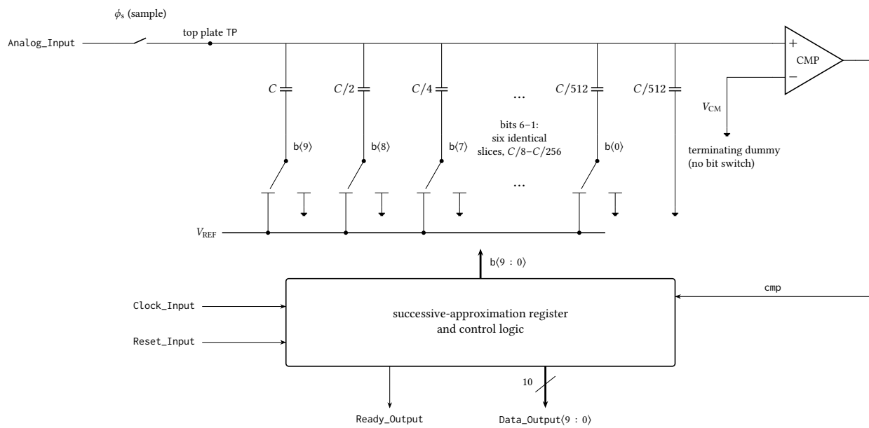
Figure 59: Generic single-ended charge-redistribution SAR ADC, drawn to explain the architecture of the 10-bit converter rather than to reproduce its implemented transistor-level schematic. The input is sampled through \phi_s onto the top plate of a binary-weighted array; the logic then switches each bottom plate from V_{REF} to ground one bit at a time, most significant first, and keeps or discards the trial from the comparator decision, so the conversion takes ten comparator cycles and the top plate converges to V_{CM} . Bits 6–1 are elided: six further slices identical to those drawn sit between C/4 and C/512 , and the terminating dummy C/512 carries no bit switch, which makes the total array 2C and the LSB weight C/512 . Only the external port names are those of the implemented block; the sampling network, comparator topology, clock generation and reset behaviour are representative, and no device dimensions are stated.
