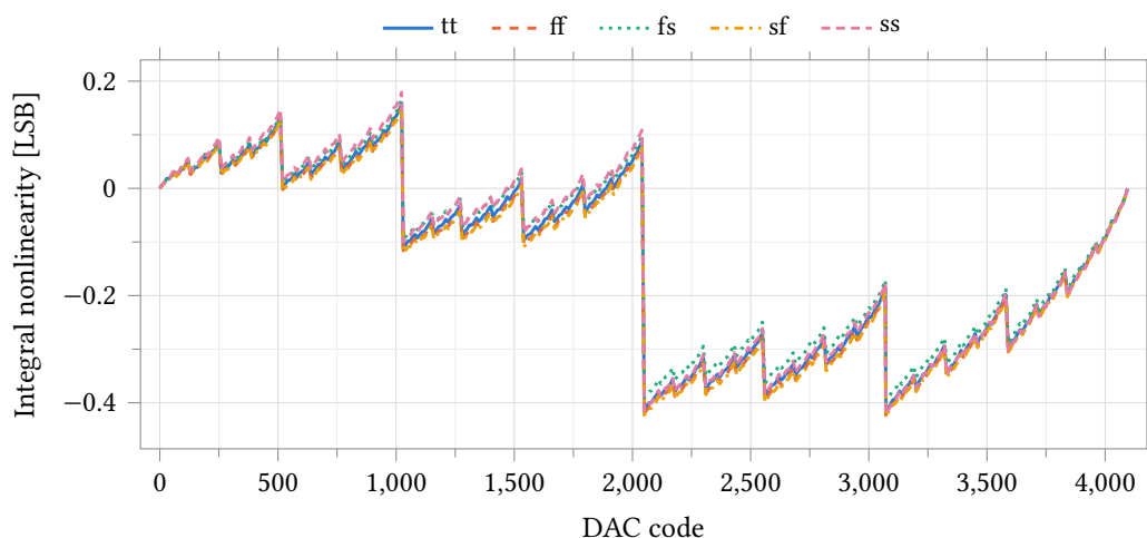
Figure 71: Integral nonlinearity against code over five process corners, ladder on an ideal 2.5 V rail, 25 °C, \text{reltol} = 1 \times 10^{-6} . INL is taken from the endpoint line through each corner's own zero- and full-scale outputs, so it is zero at codes 0 and 4095 by construction. The positive extreme is code 1023, +0.15 to +0.18 LSB; the negative extreme is shared by the major carries at codes 2048 and 3072, which sit within 0.006 LSB of each other at -0.39 to -0.43 LSB at every corner. The code of each extreme is the same at all five corners: the shape is set by the ladder, not by the process. Corner run, no device mismatch — R-2R linearity is a matching property, so this envelope is the systematic term alone.
