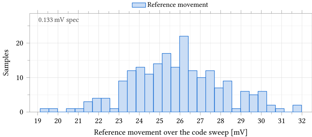
Figure 79: Peak-to-peak movement of the DAC reference V_{ddDac} across the 4096-code sweep, with the ladder referenced to the on-chip supply block instead of an ideal rail. Process and mismatch , castalia_pm_25 , 200 samples, 25 °C, no external load on V_{ddDac} . The quarter-LSB budget of 133 \mu V entered on the test sits about 200 times below the data, so it is annotated at the left axis edge rather than drawn and the distribution is not compressed into a single bar; the closest sample misses it by a factor of 144. Meeting it needs the supply’s output impedance down by a factor of 193, to about 5 \Omega , against 894 \Omega small-signal (Table 91) and 1133 \Omega as a 0 \mu A to 100 \mu A chord (Table 87).
