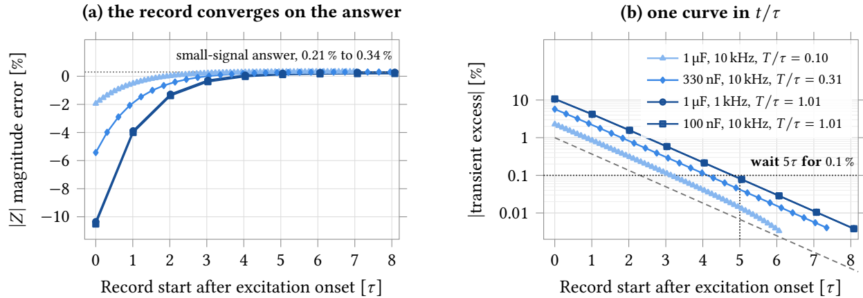
Figure 65: Impedance-magnitude error against how late the demodulation window starts, in units of the electrode's dc step time constant \tau = C_{dl}(R_u \parallel R_{ct}) , for four conditions spanning 10\times in \tau ( 99\mu\text{s} to 990\mu\text{s} ) and 10\times in excitation frequency, all on the correctly gain-ranged code 0 and all in compliance ( \max |V_{OUT} - v_{cm}| 0.358 V to 0.447 V of 0.80 V); each run asymptotes to the small-signal analysis of its own load and code within 0.003 to 0.009 percentage points, which is what validates the demodulator. (b) plots the excess over each run's own asymptote, and it is a function of t/\tau alone: colour is ordered by T/\tau rather than naming a condition, so the two runs whose \tau and frequency differ 10\times at matched T/\tau share one colour, and that their marks lie on top of each other — 0.69% apart at every point — is the result. All four decay as \exp(-t/\tau) , giving the rule wait 5\tau for 0.1% and 7\tau for 0.01% ; amplitude, not decay rate, is set by the demodulation window, so eight cycles taken at the onset still leave -2.3\% and sixteen -1.2\% and averaging is not a substitute for waiting. The published +16.4\% and +74\% are deliberately not plotted: those records sit on a gain code whose own minimum measurable impedance is 1.67\times this load, with the output at 1.25 V against a \pm 0.80 V window, and they asymptote at +8.6\% and +8.1\% against small-signal answers of 1.08% and 2.40% — saturation, not settling. On code 0 the same eight-cycle record at the onset reads -2.00\% and -1.32\% , 8\times and 56\times smaller and the opposite sign.
