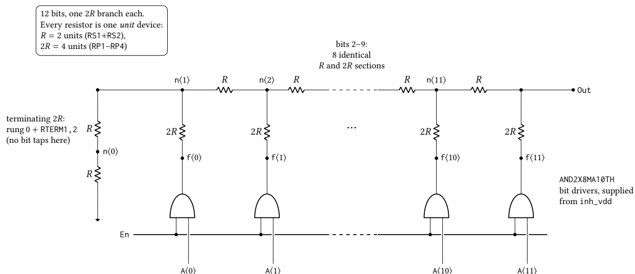
Figure 77: The 12-bit voltage-mode R-2R ladder of anatot_pixel_dacR2R12 , transcribed from the DacNonLinTB netlist. Bit k drives tap n\langle k+1 \rangle through its own 2R branch, so the twelve taps are n\langle 1 \rangle – n\langle 11 \rangle plus Out , and the MSB branch lands directly on Out at the top of the ladder; n\langle 0 \rangle carries no bit, its rung and RTERM1,2 together forming the terminating 2R . Bits 2–9 are elided: eight further sections identical to those drawn sit between n\langle 2 \rangle and n\langle 11 \rangle . Every element is the same unit resistor, so the network itself is exact and gives \text{Out} = (\text{code}/4096) V_{\text{ref}} ; the reference is the output high level of the AND2X8MA10TH drivers, which sit in series with each 2R branch and bound the ladder in place of the rails — measured zero scale is 90 \mu\text{V} above V_{\text{SS}} and full scale 103 \mu\text{V} below the ideal (4095/4096) V_{\text{ref}} on a 2.5 V rail. Device dimensions are proprietary and are not stated.
