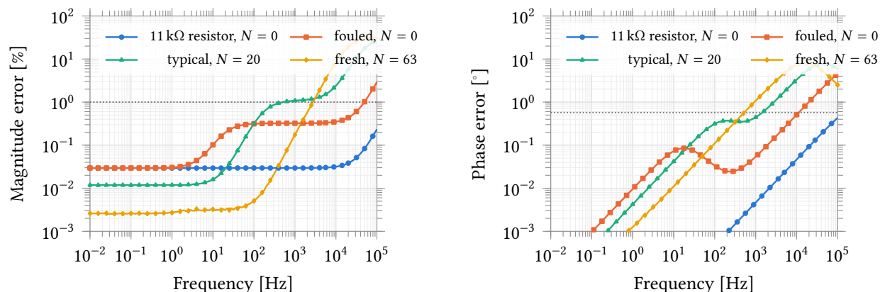
Figure 64: Measured impedance error against frequency — magnitude (left) and phase (right) — for the calibration resistor and the three electrode cases, each at the gain code that ranges it, with the applied potential read at the reference electrode and the current measured, over 0.01 Hz to 100 kHz at 20 points per decade at the nominal process point and 37 °C. Every frequency is drawn; markers are thinned to one point in four so the curves stay legible. Error is taken against the analytic impedance of the load, so these are the chain’s errors and not the model’s; dotted lines are the 1 % and 0.573° gates. Each curve turns up where the electrode’s impedance has collapsed toward R_u = 1\text{ k}\Omega and the noise gain 1 + R_f/|Z| has therefore risen, which is why the highest-gain case is the most accurate below 100 Hz and the first to degrade above 1 kHz. The gate crossings here are not the bandwidth specification: the ratio R_f/|Z| moves with frequency on a real electrode, and the specification comes from the fixed-ratio measurement of Section 8.7.2.
