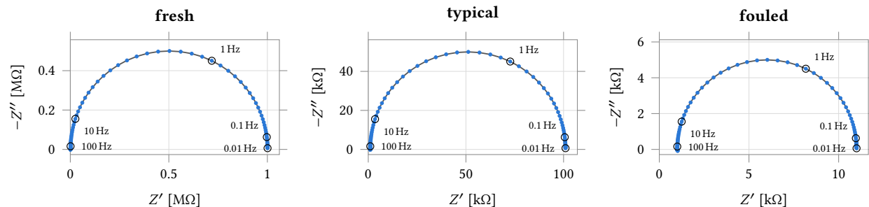
Figure 61: Nyquist arcs of the three electrode models measured by the channel itself (dots, all 143 of them) against the analytic impedance of the load (line), 0.01 Hz to 100 kHz at 20 points per decade, gain code 0, nominal process point, 37 °C, with the applied potential read at the reference electrode and the current measured; rings mark the decades 0.01 Hz, 0.1 Hz, 1 Hz, 10 Hz and 100 Hz. The three panels have independent scales — the loads span 1 M \Omega , 100 k \Omega and 10 k \Omega — and each has equal axes, so a semicircle reads as a semicircle and a departure from a circle is a measurement and not an aspect ratio. The plotting grid is no longer the limit: the chord polygon through the plotted points departs the true arc by 0.165 % of the arc radius, against 0.651 % at the archived ten points per decade and an instrument error of 0.30 %. Agreement is within 0.44 % of magnitude and 1.03° of phase below 20 kHz on all three loads, rising to 2.94 % and 4.67° at 100 kHz. A small-signal analysis has no dynamic-range limit, which the readout does: gain code 0 covers 236 \Omega to 150.9 k \Omega (Table 70), so the fresh arm above 151 k \Omega would be taken at gain code 20 in firmware.
