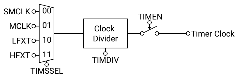
Figure 99: TIMERx Clock Diagram
