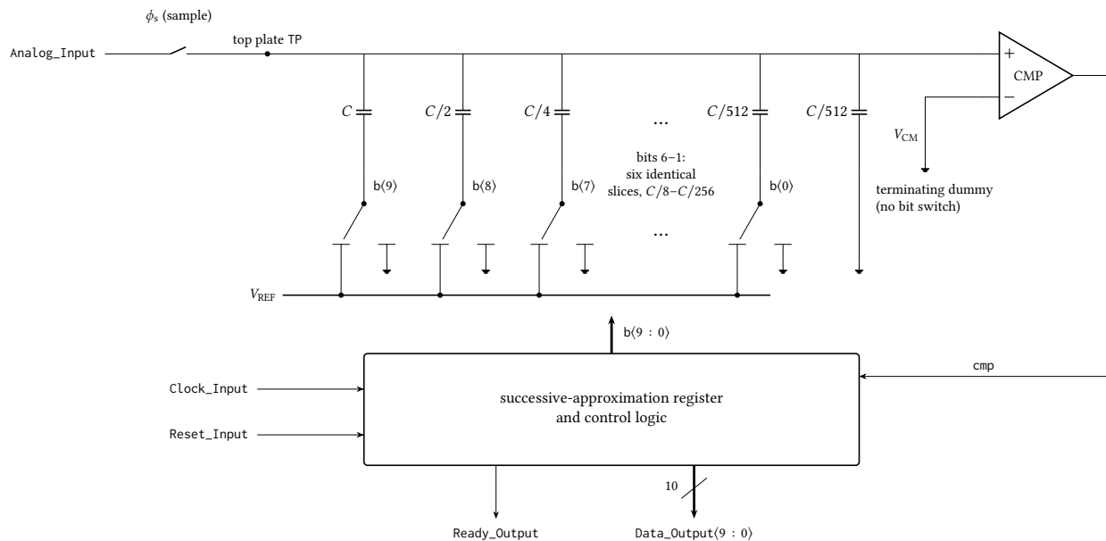
Figure 66: Generic single-ended charge-redistribution SAR ADC, drawn to explain the architecture of the 10-bit converter rather than to reproduce its implemented transistor-level schematic. The input is sampled through \phi_s onto the top plate of a binary-weighted array; the logic then switches each bottom plate from V_{REF} to ground one bit at a time, most significant first, and keeps or discards the trial from the comparator decision, so the conversion takes ten comparator cycles and the top plate converges to V_{CM} . Bits 6–1 are elided: six further slices identical to those drawn sit between C/4 and C/512 , and the terminating dummy C/512 carries no bit switch, which makes the total array 2C and the LSB weight C/512 . Only the external port names are those of the implemented block; the sampling network, comparator topology, clock generation and reset behaviour are representative, and no device dimensions are stated.
