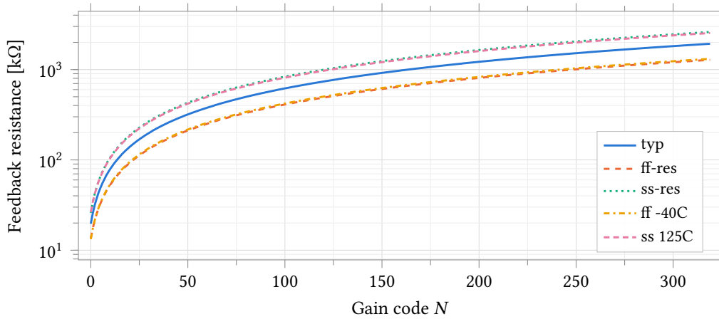
Figure 73: Measured resistance against gain code at all five corners, 500 nA forced through the A–B terminals with B held at V_{CM} = 1.25 V. The law is R = 18 \text{ k}\Omega + 6 \text{ k}\Omega \cdot N with N the binary value of ResEn<5:0> plus 64 per set ThEn<3:0> thermometer bit; every corner is strictly monotonic over all 320 codes, including the four thermometer seams. The corner families move the absolute value by -33 to +35 %, which is the poly sheet-resistance tolerance and must be absorbed by gain calibration, not by code choice.
