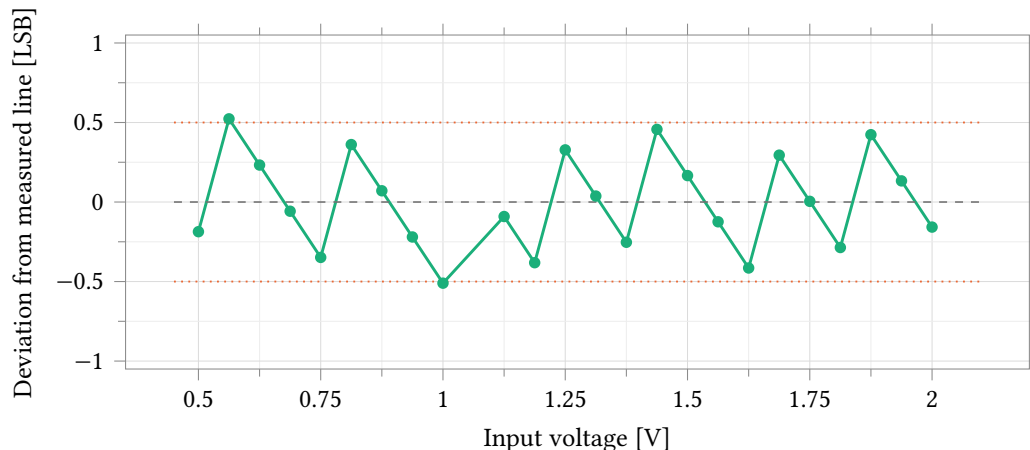
Figure 71: Deviation of each measured code from the converter's own best-fit line, 628.64 codes/V, over a 0.0625 V sweep of the unclipped window. Referred to its own scale rather than the nominal one the converter is straight to 0.523 LSB worst case and 0.294 LSB rms, so the 168 LSB of Figure 69 is gain error alone and carries no linearity information. The worst point sits just outside the \pm 0.5 LSB dotted guides. Twenty-four points 39 codes apart bound the deviation at the sampled inputs; a DNL or INL measurement needs every code and this grid does not provide one. A twenty-fifth point at 1.0625 V is absent because its simulation returned an error.
