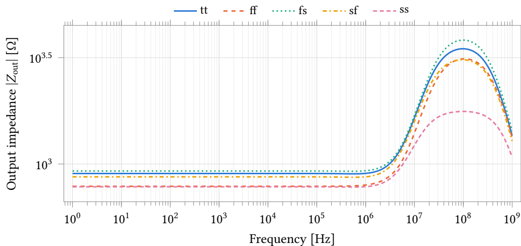
Figure 90: Magnitude of the supply block's output impedance against frequency over five process corners, 27 °C at point 1 and 25 °C at points 2–5. The AC load source carries unit magnitude, so |V_{DDDAC}| is the impedance in ohms. It is flat at 781 Ω to 927 Ω from 1 Hz to 100 kHz and peaks at 1.8 kΩ to 3.8 kΩ near 100 MHz. This is the small-signal impedance at zero load; the large-signal chord over the 0 μA to 100 μA sweep is 18 % to 51 % higher (Table 91).
