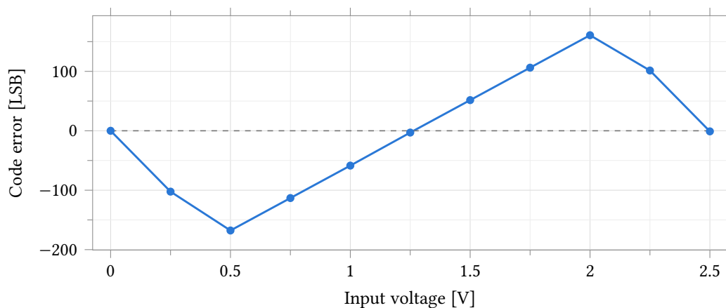
Figure 69: Code error against input voltage — measured code minus the ideal 409.6 codes/V line — from the same run as Figure 68. The error is the 1.535 slope ratio, not nonlinearity: it reaches -167.8 LSB at 0.5 V and 160.8 LSB at 2.0 V, crossing zero near the 1.25 V common mode where the measured and ideal lines intersect. It also returns near zero at 0 V and 2.5 V, where the clipped output coincides with the ideal endpoints; those two points are not accuracy. Referred to the fitted line instead, the residual over 0.5 V to 2.0 V is at most 0.52 LSB.
