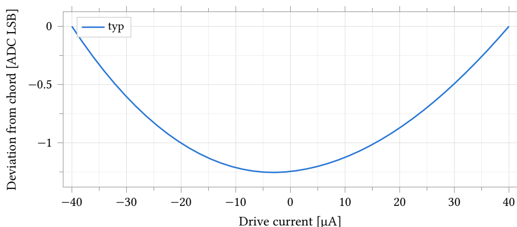
Figure 75: Drive nonlinearity of the bottom code ( N = 0 , R \approx 19.6 k \Omega ): voltage deviation from the endpoint chord over \pm 90 % of full scale ( \pm 40 \mu A), typical corner, expressed in 1.592 mV ADC LSB. All ten bypass gates are closed at this code and carry the full signal current; their on-resistance rises with the terminal's excursion from V_{CM} , so the chord — pinned at the sweep endpoints where that excursion is largest — overestimates the mid-range voltage by up to 1.25 LSB, and the deviation is bowl-shaped with a slight skew from the gates' voltage asymmetry. The same measurement at N = 63 and N = 319 , where the ladder dominates and current is 20–100 \times smaller, stays below 0.004 LSB and is tabulated, not plotted.
