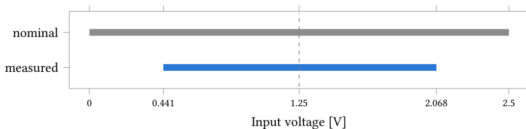
Figure 70: Usable input window of the converter against the nominal 0 V to 2.5 V supply span. The measured window runs 0.441 V to 2.068 V, 1.627 V wide, so 34.9 % of the nominal span is unreachable — 0.441 V at the bottom and 0.432 V at the top, near enough symmetric about the 1.25 V common mode (dashed). Outside that window the output sits at a code rail, so a transimpedance swing wider than \pm 0.81 V about V_{CM} is truncated rather than digitised.
