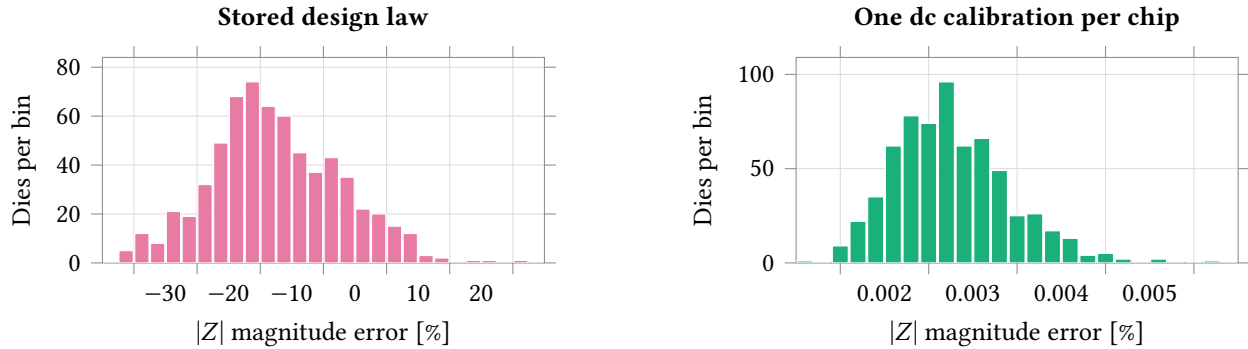
Figure 63: Impedance-magnitude error over 649 Monte Carlo dies at 0.1 Hz on the typical electrode at gain code 0, with process and mismatch together at the nominal corner and 37 °C, under two calibration policies: a stored 18 k \Omega + 6 k \Omega N design law (left) and one dc measurement of the feedback resistance per chip (right). \sigma falls from 10.24 % (95 % interval 9.71 to 10.83) to 0.000 65 % (0.000 61 to 0.000 68), a factor of 1.6 \times 10^4 , and the right panel is indistinguishable from measuring the current at every frequency — the bound, which needs a current reference the die does not carry. The two x -axes are independent and are not to be compared by eye: the left spans 70 % and the right 0.005 %, and both are the same 649 dies, load, gain code and run. The plotted range is that run’s own, -32.1 % to +30.6 %, and not a union over the campaign; no sample is censored. The statistical model section holds the capacitor family at typical, so the 22 pF feedback capacitor does not vary here and the figure bounds the feedback resistance rather than the pole — which matters because 0.1 Hz is below that pole, and above it a dc calibration stops working at all (Section 8.7.1).
