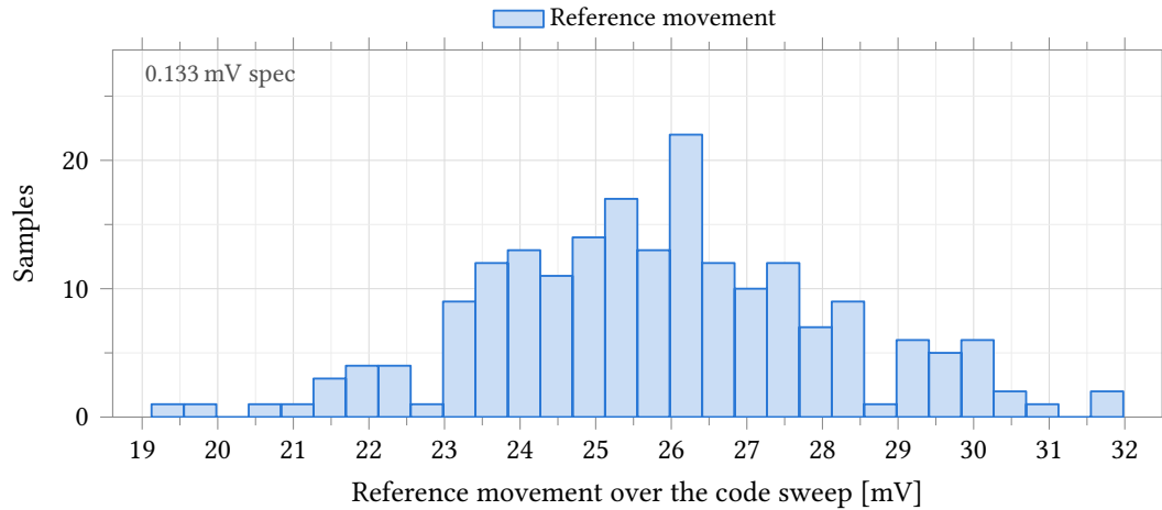
Figure 86: Peak-to-peak movement of the DAC reference V_{dd}DAC across the 4096-code sweep, with the ladder referenced to the on-chip supply block instead of an ideal rail. Process and mismatch , castalia_pm_25 , 200 samples, 25 °C, no external load on V_{dd}DAC . The quarter-LSB budget of 133 \mu V entered on the test sits about 200 times below the data, so it is annotated at the left axis edge rather than drawn and the distribution is not compressed into a single bar; the closest sample misses it by a factor of 144. Meeting it needs the supply's output impedance down by a factor of 193, to about 5 \Omega , against 894 \Omega small-signal (Table 96) and 1133 \Omega as a 0 \mu A to 100 \mu A chord (Table 92).
