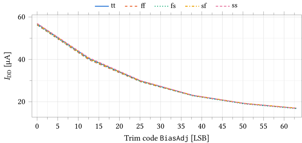
Figure 31: Trim characteristic: quiescent supply current against the BiasAdj word over all process corners, at the same six sampled codes. The current is strongly monotonic in the trim word, falling by a factor of about 3.4 from code 0 to code 63.
