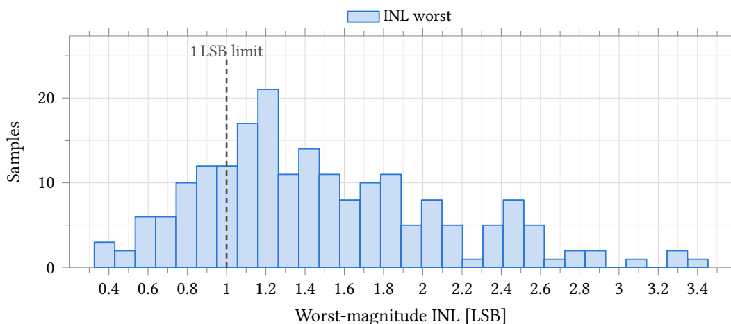
Figure 74: Integral nonlinearity of the R -2 R ladder driven from an ideal 2.5 V reference. Process and mismatch , model section castalia_pm_25 , 200 samples, seed 12345, low-discrepancy sampling, 25 °C, all 4096 codes. The dashed rule is the 1 LSB limit entered on the test; 42 of 200 samples fall inside it and the worst reaches 3.453 LSB. The distribution is right-skewed (Fisher skew +0.74), so Table 77 quotes the median and percentiles rather than \text{mean} \pm 3\sigma . LSB size, full scale and gain error are fixed to a part in 10^6 on this bench (Table 78), so the whole of this spread is resistor mismatch in the ladder and none of it is the reference.
