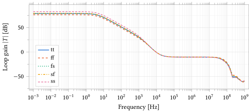
Figure 40: Transimpedance loop gain over five process corners, measured through a probe in series with the feedback network (Figure 38). R_f = 560 \text{ k}\Omega , C_f = 22 \text{ pF} , C_L = 5 \text{ pF} , C_c = 500 \text{ fF} , BiasAdj = 37, 2.5 V, Randles electrode with R_s = 100 \text{ }\Omega , R_{ct} = 1 \text{ M}\Omega , C_{dl} = 100 \text{ nF} . tt is at 37^\circ\text{C} , the four skew corners at 25^\circ\text{C} . This is the loop around the amplifier, the feedback network and the electrode together, not the amplifier's own gain; the two are tabulated separately in Table 37 and Table 24.
