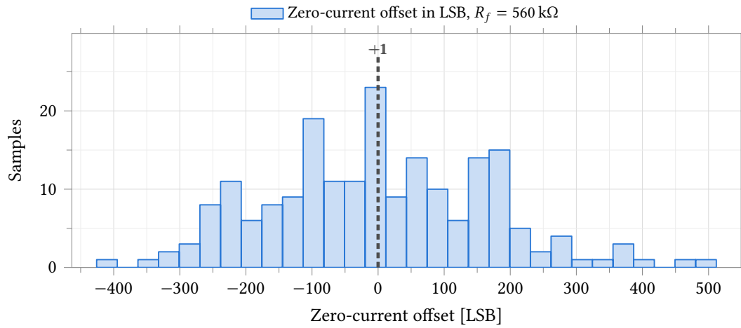
Figure 55: Zero-current output offset at R_f = 560\text{ k}\Omega , conditions as Figure 54 but at R_{ct} = 10\text{ k}\Omega (the same stiff electrode as the finite-loop-gain demonstration of Table 54, NOT the 1\text{ M}\Omega operational electrode of Table 53). Some samples reach the sweep’s output rails (Table 63); the LSB spread here is 14\times wider than at 35\text{ k}\Omega for the same underlying current offset, since the same offset current is multiplied through a 16\times larger R_f .
