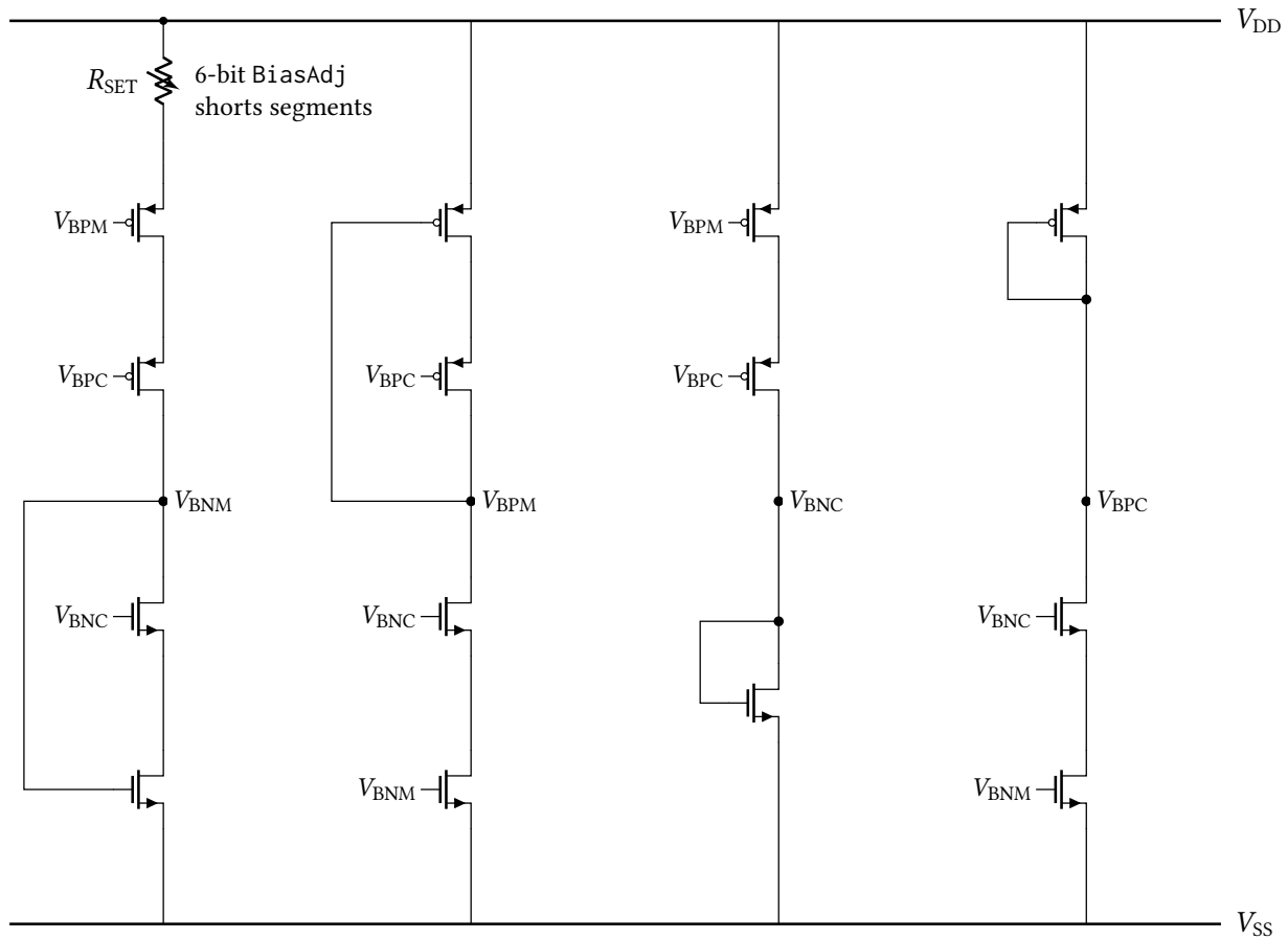
Figure 23: Simplified core of the local wide-swing cascode bias generator, drawn from the anatop_biasgen_local schematic. Four self-biased branches develop the four rails: the reference branch (left) passes the current set by the trimmable resistor R_{\text{SET}} , and the remaining branches mirror it to produce V_{\text{BPM}} , V_{\text{BNC}} and V_{\text{BPC}} . Each branch's own self-bias (diode) connection is drawn, from the rail it generates back to the gate it drives in the same branch; the cross-branch gate connections are identified by net name rather than drawn as buses. The enable switches, the decoupling capacitors on each rail and the individual segments of the resistor string are omitted for clarity.
