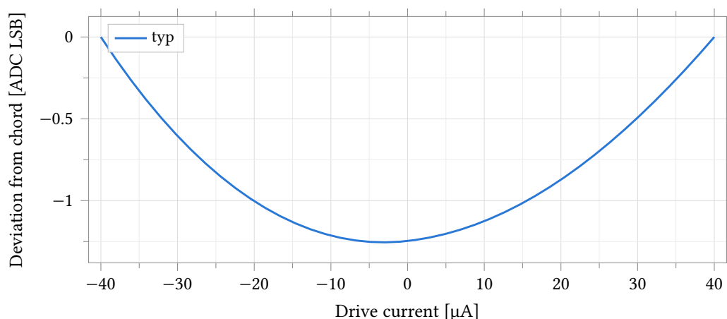
Figure 65: Drive nonlinearity of the bottom code ( N = 0 , R \approx 19.6 k \Omega ): voltage deviation from the endpoint chord over \pm 90 % of full scale ( \pm 40 \mu A), typical corner, expressed in 1.592 mV ADC LSB. All ten bypass gates are closed at this code and carry the full signal current; their on-resistance rises with the terminal's excursion from V_{CM} , so the chord — pinned at the sweep endpoints where that excursion is largest — overestimates the mid-range voltage by up to 1.25 LSB, and the deviation is bowl-shaped with a slight skew from the gates' voltage asymmetry. The same measurement at N = 63 and N = 319 , where the ladder dominates and current is 20–100 \times smaller, stays below 0.004 LSB and is tabulated, not plotted.
