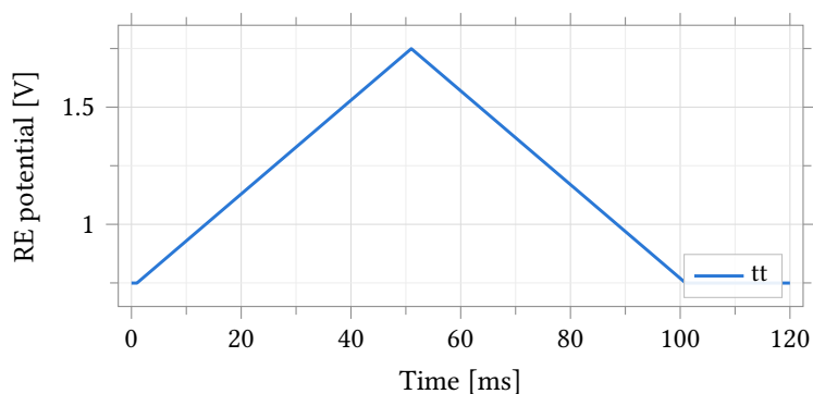
Figure 52: Commanded reference-electrode potential against time for the triangular voltammetry sweep, typical process point, 37^{\circ}\text{C} , R_f = 35\text{ k}\Omega , R_{ct} = 1\text{ M}\Omega electrode. Paired with the current response of Figure 51.
