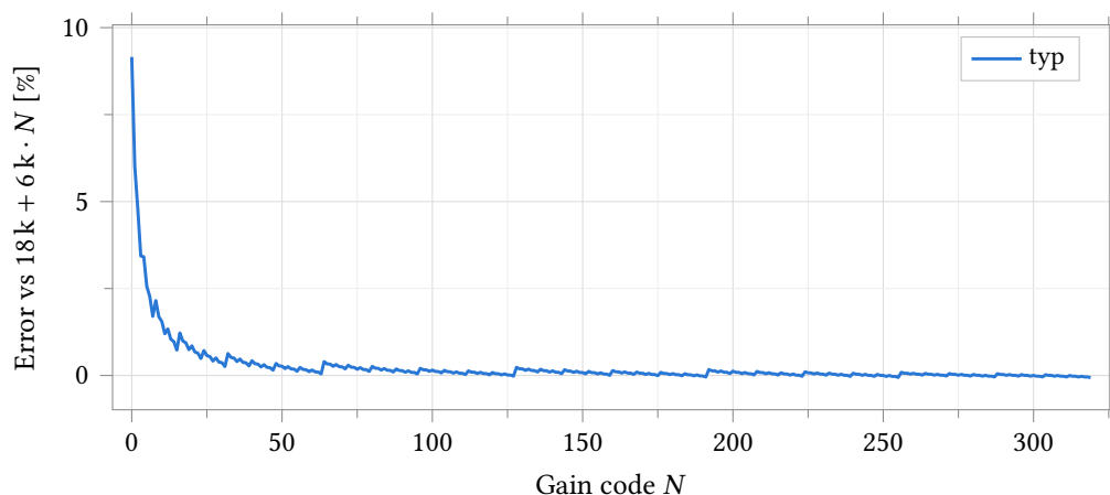
Figure 64: Typical-corner deviation from the ideal code law. The +9.2 % at N = 0 is the series resistance of the ten closed bypass switches (1.65 k \Omega , about 165 \Omega each), which decays as 1/R once real ladder segments dominate; by N = 319 the error is -0.063 %. The ripple is the carry structure: at each binary carry and at each thermometer seam the set of closed switches changes, so the R_{on} term steps while the ladder term is exact.
