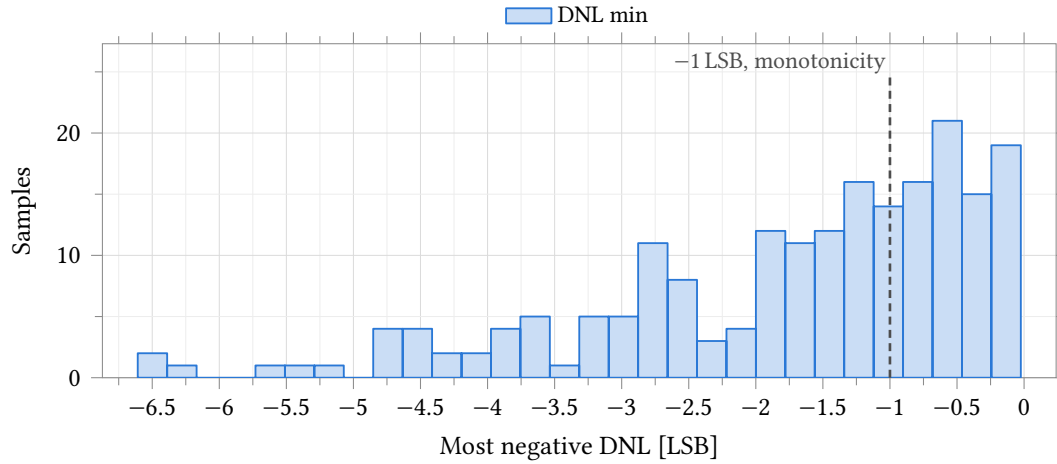
Figure 75: Worst negative differential nonlinearity, same bench, samples and conditions as Figure 74. The dashed rule at -1 LSB is the monotonicity limit entered on the test: 80 of 200 samples clear it, so 40 % of channels are monotonic and 0.40^4 = 2.6 % of four-channel chips are monotonic on all four. The distribution is left-skewed (skew -1.11 ) with a tail to -6.608 LSB, so the median -1.318 LSB and the percentiles of Table 77 describe it and mean \pm 3\sigma does not.
