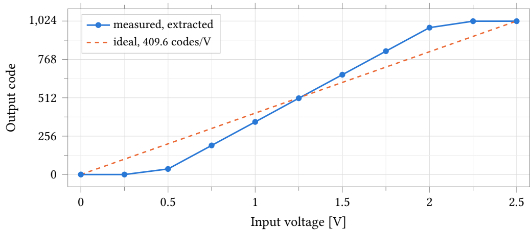
Figure 58: Output code against input voltage for the extracted anatop_pixel_adc , nominal corner, 37 °C, 2.5 V analog and 1.0 V digital supplies, with the ideal 409.6 codes/V line overlaid. The transfer is monotonic and reaches both code limits, but its slope is 628.64 codes/V – 1.535 times ideal – so the flat segments below 0.44 V and above 2.07 V are the code limits, not the ends of the sweep. Markers are the eleven simulated points; the 0.25 V step is 157 codes, so the curve between them is interpolation and carries no linearity information.
