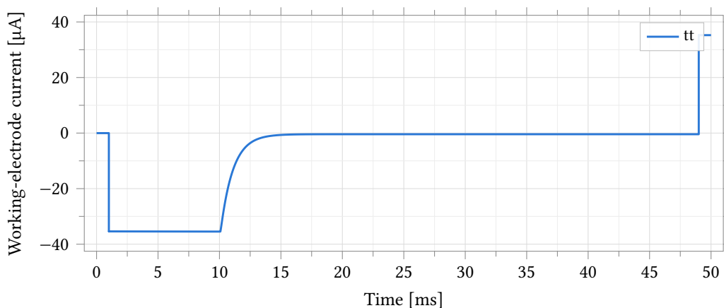
Figure 53: Step response of the working-electrode current to a 400 mV step in the commanded reference potential, typical process point, 37^{\circ}\text{C} , R_f = 35\text{ k}\Omega , R_{ct} = 1\text{ M}\Omega electrode, 1\text{ }\mu\text{s} edge. The transient overshoots and briefly rails against the loop's slew-limited edges immediately after the step – by design, the bench exercises the edge rather than a settled operating condition – before settling to the value set by the cell impedance.
