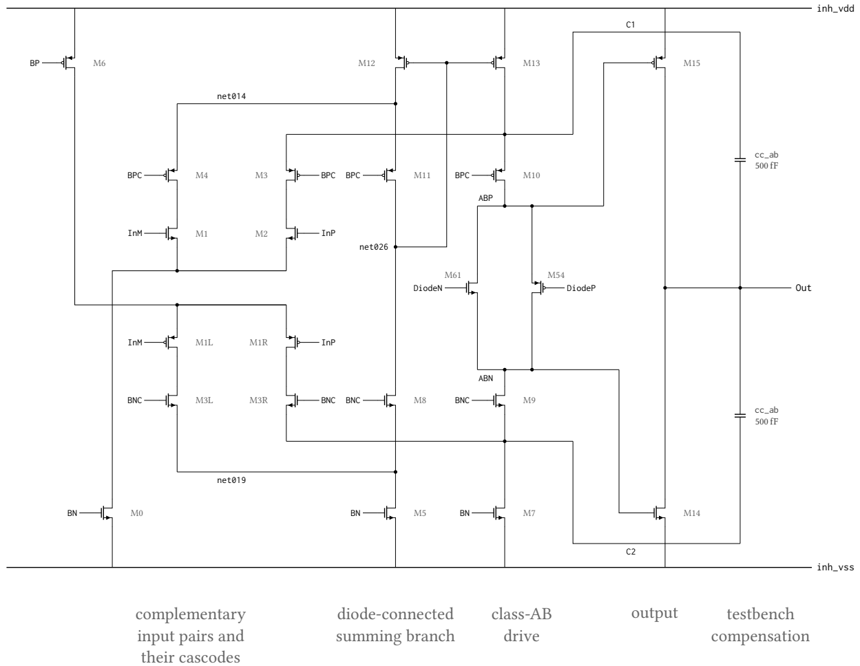
Figure 34: Signal-path topology of the class-AB amplifier anatop_tia_amp_ab , drawn from its netlist. The complementary pairs M1 / M2 (NMOS, tail M0 ) and M1L / M1R (PMOS, tail M6 ) fold into two cascode branches; the InM side terminates in the diode-connected branch M12 – M11 – M8 – M5 , whose summing node net026 sets M13 , which restates that current into the InP branch, and the floating pair M54 / M61 holds ABP above ABN so both output devices M15 and M14 are actively driven. C1 and C2 are the common source nodes of the PMOS cascodes M10 / M3 and of the NMOS cascodes M9 / M3R , brought out as pins; the two cc_ab capacitors that return them to Out are testbench components outside the cell, 500 fF per side. Simplified: the enable switch and its four power-down devices, and the bias generator that develops DiodeN / DiodeP , are omitted, so 22 of the cell’s 34 transistors are drawn; BP / BPC / BN / BNC are the enabled forms of the bp !/bpc!/bn!/bnc! globals and device dimensions are not shown. Identically labelled nets are connected; wires crossing without a filled dot are not.
