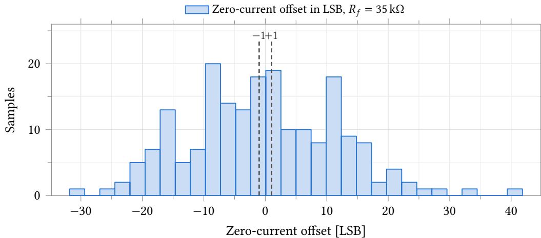
Figure 54: Zero-current output offset at R_f = 35\ \text{k}\Omega , referred to the 2.441\ \text{mV} ADC LSB. Mismatch only , 25^\circ\text{C} nominal process, 200 samples, R_{\text{ct}} = 10\ \text{k}\Omega electrode. The limit shown is the \pm 1\ \text{LSB} entered on the test in Assembler – comparable in kind across the four gain taps but mechanically harder to meet as R_f rises, since the underlying offset is closer to gain-independent in current (Table 63). Statistics are in Table 63.
