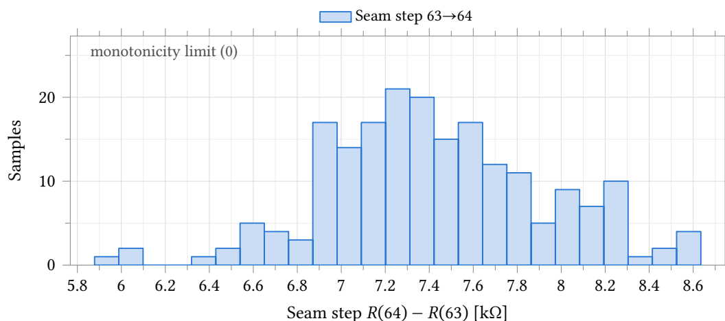
Figure 66: Per-sample step across the first thermometer seam (code 63 to 64: one 64-unit segment switches in while all six binary segments switch out), the code transition most exposed to mismatch. Mismatch only , model section castalia_pm_25 , nominal process, 200 samples, seed 12345, low-discrepancy sampling, 25 °C. Mean 7.42 k \Omega , \sigma = 504 \Omega , worst sample 5.88 k \Omega – 14.7\sigma above the monotonicity limit at zero, so no realistic mismatch closes the seam.
