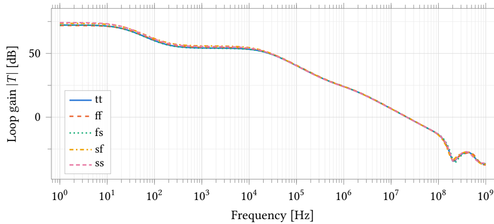
Figure 50: Potentiostat control-loop gain over five process corners, measured through the 0 V probe IPRB1 in the RE feedback path (Figure 47). R_f = 35 \text{ k}\Omega , cell R_{\text{ce}} = R_u = 1 \text{ k}\Omega , R_{\text{ct}} = 10 \text{ k}\Omega , C_{\text{dl}} = 100 \text{ nF} , 2.5 V supply. This is the full loop – A1, A2, both feedback networks and the electrode together – and is not the open-loop amplifier gain of Section 8.4. tt is at 37 °C, the four skew corners at 25 °C.
