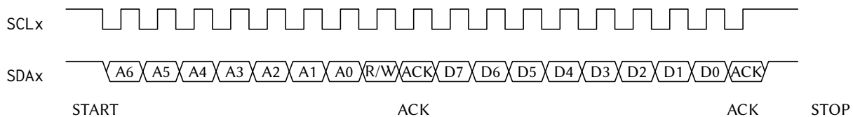
Figure 96: One I2C byte write on the wire: START, the 7-bit address and direction bit, the addressed device's ACK, one data byte, its ACK, then STOP. START and STOP are the two transitions of SDAx that occur while SCLx is high; every data bit is stable across the SCLx high period.
