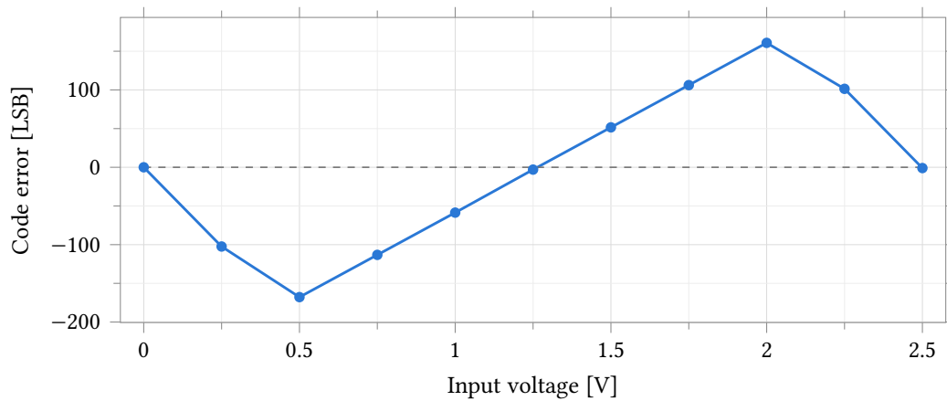
Figure 59: Code error against input voltage — measured code minus the ideal 409.6 codes/V line — from the same run as Figure 58. The error is the 1.535 slope ratio, not nonlinearity: it reaches -167.8 LSB at 0.5 V and 160.8 LSB at 2.0 V, crossing zero near the 1.25 V common mode where the measured and ideal lines intersect. It also returns near zero at 0 V and 2.5 V, where the clipped output coincides with the ideal endpoints; those two points are not accuracy. Referred to the fitted line instead, the residual over 0.5 V to 2.0 V is at most 0.52 LSB.
