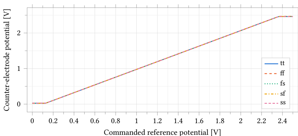
Figure 45: Counter-electrode potential against commanded reference potential over five process corners, cell-drive bench (Figure 44). The amplifier drives a Randles cell with R_{CE} = 1\text{ k}\Omega , R_u = 1\text{ k}\Omega , R_{ct} = 10\text{ k}\Omega , C_{dl} = 1\text{ }\mu\text{F} with the working electrode held at 1.25 V, C_L = 5\text{ pF} , C_c = 500\text{ fF} , 2.5 V supply; the typical point is at 37 °C and the four skew corners at 25 °C. The central segment rises with slope 12/11, the divider between the 1 k \Omega counter-electrode branch and the 11 k \Omega remainder of the cell; the flat ends are the amplifier against its rails, and their heights are the compliance limits tabulated in Table 46. Over the whole central segment the cell current is set by the cell resistance and the commanded potential, not by the amplifier.
