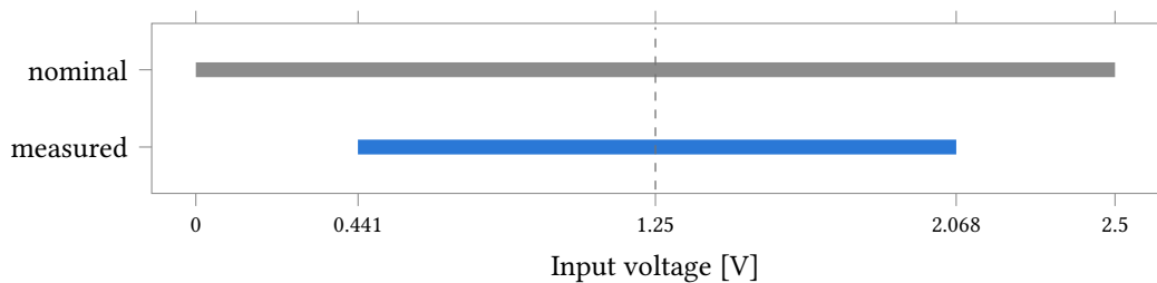
Figure 60: Usable input window of the converter against the nominal 0 V to 2.5 V supply span. The measured window runs 0.441 V to 2.068 V, 1.627 V wide, so 34.9 % of the nominal span is unreachable — 0.441 V at the bottom and 0.432 V at the top, near enough symmetric about the 1.25 V common mode (dashed). Outside that window the output sits at a code rail, so a transimpedance swing wider than \pm 0.81 V about V_{CM} is truncated rather than digitised.
