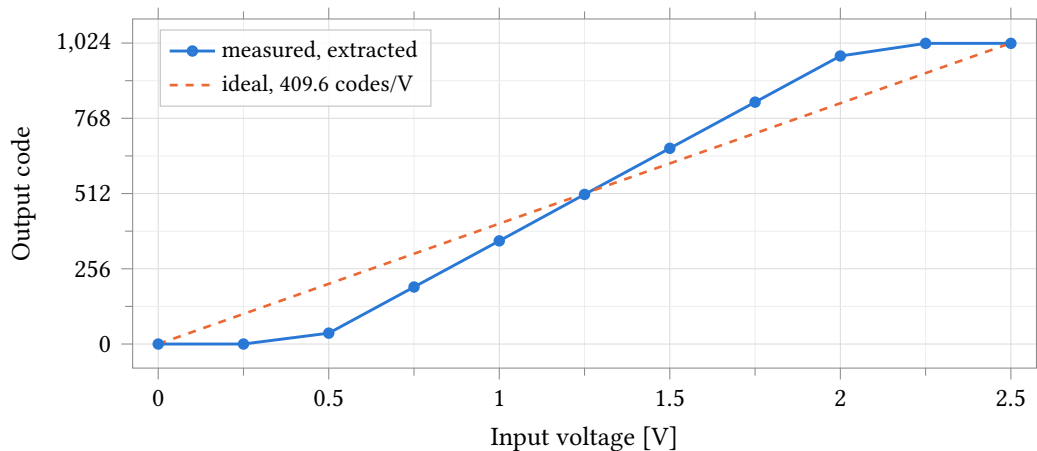
Figure 60: Output code against input voltage for the extracted anatop_pixel_adc, nominal corner, 37 °C, 2.5 V analog and 1.0 V digital supplies, with the ideal 409.6 codes/V line overlaid. The transfer is monotonic and reaches both code limits, but its slope is 628.64 codes/V — 1.535 times ideal — so the flat segments below 0.44 V and above 2.07 V are the code limits, not the ends of the sweep. Markers are the eleven simulated points; the 0.25 V step is 157 codes, so the curve between them is interpolation and carries no linearity information.
