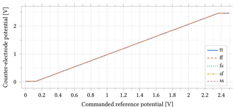
Figure 47: Counter-electrode potential against commanded reference potential over five process corners, cell-drive bench (Figure 46). The amplifier drives a Randles cell with R_{CE} = 1 \text{ k}\Omega , R_u = 1 \text{ k}\Omega , R_{ct} = 10 \text{ k}\Omega , C_{dl} = 1 \mu\text{F} with the working electrode held at 1.25 V, C_L = 5 \text{ pF} , C_c = 500 \text{ fF} , 2.5 V supply; the typical point is at 37 °C and the four skew corners at 25 °C. The central segment rises with slope 12/11, the divider between the 1 k \Omega counter-electrode branch and the 11 k \Omega remainder of the cell; the flat ends are the amplifier against its rails, and their heights are the compliance limits tabulated in Table 47. Over the whole central segment the cell current is set by the cell resistance and the commanded potential, not by the amplifier.
