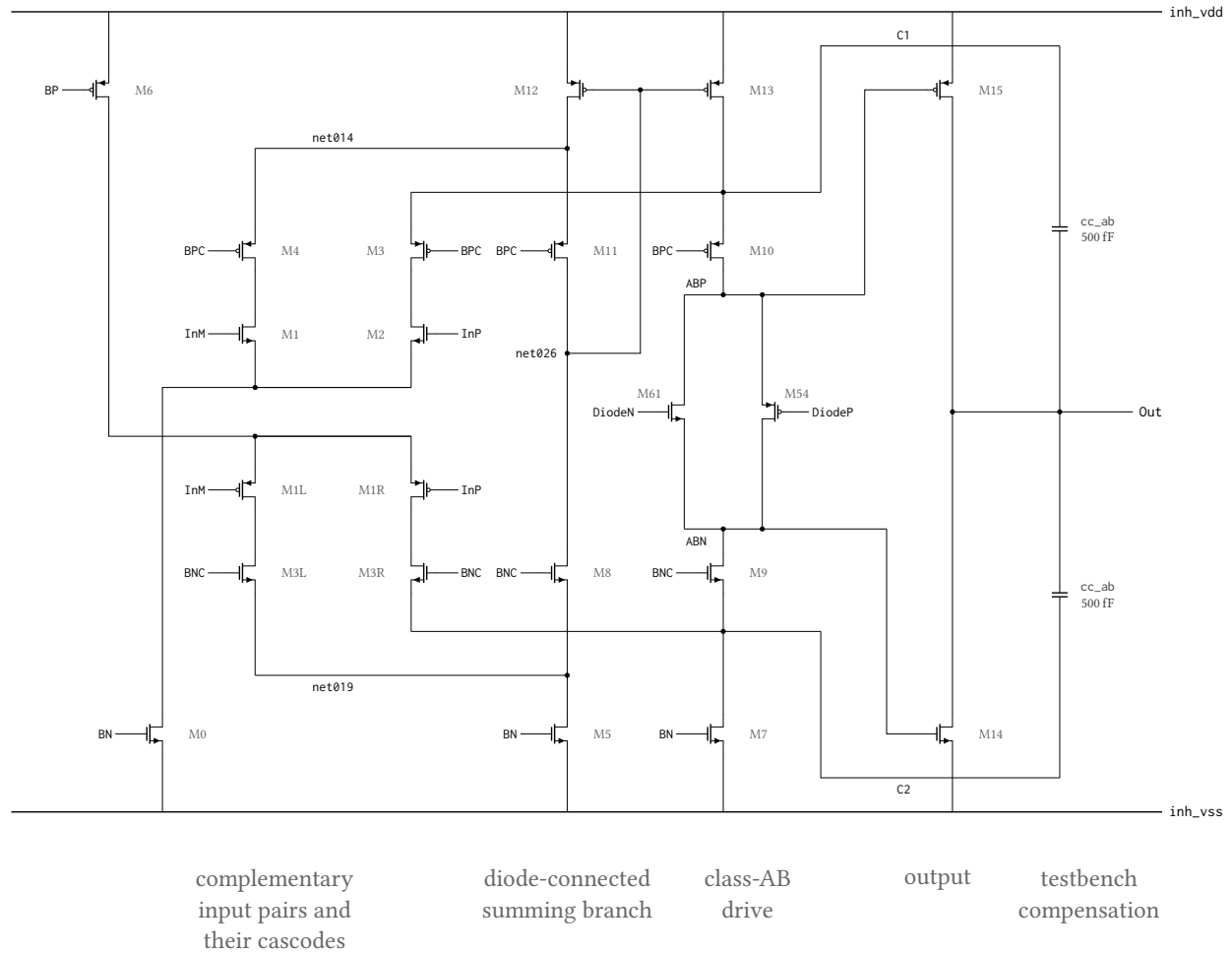
Figure 36: Signal-path topology of the class-AB amplifier anatop_tia_amp_ab, drawn from its netlist. The complementary pairs M1/M2 (NMOS, tail M0) and M1L/M1R (PMOS, tail M6) fold into two cascode branches; the InM side terminates in the diode-connected branch M12–M11–M8–M5, whose summing node net026 sets M13, which restates that current into the InP branch, and the floating pair M54/M61 holds ABP above ABN so both output devices M15 and M14 are actively driven. C1 and C2 are the common source nodes of the PMOS cascodes M10/M3 and of the NMOS cascodes M9/M3R, brought out as pins; the two cc_ab capacitors that return them to Out are testbench components outside the cell, 500 fF per side. Simplified: the enable switch and its four power-down devices, and the bias generator that develops DiodeN/DiodeP, are omitted, so 22 of the cell’s 34 transistors are drawn; BP/BPC/BN/BNC are the enabled forms of the bp!/bpc!/bn!/bnc! globals and device dimensions are not shown. Identically labelled nets are connected; wires crossing without a filled dot are not.
