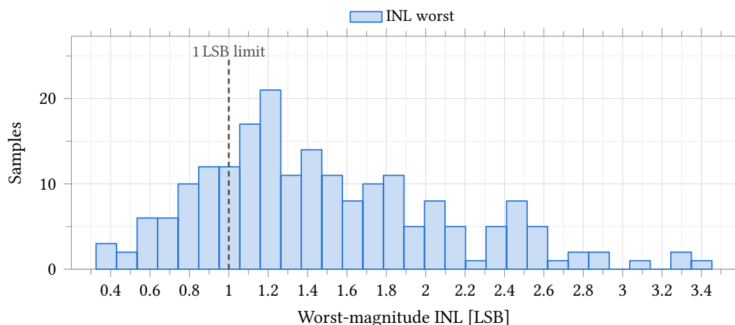
Figure 76: Integral nonlinearity of the R - 2R ladder driven from an ideal 2.5 \text{ V} reference. Process and mismatch , model section castalia_pm_25 , 200 samples, seed 12345, low-discrepancy sampling, 25^\circ\text{C} , all 4096 codes. The dashed rule is the 1 LSB limit entered on the test; 42 of 200 samples fall inside it and the worst reaches 3.453 LSB. The distribution is right-skewed (Fisher skew +0.74 ), so Table 82 quotes the median and percentiles rather than \text{mean} \pm 3\sigma . LSB size, full scale and gain error are fixed to a part in 10^6 on this bench (Table 83), so the whole of this spread is resistor mismatch in the ladder and none of it is the reference.
