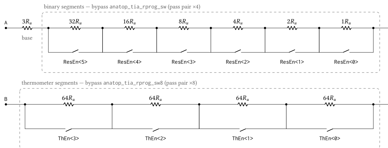
Figure 64: Segment and bypass-switch structure of anatop_tia_rprog, transcribed from the executed spec-run netlist. The unit R_u is one series poly resistor; from terminal A the chain runs through the never-switched three-unit base, the six binary-weighted segments of 32 down to 1 unit, and the four identical 64-unit thermometer segments to terminal B. Each switched segment is shunted by a CMOS transmission gate with a local inverter: the control pin EnBar is the ResEn/ThEn bit itself and drives the PMOS pass gate directly and the NMOS pass gate through the inverter, so a bit at 1 turns both pass devices off and inserts the segment. The pass pair has multiplicity 4 in the binary switch ( _sw ) and 8 in the thermometer switch ( _sw8 ), which halves the thermometer gates' on-resistance where up to six binary gates close at a seam. Three grounded dummy units accompany the 322 active units for matching.
