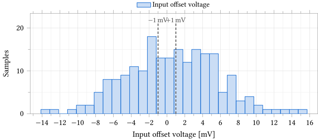
Figure 38: Input offset voltage of the amplifier. Process and mismatch , 37 °C, 200 samples, 2.5 V supply, C_L = 5 \text{ pF} , C_c = 500 \text{ fF} , a 5 pF load, differential input swept about mid-supply. The distribution is symmetric about 0.58 mV, so the systematic term of Table 26 is small against the random one, and the \pm 1 \text{ mV} rules are the limits entered on the test; 24 of 200 samples fall inside them. Statistics are in Table 29.
