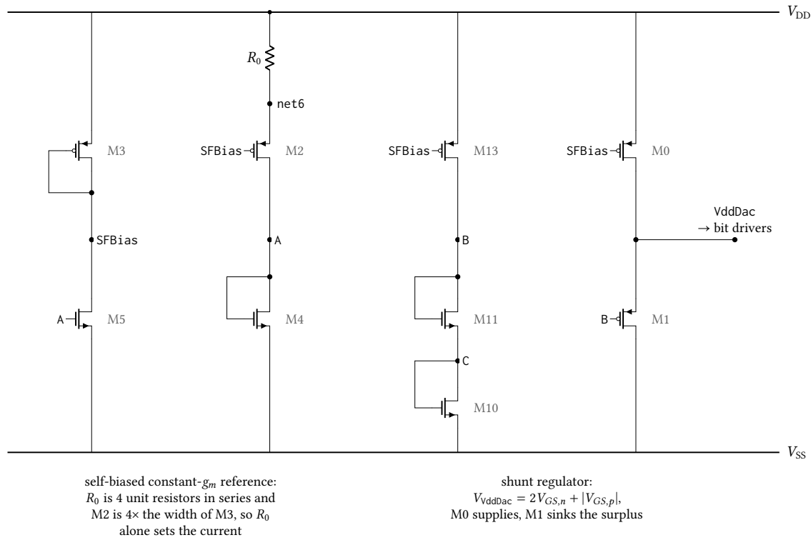
Figure 72: Core of atop_pixel_dac_psu , the shunt regulator that generates the V_{ddDac} rail the ladder uses as its reference, transcribed from the LoadRegTB netlist. The self-biased constant- g_m reference on the left sets SFBias ; M_{13} drives that current through the stacked diodes M_{11} and M_{10} to hold B two gate-source voltages above V_{SS} , and M_1 sinks whatever of M_0 's current the ladder leaves, clamping V_{ddDac} one PMOS gate-source voltage above B : 2.177 V unloaded from a 2.5 V rail. There is no error amplifier, so load regulation is set by M_1 's g_m alone. The five start-up and enable devices — the weak pull-up and its two kick devices on SU , the shutdown pull-up on SFBias and the En inverter — are omitted; none carries current once the loop is running. Device dimensions are proprietary and are not stated.
