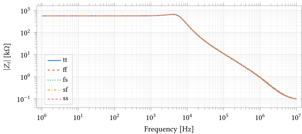
Figure 45: Closed-loop transimpedance magnitude over five process corners, conditions as Figure 43. Peaking 1.2 dB to 1.5 dB at 3.98 kHz; -3 \text{ dB} bandwidth 7.2 kHz to 7.5 kHz. At C_f = 5 \text{ pF} the same conditions give 3.0 dB to 3.7 dB of peaking and 41.7^\circ to 46.4^\circ of phase margin.
