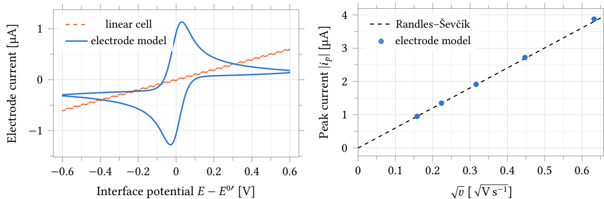
Figure 24.3: Standalone validation of the electrode model against closed-form voltammetry, ideal potential source, model defaults of Table 24.2 with R_s = 500 \Omega and C_{dl} = 0.2 \mu F in series and in parallel respectively, 25^\circ C . Left: current against interface potential over a \pm 0.6 V triangular sweep at 50 mV s^{-1} , second cycle, for the nonlinear model (solid) and for the linear cell of Section 24.1 driven identically (dashed, R_{ct} = 1 M\Omega ); the linear response is a ramp with its extrema pinned at the switching potentials (its C_{dl} box is only 20 nA wide at this scan rate and invisible here), while the nonlinear one peaks 30 mV either side of E^{0'} and decays afterwards. Right: peak cathodic current of the first scan against \sqrt{v} over 25 mV s^{-1} to 400 mV s^{-1} , against the Randles–Ševčík line, of slope 6.015 \mu A per \sqrt{V s^{-1}} ; the two panels use different cycles because Randles–Ševčík describes the first scan into an undepleted bulk, while the second cycle is the repeatable steady response and sits 3 % to 5 % below it. Numbers in Table 24.3.
