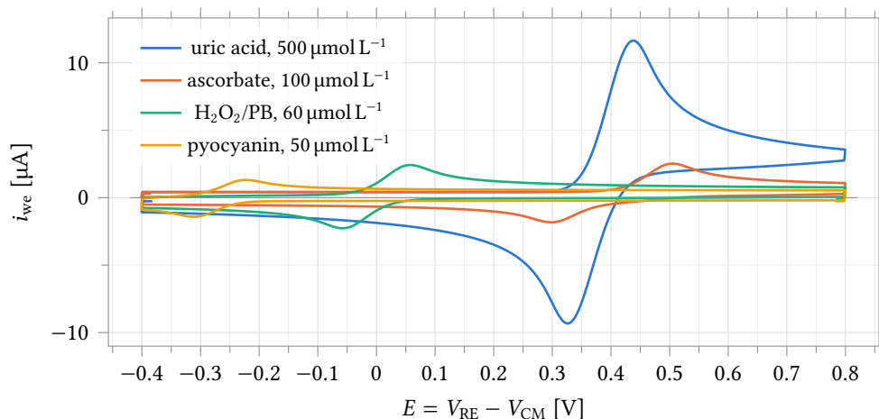
Figure 24.4: Voltammograms of the four-analyte wound panel through the rev-2 channel, one electrode parameter set per channel, from the cyclic-voltammetry Maestro corner run of Section 24.2 (2 V s -1 , R_f = 35 kΩ, conditions of the in-loop run above). Peak potential identifies the analyte and peak height its concentration; each trace is one full cycle started at that analyte’s non-faradaic vertex. E^{0'} and concentrations are literature-anchored; k^0 is fitted (no measured value exists on carbon for any of the four), and reversal peaks appear for the chemically irreversible couples because following chemistry is not modelled. The two cathodic markers span -1.4 μA to -2.4 μA, unmeasurable by the unidirectional rev-1 front end.
