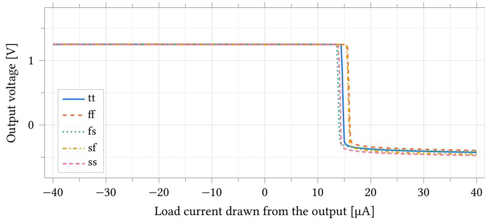
Figure 28: Output voltage as a DC load current is drawn from the output, over the five corners. Positive current is drawn out of the node, so the amplifier must source it; the collapse at 13.6 \mu\text{A} to 15.6 \mu\text{A} is the class-A stage running out of the fixed current in M5. Sinking holds within 0.8 mV of v_{cm} to the -40 \mu\text{A} sweep limit, so that direction is bounded, not measured.
