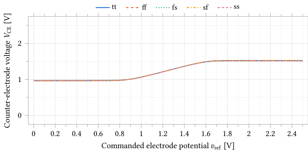
Figure 19: Counter-electrode voltage over the same sweep, against the full supply range. V_{\text{CE}} stops about 1 V short of each rail because the amplifier reaches its current limit before its voltage limit, so the drive shortfall in Table 14 is a current-budget problem rather than a compliance one.
