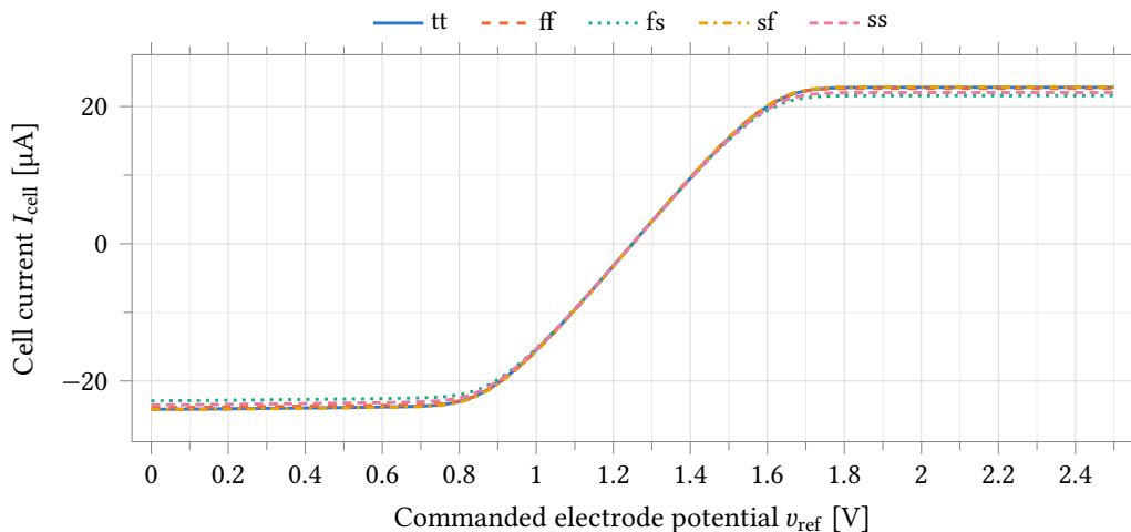
Figure 18: Cell current against commanded electrode potential, over the five process corners. The amplifier drives the counter electrode of a Randles cell ( 1\text{ k}\Omega CE–RE, 1\text{ k}\Omega RE–WE, 10\text{ k}\Omega charge transfer, 1\text{ }\mu\text{F} double layer) with the working electrode held at v_{\text{cm}} . The flat ends are the output current limit, and it is closely symmetric in both directions.
