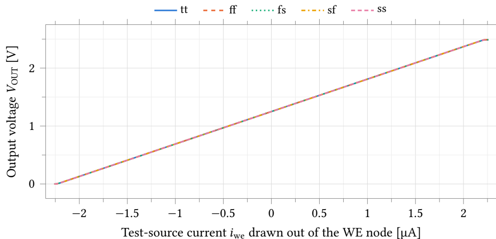
Figure 32: Output voltage against the swept test-source current over the five corners, at R_f = 560 \text{ k}\Omega with the electrode held at v_{cm} = 1.25 \text{ V} . The bench source draws current out of the WE node, so i_{we} = -I_{WE} against Equation (1) and the slope is +R_f . The corners overlay to the line width because that slope is the feedback resistor, ideal in this bench.
