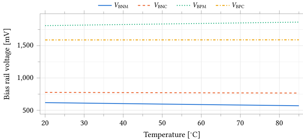
Figure 8: The four local bias rails against temperature at the typical corner. V_{\text{BNM}} and V_{\text{BNC}} are referred to v_{\text{ss}} ; V_{\text{BPM}} and V_{\text{BPC}} sit near the supply.
