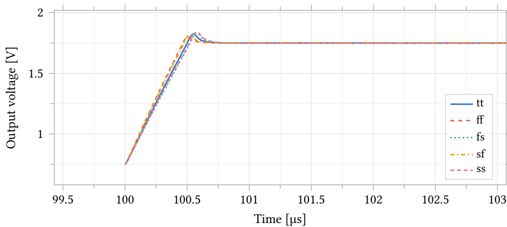
Figure 30: Rising edge of a 1 V step ( v_{cm} \pm 0.5 V) in unity feedback into 5 pF, over the five corners; the window is 3.5 \mu s around the edge at 100 \mu s, and the falling edge at 1.1 ms lies outside it. The output slews for about 0.4 \mu s, overshoots once by 5.0 % to 9.0 % of the step and recovers without ringing — slew recovery, not small-signal ringing, as the 88° phase margin predicts.
