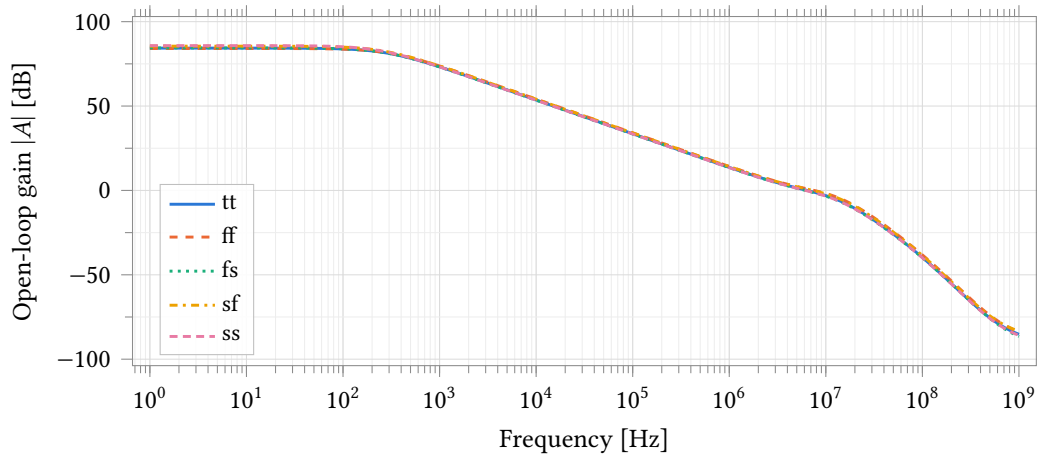
Figure 26: Open-loop gain over the five process corners, by stb through the feedback probe with the amplifier in unity feedback and a 5 pF load. Miller compensation gives a single-pole roll-off from 290 Hz to a 6.2 MHz to 7.6 MHz crossover. This is the amplifier alone; the loop that closes around the electrode is not this well behaved (Figure 31).
