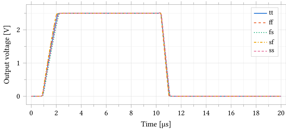
Figure 29: Open-loop large-signal response to a rail-to-rail input pulse into 5 pF, over the five corners. The falling edge is 1.7 times faster because the second stage is class A: M12 is a driven device, M5 a fixed current source.
