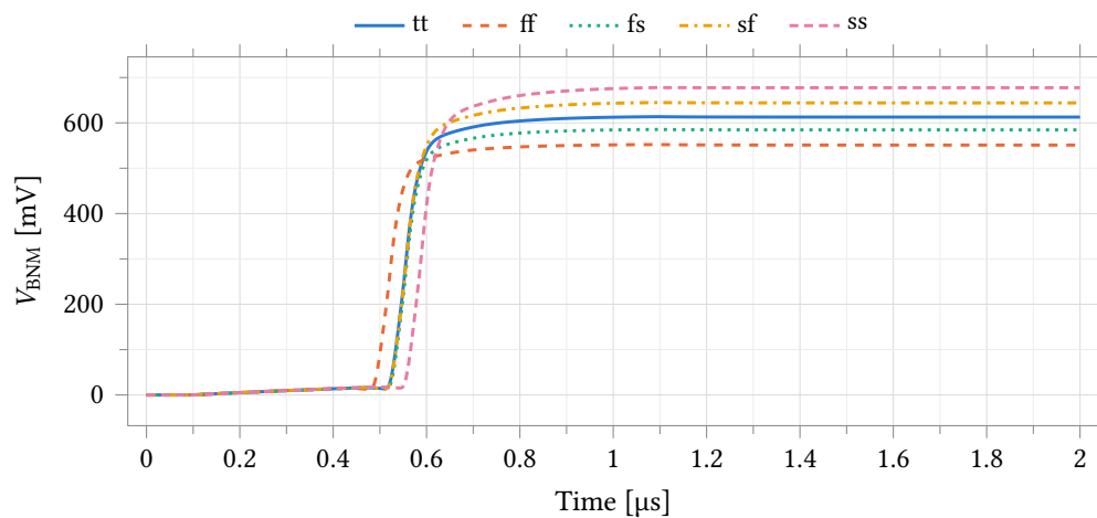
Figure 16: Power-up settling of V_{BNM} over all process corners.
