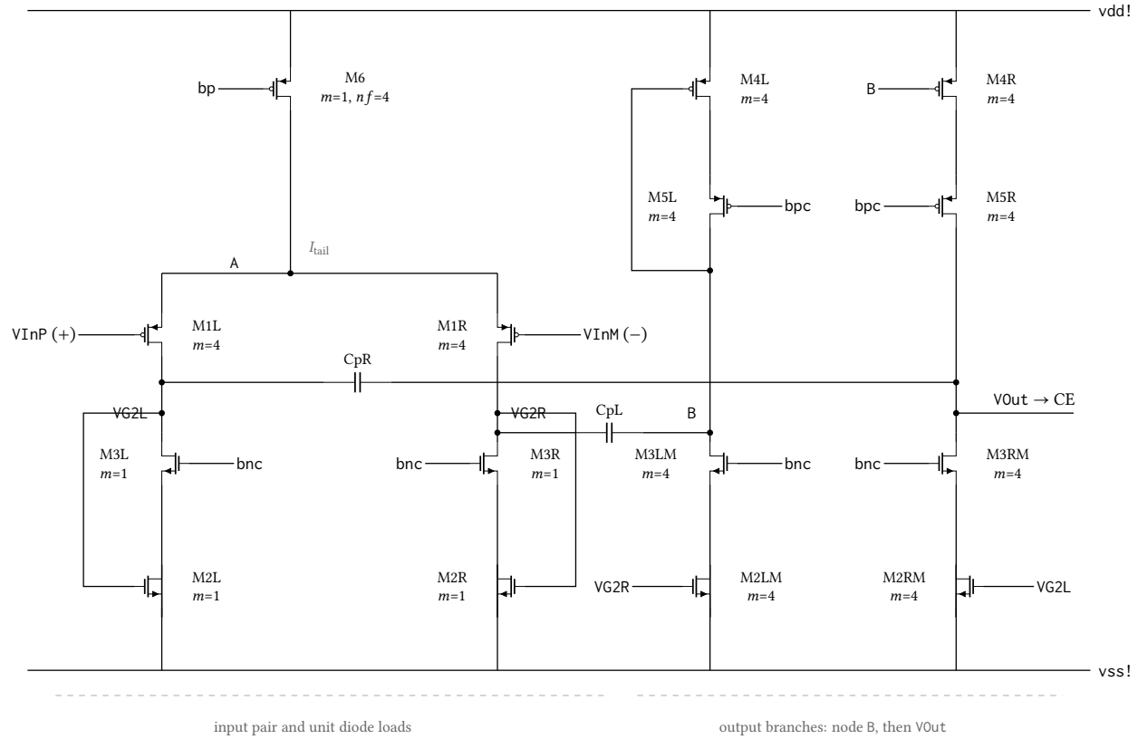
Figure 17: Control amplifier core: a symmetric current-mirror (mirrored) OTA with a PMOS input pair, drawn in the same arrangement as the Virtuoso cellview — input pair and its two unit diode loads on the left, the two output branches on the right. Each input device steers part of I_{tail} into a unit diode ( m=1 ); a mirror four times larger then restates it, the extttVG2L half directly onto extttVOut and the extttVG2R half into node extttB, where the PMOS mirror inverts it and returns it to extttVOut so the two halves add. Both output devices are cascoded. extttCpL and extttCpR damp the mirror poles. Identically labelled nets are connected; matching dummies are omitted.
