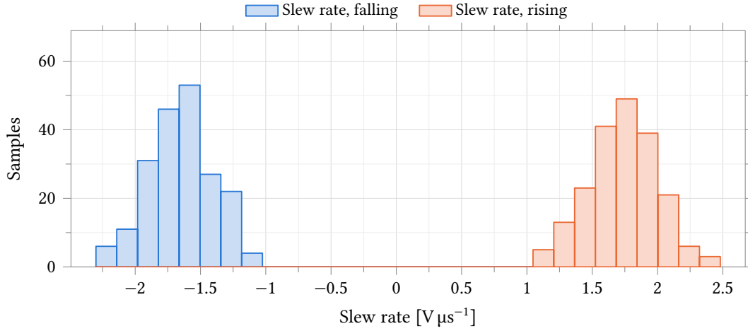
Figure 24: Slew rate on both edges of a 1 V step into 10 pF. Rising and falling averages are 1.74 \text{ V } \mu\text{s}^{-1} and 1.65 \text{ V } \mu\text{s}^{-1} , a 5 % imbalance: the tail current is steered into one input device and mirrored to the output, so the slewing current is equal in both directions by construction.
