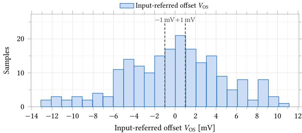
Figure 22: Input-referred offset, mismatch only (castalia_mm_25, process fixed at typical). The distribution is Gaussian with \sigma = 4.82 mV against a \sigma \leq 2 mV budget; 37 of 200 samples fall inside the \pm 1 mV rules shown. Offset lands directly on the commanded electrode potential and is the dominant accuracy term at low cell current.
