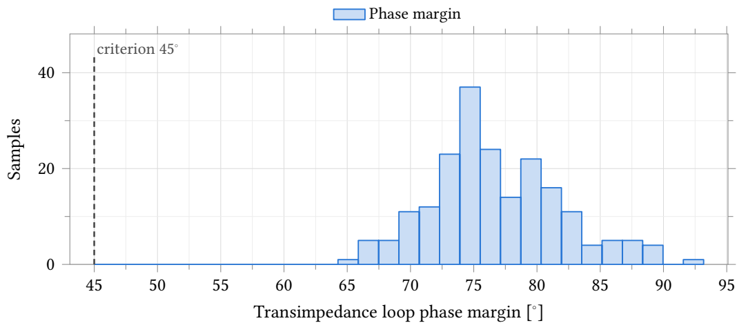
Figure 24.26: Phase margin of the transimpedance loop, conditions as Figure 24.25. The loop is measured through the feedback probe of Figure 24.22 and includes the amplifier, the feedback network and the Randles electrode ( R_s = 100\ \Omega , R_{ct} = 1\ \text{M}\Omega , C_{dl} = 100\ \text{nF} ). All 200 samples clear the 45^\circ criterion, minimum 64.7^\circ . The distribution is right-skewed, so percentiles and the extreme sample are quoted in Table 24.31 rather than \pm 3\sigma .
