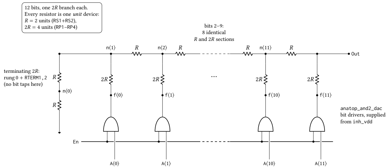
Figure 33.51: The 12-bit voltage-mode R - 2R ladder of anatotop_pixel_dacR2R12 , transcribed from the DacNonLinTB netlist. Bit k drives tap n(k+1) through its own 2R branch, so the twelve taps are n(1) – n(11) plus Out, and the MSB branch lands directly on Out at the top of the ladder; n(0) carries no bit, its rung and R_{TERM1,2} together forming the terminating 2R . Bits 2–9 are elided: eight further sections identical to those drawn sit between n(2) and n(11) . Every element is the same unit resistor, so the network itself is exact and gives \text{Out} = (\text{code}/4096) V_{\text{ref}} ; the reference is the output high level of the anatotop_and2_dac drivers, which sit in series with each 2R branch and bound the ladder in place of the rails: measured zero scale is 20 nV above V_{\text{SS}} and full scale 1.2 \mu\text{V} below the ideal (4095/4096) V_{\text{ref}} on a 2.5 V rail. Device dimensions are proprietary and are not stated.
