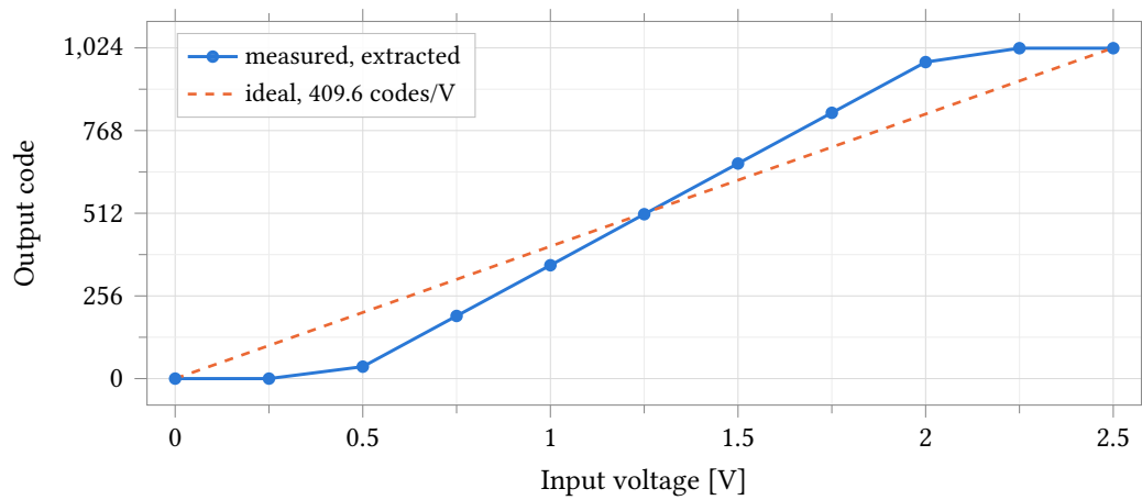
Figure 33.42: Output code against input voltage for the extracted anatop_pixel_adc, nominal corner, 37°C, 2.5 V analog and 1.0 V digital supplies, with the ideal 409.6 codes/V line overlaid. The transfer is monotonic and reaches both code limits, but its slope is 628.64 codes/V, 1.535 times ideal, so the flat segments below 0.44 V and above 2.07 V are the code limits, not the ends of the sweep. Markers are the eleven simulated points; the 0.25 V step is 157 codes, so the curve between them is interpolation and carries no linearity information.
