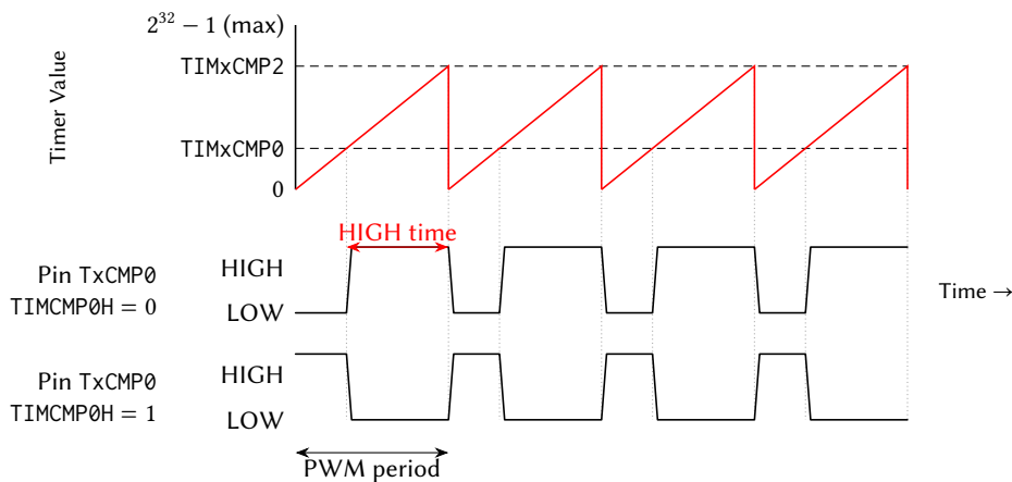
Figure 14: Timer Output Compare and PWM Operation
