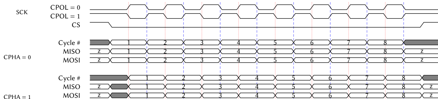
Figure 7: SPI Timing Diagram
