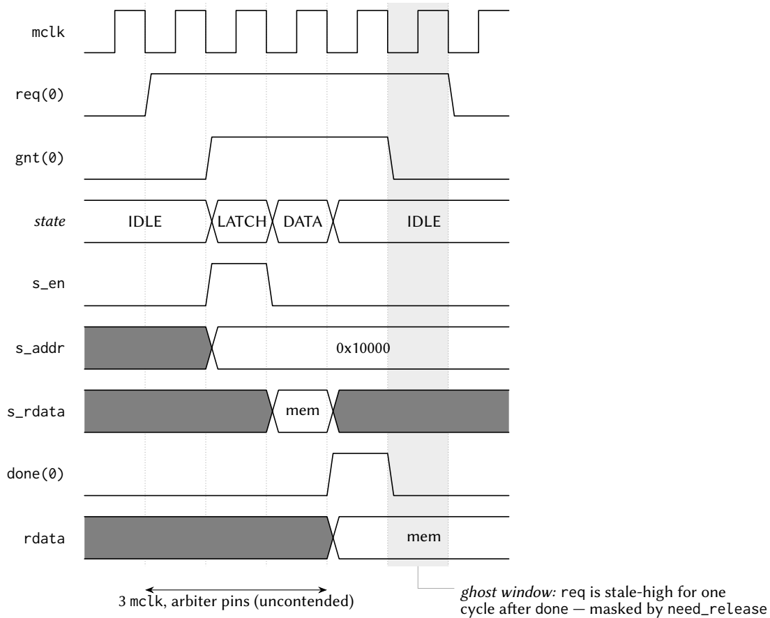
Figure 3: One uncontended shared-window read, at the mp_arbiter pins. The arbiter walks IDLE → LATCH → DATA : the transaction is presented to the slave for one cycle, the synchronous slave returns data the following cycle, and done and rdata are registered together at the edge leaving DATA — three mclk from an observed req . The hart itself sees about two cycles more, one in each direction across the registered tile boundary. In the shaded cycle the master's req is still high although its transaction is over; the arbiter masks that stale request until it is observed low, which is what stops a completed access from being served twice.
