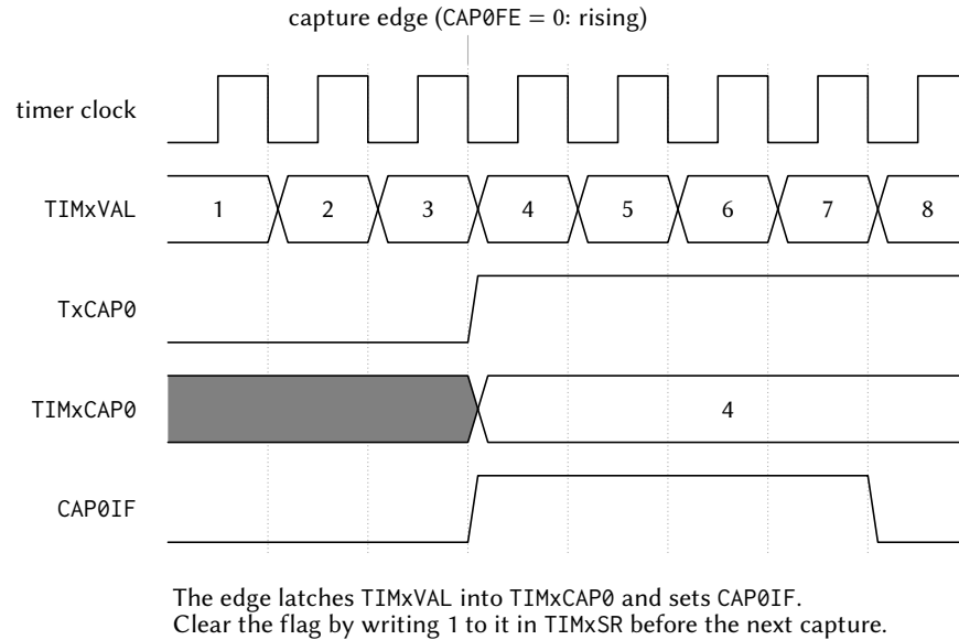
Figure 26: Input capture. The selected edge on TxCAP0 latches the live TIMxVAL into TIMxCAP0 and sets CAP0IF; the flag must be cleared by writing 1 to it in TIMxSR before the next capture event.
