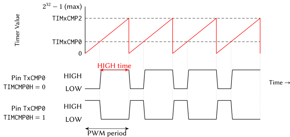
Figure 25: Timer Output Compare and PWM Operation
