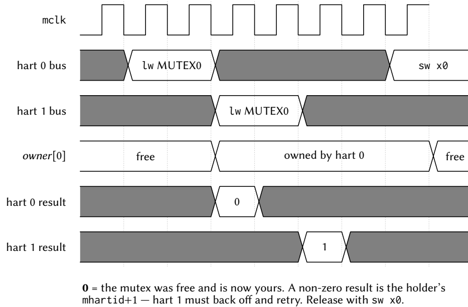
Figure 29: Two harts racing for the same mutex. The arbiter serializes the two claim reads, so the return-old-and-claim happens atomically with no retry loop: hart 0 reads 0 and thereby owns the mutex, and hart 1 reads hart 0's marker and must back off.
