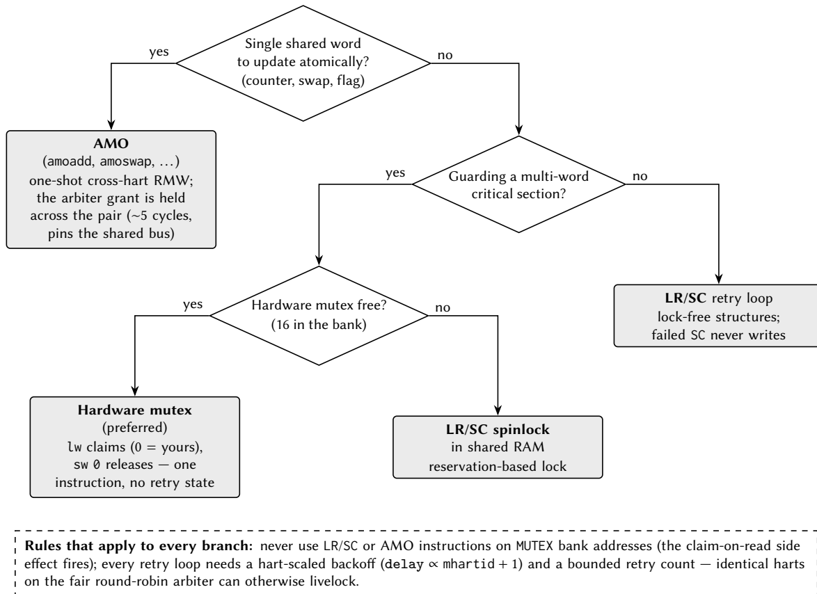
Figure 4: Choosing a synchronization primitive. The dashed box lists the two rules that apply to every branch.
