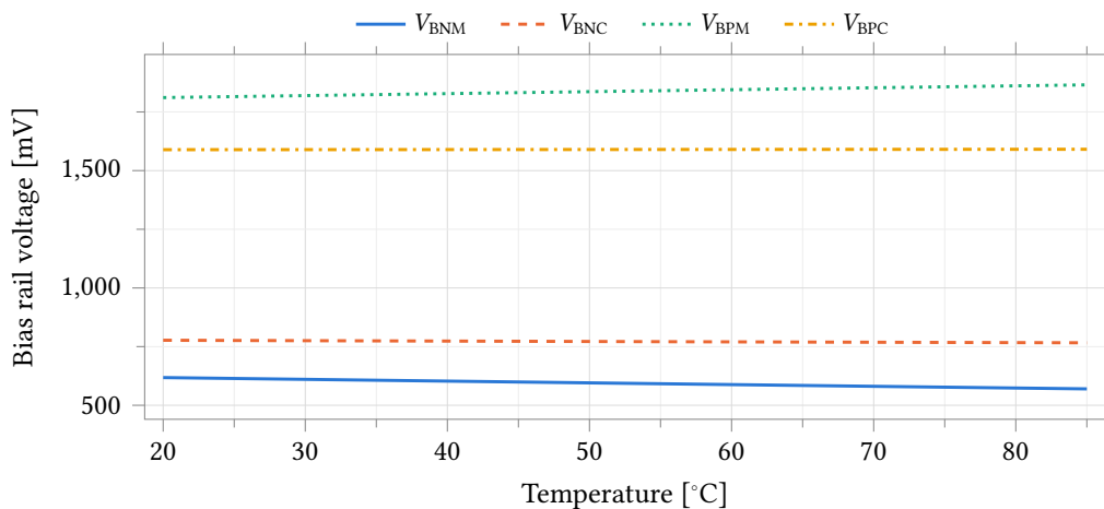
Figure 23: The four local bias rails against temperature at the typical corner. V_{\text{BNM}} and V_{\text{BNC}} are referred to vss!; V_{\text{BPM}} and V_{\text{BPC}} sit near the supply.
