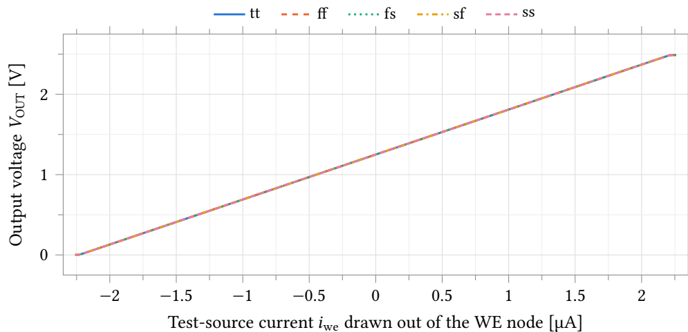
Figure 32: Output voltage against the swept test-source current, over the five process corners. Conditions are R_f = 560 \text{ k}\Omega with the working electrode held at v_{cm} = 1.25 \text{ V} . The bench source draws its current out of the WE node, so i_{we} = -I_{WE} against the convention of Equation (1) and the plotted slope is +R_f : the amplifier sources this current through R_f and the output rises. The \pm 2.26 \mu A sweep takes the output to within 12 mV of vdd and 1.2 mV of vss. The corners overlay to the line width because the slope is the feedback resistor, an ideal component in this bench.
