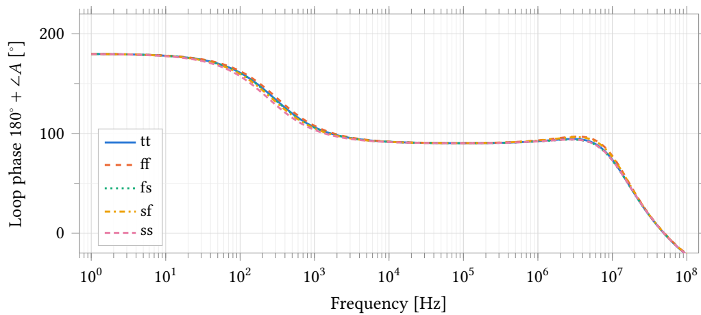
Figure 27: Phase of the same loop-gain measurement, over the five process corners. Spectre’s stb analysis reports 180^\circ + \angle A , so the curve starts at 180^\circ at DC and its value at the 6.4 MHz crossover is the phase margin. The dominant pole costs 90^\circ by 100 kHz; the lift from 90.3^\circ there back to 92.3^\circ at 1 MHz is the left-half-plane zero of Equation (4) adding lead, which is what holds the margin near 88^\circ through crossover despite the second pole at 10.8 MHz.
