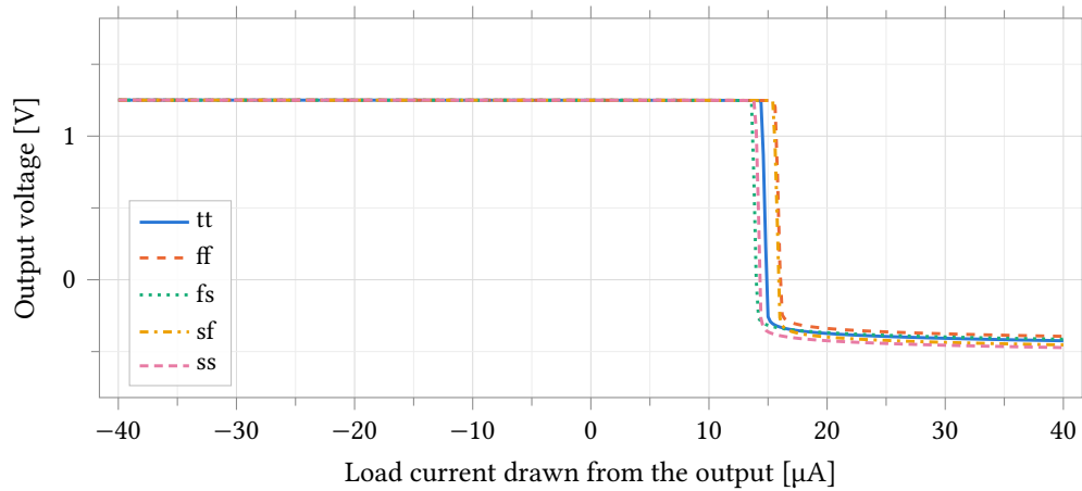
Figure 28: Output voltage of the amplifier in unity feedback as a DC load current is drawn from its output, over the five process corners. Positive current is drawn out of the output node, so the amplifier must source it; the collapse at 13.6 \mu\text{A} to 15.6 \mu\text{A} is the class-A second stage running out of the fixed current in M5. In the sinking direction the output holds within 0.8 mV of v_{\text{cm}} all the way to the -40 \mu\text{A} end of the sweep, so the sinking capability is bounded below by the sweep and not measured.
