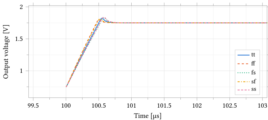
Figure 30: Rising edge of a 1 V step ( v_{\text{cm}} \pm 0.5 \text{ V} ) in unity feedback into 5 pF, over the five process corners. The window is 3.5 \mu\text{s} around the edge at 100 \mu\text{s} ; the falling edge at 1.1 \text{ ms} is outside it. The output slews for about 0.4 \mu\text{s} , overshoots once by 5.0 % to 9.0 % of the step and recovers without ringing — the excursion is slow recovery, not small-signal ringing, which is what the 88^\circ phase margin of Table 22 predicts.
