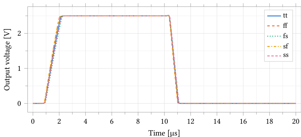
Figure 29: Large-signal response with the amplifier open-loop, driven by a rail-to-rail input pulse into 5 pF, over the five process corners. The falling edge is 1.7 times faster than the rising edge for the same reason the drive is asymmetric: the second stage is class A, and M12 sinks the load with a device eight times wider than the fixed current source M5 that has to source it.
