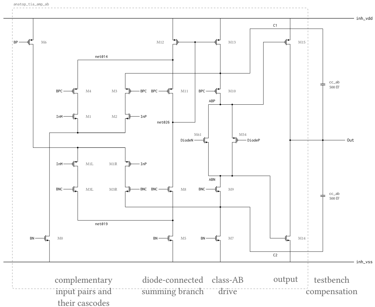
Figure 34: Signal-path topology of the class-AB amplifier anatop_tia_amp_ab , drawn from its netlist. The complementary pairs M1/M2 (NMOS, tail M0 ) and M1L/M1R (PMOS, tail M6 ) fold into two cascode branches; the InM side terminates in the diode-connected branch M12–M11–M8–M5 , whose summing node net026 sets M13 , which restates that current into the InP branch, and the floating pair M54/M61 holds ABP above ABN so both output devices M15 and M14 are actively driven. C1 and C2 are the common source nodes of the PMOS cascodes M10/M3 and of the NMOS cascodes M9/M3R , brought out as pins; the two cc_ab capacitors that return them to Out sit outside the cell boundary (dashed) in the testbench, 500 fF per side. Simplified: the enable switch and its four power-down devices, and the bias generator that develops DiodeN/DiodeP , are omitted, so 22 of the cell’s 34 transistors are drawn; BP/BPC/BN/BNC are the enable-gated forms of the bp!/bpc!/bn!/bnc! globals and device dimensions are not shown. Identically labelled nets are connected; wires crossing without a filled dot are not.
