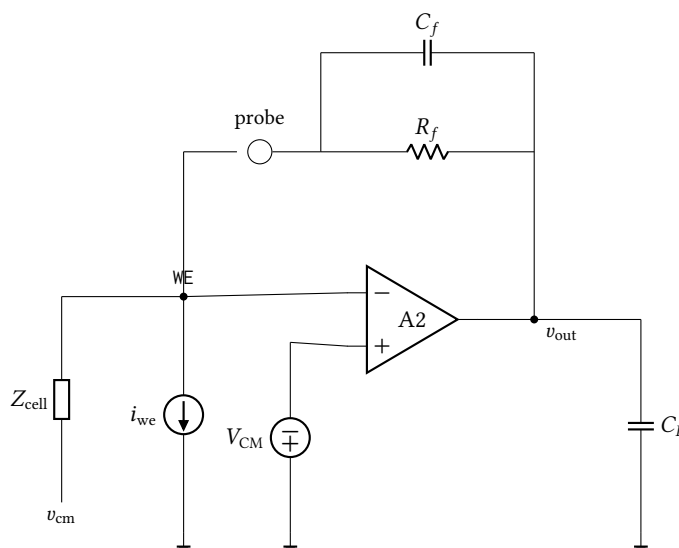
Figure 35: The closed transimpedance loop bench, the only one in this section that closes feedback around the electrode. R_f \parallel C_f returns the output to the working electrode through a current probe, i_{we} is the test source, and Z_{cell} is the Randles cell of Figure 12, returned to v_{cm} . The loop gain, phase margin and crossover are measured through the probe; the DC accuracy, closed-loop transfer and noise figures come from the same wiring.
