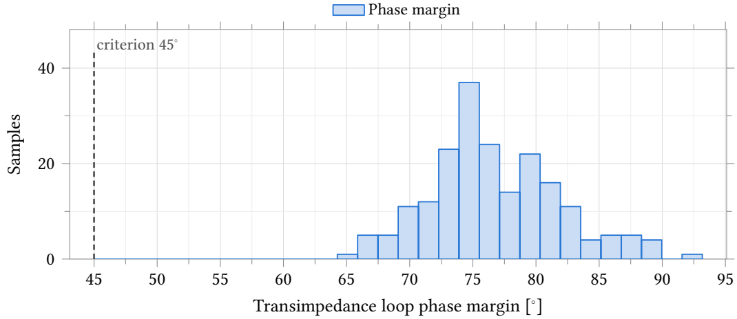
Figure 40: Phase margin of the transimpedance loop, conditions as Figure 39. The loop is measured through the feedback probe of Figure 35 and includes the amplifier, the feedback network and the Randles electrode ( R_s = 100 \Omega , R_{ct} = 1 \text{ M}\Omega , C_{dl} = 100 \text{ nF} ). All 200 samples clear the 45^\circ criterion, minimum 64.7^\circ . The distribution is right-skewed, so percentiles and the extreme sample are quoted in Table 36 rather than \pm 3\sigma .
