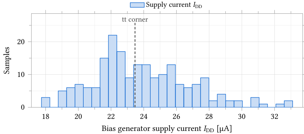
Figure 33: Supply current of the local bias generator over 200 process-and-mismatch samples, with the tt corner at the same trim code marked. Monte Carlo gives \sigma/\mu = 12.5\% , 17.7–33.1 \mu\text{A} , where the five process corners span 1.2 %, 23.25–23.52 \mu\text{A} (Table 12, interpolated to BiasAdj = 37); the corner sweep is at 27 °C against 37 °C here, which accounts for the 0.45 \mu\text{A} of mean offset and not for the width. A self-biased loop fixes its current by a device-ratio and resistor balance that a global corner shift leaves intact but local mismatch does not, so corner analysis under-reports this term tenfold. It is the largest single contributor to A1’s own spread (peak cell current 14.5 %, f_u 12.4 %), leaving roughly 7 % in quadrature for the amplifier’s own devices. This is a separate netlist and a separate draw, so sample n here is not sample n in the A1 tests and the two must not be paired.
