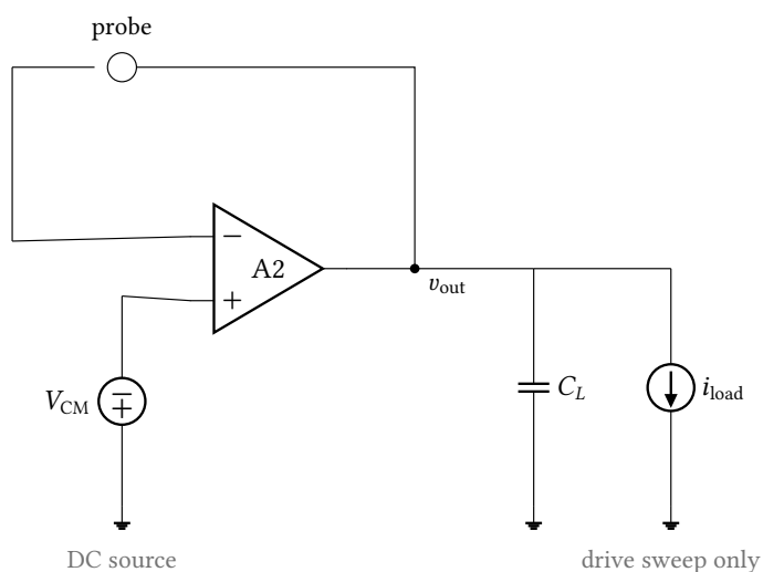
Figure 36: Unity-feedback bench. The amplifier's output is returned to its inverting input through a current probe and loaded by C_L = 5 pF; the loop-gain analysis through that probe gives the amplifier's own gain and margins, and DC and noise analyses on the same wiring give the offset and output noise. The drive measurement adds the swept load current i_{load} on the same schematic. Supplies, the bias rails and the enable pin are omitted here and in Figure 35.
