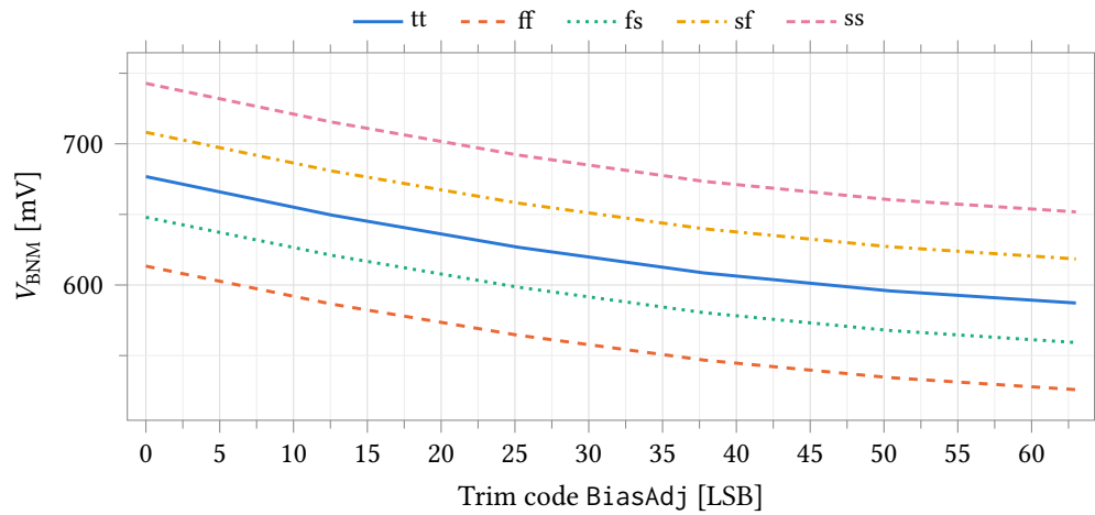
Figure 21: Trim characteristic: V_{\text{BNM}} against the BiasAdj word over all process corners. The bench sweeps the trim word as a continuous variable, so only the six codes 0, 12.6, 25.2, 37.8, 50.4 and 63 are sampled: this is the shape of the trim law, not a per-code characterisation.
