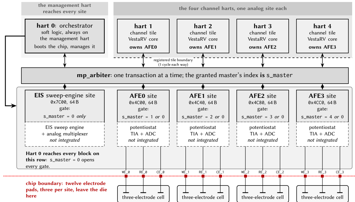
Figure 11: Analog front-end connectivity: who reaches which site, and what leaves the die. Each channel hart owns exactly one measurement site and reaches no other; hart 0, the orchestrator, opens every gate in the row, because the gate compares the arbiter's granted-master index against a single owner and against 0. The analog stages are drawn dashed because they are not yet integrated: what the chip carries today is the digital register site in front of each one (and the pads behind them). Each site brings out a three-electrode cell: WE the working electrode, RE the reference, CE the counter. A fourth pad per site, RE_{2h} , is bonded as well and is not drawn: it is the second sense electrode of the optional four-terminal (Kelvin) configuration.
