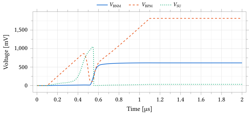
Figure 34: Power-up transient at the typical corner. The start-up node V_{SU} pulls the core out of its zero-current state, after which both mirror rails settle to their steady-state values.
