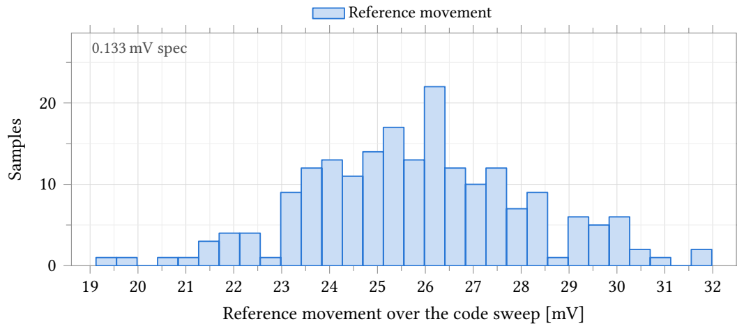
Figure 79: Peak-to-peak movement of the DAC reference VddDac across the 4096-code sweep, with the ladder referenced to the on-chip supply block instead of an ideal rail. Process and mismatch , castalia_pm_25, 200 samples, 25 °C, no external load on VddDac. The quarter-LSB budget of 133 \mu V entered on the test sits about 200 times below the data, so it is annotated at the left axis edge rather than drawn and the distribution is not compressed into a single bar; the closest sample misses it by a factor of 144. Meeting it needs the supply’s output impedance down by a factor of 193, to about 5 \Omega , against 894 \Omega small-signal (Table 87) and 1133 \Omega as a 0 \mu A to 100 \mu A chord (Table 83).
