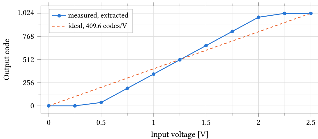
Figure 61: Output code against input voltage for the extracted anatop_pixel_adc, nominal corner, 37 °C, 2.5 V analog and 1.0 V digital supplies, with the ideal 409.6 codes/V line overlaid. The transfer is monotonic and reaches both code limits, but its slope is 628.64 codes/V — 1.535 times ideal — so the flat segments below 0.44 V and above 2.07 V are the code limits, not the ends of the sweep. Markers are the eleven simulated points; the 0.25 V step is 157 codes, so the curve between them is interpolation and carries no linearity information.
