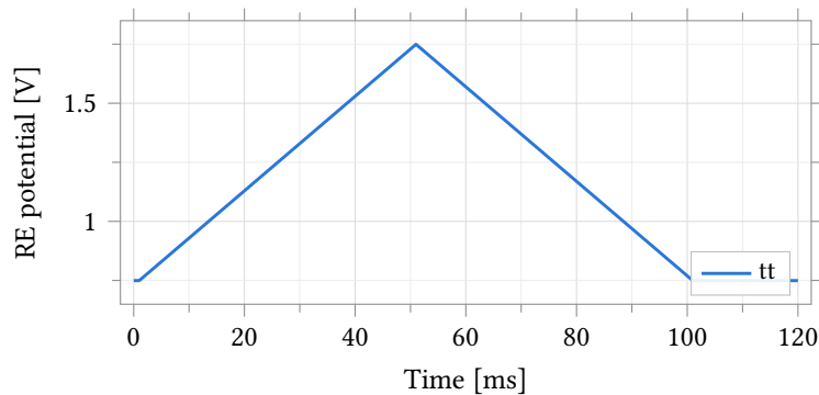
Figure 54: Commanded reference-electrode potential against time for the triangular voltammetry sweep, typical process point, 37^\circ\text{C} , R_f = 35\text{ k}\Omega , R_{ct} = 1\text{ M}\Omega electrode. Paired with the current response of Figure 53.
