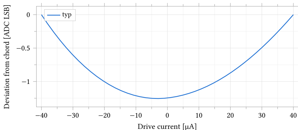
Figure 68: Drive nonlinearity of the bottom code ( N = 0 , R \approx 19.6 \text{ k}\Omega ): voltage deviation from the endpoint chord over \pm 90\% of full scale ( \pm 40 \mu\text{A} ), typical corner, expressed in 1.592 \text{ mV ADC LSB} . All ten bypass gates are closed at this code and carry the full signal current; their on-resistance rises with the terminal's excursion from V_{\text{CM}} , so the chord — pinned at the sweep endpoints where that excursion is largest — overestimates the mid-range voltage by up to 1.25 \text{ LSB} , and the deviation is bowl-shaped with a slight skew from the gates' voltage asymmetry. The same measurement at N = 63 and N = 319 , where the ladder dominates and current is 20\text{--}100\times smaller, stays below 0.004 \text{ LSB} and is tabulated, not plotted.
