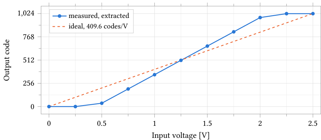
Figure 64: Output code against input voltage for the extracted anatop_pixel_adc , nominal corner, 37 °C, 2.5 V analog and 1.0 V digital supplies, with the ideal 409.6 codes/V line overlaid. The transfer is monotonic and reaches both code limits, but its slope is 628.64 codes/V — 1.535 times ideal — so the flat segments below 0.44 V and above 2.07 V are the code limits, not the ends of the sweep. Markers are the eleven simulated points; the 0.25 V step is 157 codes, so the curve between them is interpolation and carries no linearity information.
