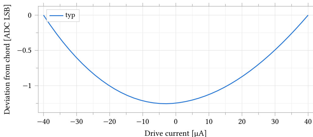
Figure 71: Drive nonlinearity of the bottom code ( N = 0 , R \approx 19.6 \text{ k}\Omega ): voltage deviation from the endpoint chord over \pm 90\% of full scale ( \pm 40 \mu\text{A} ), typical corner, expressed in 1.592 \text{ mV ADC LSB} . All ten bypass gates are closed at this code and carry the full signal current; their on-resistance rises with the terminal's excursion from V_{\text{CM}} , so the chord — pinned at the sweep endpoints where that excursion is largest — overestimates the mid-range voltage by up to 1.25 \text{ LSB} , and the deviation is bowl-shaped with a slight skew from the gates' voltage asymmetry. The same measurement at N = 63 and N = 319 , where the ladder dominates and current is 20\text{--}100\times smaller, stays below 0.004 \text{ LSB} and is tabulated, not plotted.
