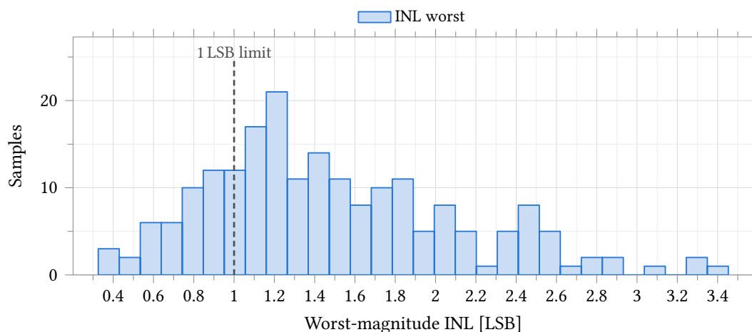
Figure 80: Integral nonlinearity of the R - 2R ladder driven from an ideal 2.5 V reference. Process and mismatch , model section castalia_pm_25 , 200 samples, seed 12345, low-discrepancy sampling, 25^\circ\text{C} , all 4096 codes. The dashed rule is the 1 LSB limit entered on the test; 42 of 200 samples fall inside it and the worst reaches 3.453 LSB. The distribution is right-skewed (Fisher skew +0.74 ), so Table 86 quotes the median and percentiles rather than \text{mean} \pm 3\sigma . LSB size, full scale and gain error are fixed to a part in 10^6 on this bench (Table 87), so the whole of this spread is resistor mismatch in the ladder and none of it is the reference.
