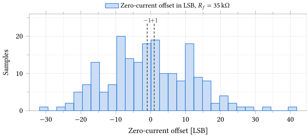
Figure 56: Zero-current output offset at R_f = 35\text{ k}\Omega , in nominal 2.441\text{ mV} ADC LSB. Mismatch only , 25^\circ\text{C} nominal process, 200 samples, R_{\text{ct}} = 10\text{ k}\Omega electrode. The limit shown is the \pm 1\text{ LSB} entered on the test in Assembler – comparable in kind across the four gain taps but mechanically harder to meet as R_f rises, since the underlying offset is closer to gain-independent in current (Table 64). The converter's measured step is 1.591\text{ mV} , not the nominal 2.441\text{ mV} (Table 72); multiply the axis and the limit by 1.535 to read them as converter codes. Statistics are in Table 64.
