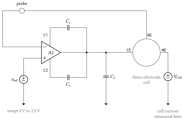
Figure 46: Cell-drive bench. The amplifier drives the counter electrode of a three-electrode cell and closes its loop on the reference electrode, with the commanded potential v_{ref} swept over the full 0 V to 2.5 V supply range. The working electrode is held at V_{CM} by an ideal source: no load current is injected, so the cell current is set by the sweep against the cell impedance and is measured in that source, and the regulation errors quoted at \pm 10 \mu\text{A} are read off the sweep at the points where the cell current reaches those values. The probe in the reference-electrode return measures the loop gain with the cell inside the loop; it is not the amplifier's own gain, and the two are tabulated separately. Cell elements are R_{ce} = R_u = 1 \text{ k}\Omega and R_{ct} = 10 \text{ k}\Omega in parallel with C_{dl} = 1 \mu\text{F} (Figure 19), the load is C_L = 5 \text{ pF} , and each external compensation capacitor C_c is 500 fF.
