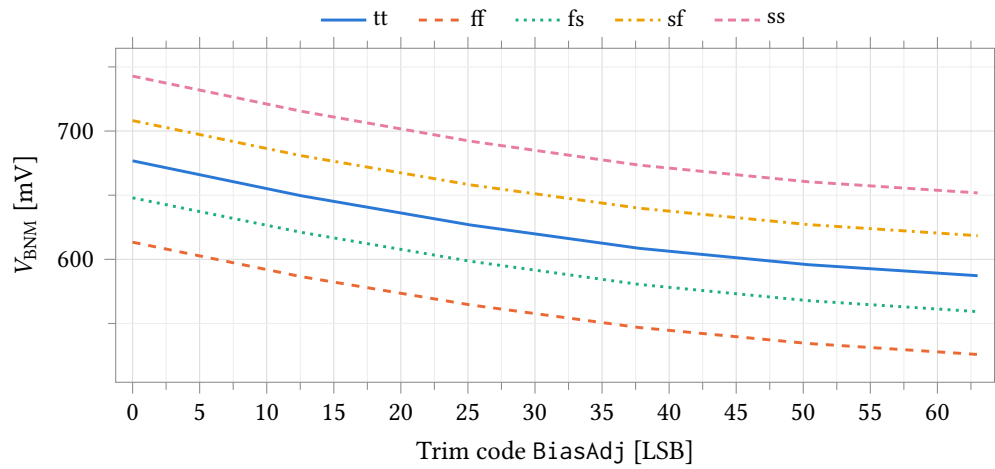
Figure 18: Trim characteristic: V_{BNM} against the BiasAdj word over all process corners. The bench sweeps the trim word as a continuous variable, so only the six codes 0, 12.6, 25.2, 37.8, 50.4 and 63 are sampled — this is the shape of the trim law, not a per-code characterisation.
