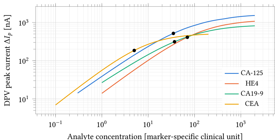
Figure 33.6: Dose response of the four-reporter panel: published-assay binding curves composed with the current transfer measured from the DPV runs of Figure 33.5 (11 simulated concentrations per reporter, 560 kΩ tap). Filled circles are the clinical decision points through the same chain: CA-125 35 U/mL → 517 nA, HE4 70 pmol L -1 → 409 nA, CA19-9 37 U/mL → 313 nA, CEA 5 ng mL -1 → 185 nA. The concentration axis carries each marker's own clinical unit; only the current axis is common. The binding model is analytic; the electrode and channel behind the current axis are simulated.
