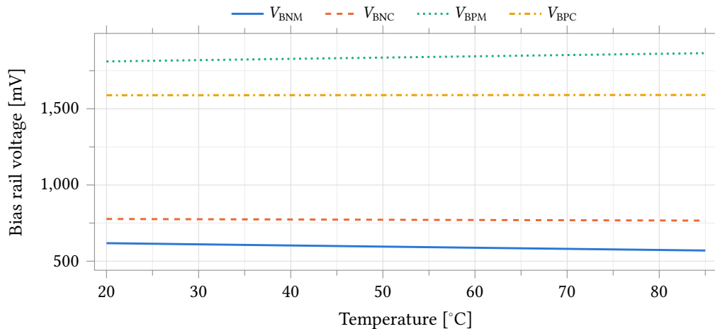
Figure 33.9: The four local bias rails against temperature at the typical corner. V_{\text{BNM}} and V_{\text{BNC}} are referred to vss!; V_{\text{BPM}} and V_{\text{BPC}} sit near the supply.
