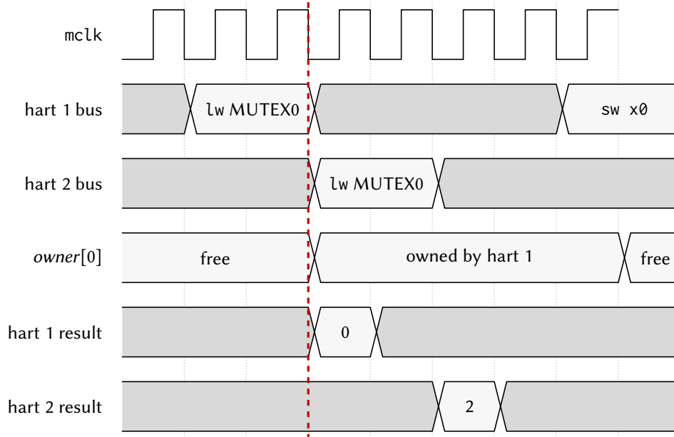
Figure 22.1: Two harts racing for the same mutex: the first read returns 0 and takes the word, the second returns the holder's marker ( mhartid + 1 ) and must retry, and the holder releases with sw x0 .
