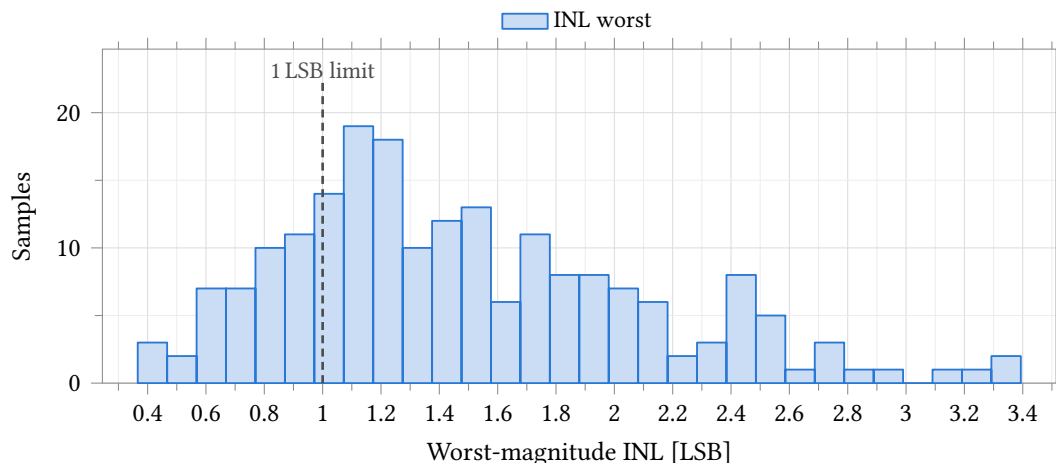
Figure 33.54: Integral nonlinearity of the R - 2R ladder driven from an ideal 2.5 V reference, with the custom 2.5 V bit driver anatop_and2_dac the tapeout cell carries. Process and mismatch , model section castalia_pm_25 , 200 samples, seed 12345, low-discrepancy sampling, 25 °C, all 4096 codes. The dashed rule is the 1 LSB limit entered on the test; 41 of 200 samples fall inside it and the worst reaches 3.393 LSB. The distribution is right-skewed (Fisher skew +0.74 ), so Table 33.70 quotes the median and percentiles rather than \text{mean} \pm 3\sigma . LSB size, full scale and gain error are fixed to a part in 10^6 on this bench (Table 33.71), so the whole of this spread is resistor mismatch in the ladder and none of it is the reference.
