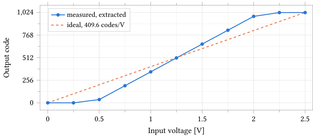
Figure 33.42: Output code against input voltage for the extracted anatop_pixel_adc, nominal corner, 37°C, 2.5 V analog and 1.0 V digital supplies, with the ideal 409.6 codes/V line overlaid. The transfer is monotonic and reaches both code limits, but its slope is 628.64 codes/V, 1.535 times ideal, so the flat segments below 0.44 V and above 2.07 V are the code limits, not the ends of the sweep. Markers are the eleven simulated points; the 0.25 V step is 157 codes, so the curve between them is interpolation and carries no linearity information.
