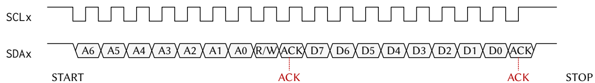
Figure 20.1: One I2C byte write on the wire: START, address, ACK, data byte, ACK, STOP.
