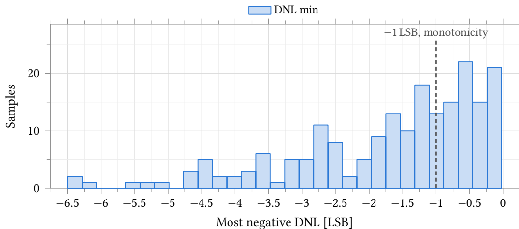
Figure 33.55: Worst negative differential nonlinearity, same bench, samples and bit driver as Figure 33.54. The dashed rule at -1 LSB is the monotonicity limit entered on the test: 84 of 200 samples clear it, so 42.0 % of channels are monotonic and 0.420^4 = 3.1 % of four-channel chips are monotonic on all four. Graded on integral nonlinearity as well, 37 of 200 pass and the four-channel figure is 0.12 %. The distribution is left-skewed (skew -1.14 ) with a tail to -6.499 LSB, so the median -1.287 LSB and the percentiles of Table 33.70 describe it and \text{mean} \pm 3\sigma does not.
