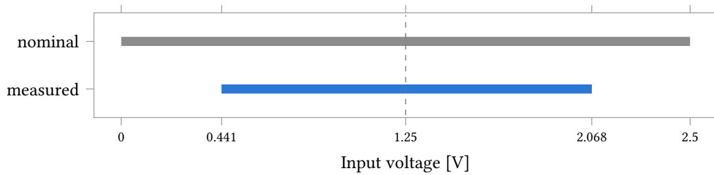
Figure 33.44: Usable input window of the converter against the nominal 0 V to 2.5 V supply span. The measured window runs 0.441 V to 2.068 V, 1.627 V wide, so 34.9 % of the nominal span is unreachable: 0.441 V at the bottom and 0.432 V at the top, near enough symmetric about the 1.25 V common mode (dashed). Outside that window the output sits at a code rail, so a transimpedance swing wider than \pm 0.81 V about V_{CM} is truncated rather than digitised.
