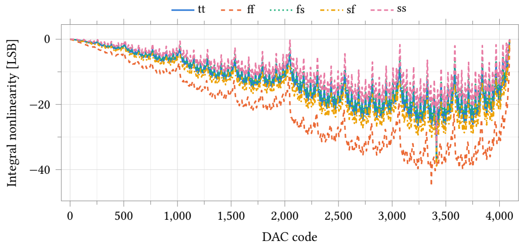
Figure 33.58: Integral nonlinearity against code over five process corners with the ladder referenced to V_{ddDac} from the supply block, zero external load, 25 °C. Endpoint-line INL as in Figure 33.52; the vertical scale is tens of LSB, not tenths. The bow reaches −37.1 LSB at tt (code 3413) and −45.1 LSB at ff (code 3365) and tracks the reference droop of Figure 33.57 scaled by code. Dividing each code’s output by the reference measured at that code removes it and leaves 0.43 to 0.45 LSB (Table 33.73), so the ladder is unchanged from the ideal-rail case.
