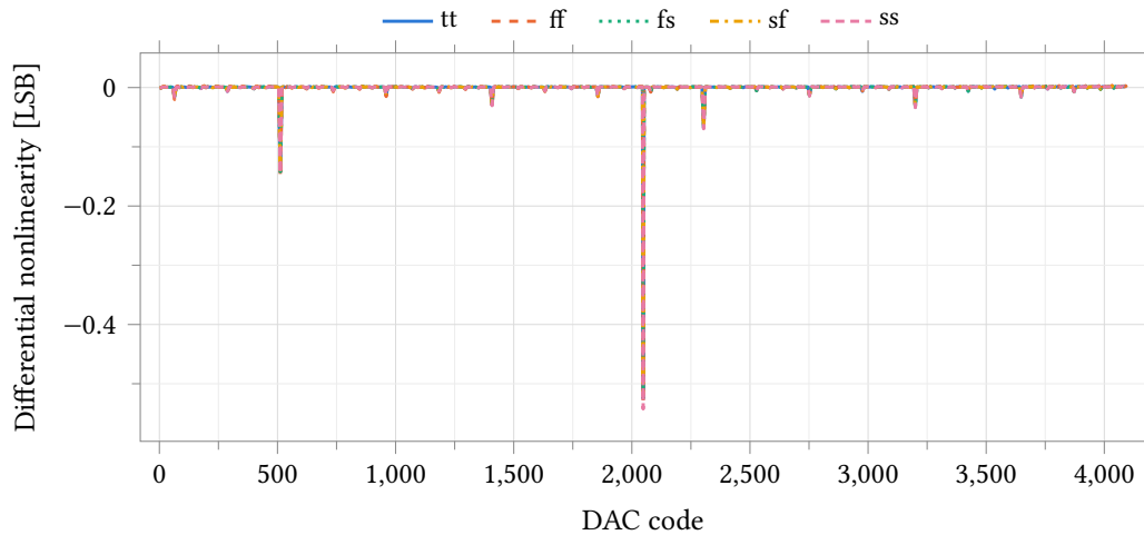
Figure 33.59: Ratiometric differential nonlinearity against code over five process corners: each code's output is divided by the reference measured at that code before the LSB and the first difference are taken, so the reference droop divides out and the ladder alone is measured. Conditions as Figure 33.58; the 4095-point curve is stride-decimated for the plot as in Figure 33.53. The major-carry hierarchy is the ideal-rail one ( -0.53 at code 2048, then -0.28 at 1024, -0.24 at 3072, -0.14 at 512 and -0.13 LSB at 2560), and the worst step matches Figure 33.53 to within 0.03 LSB. Raw DNL on the same bench is -9.8 to -18.4 LSB (Table 33.73); the difference is the reference step between adjacent codes and nothing else.
