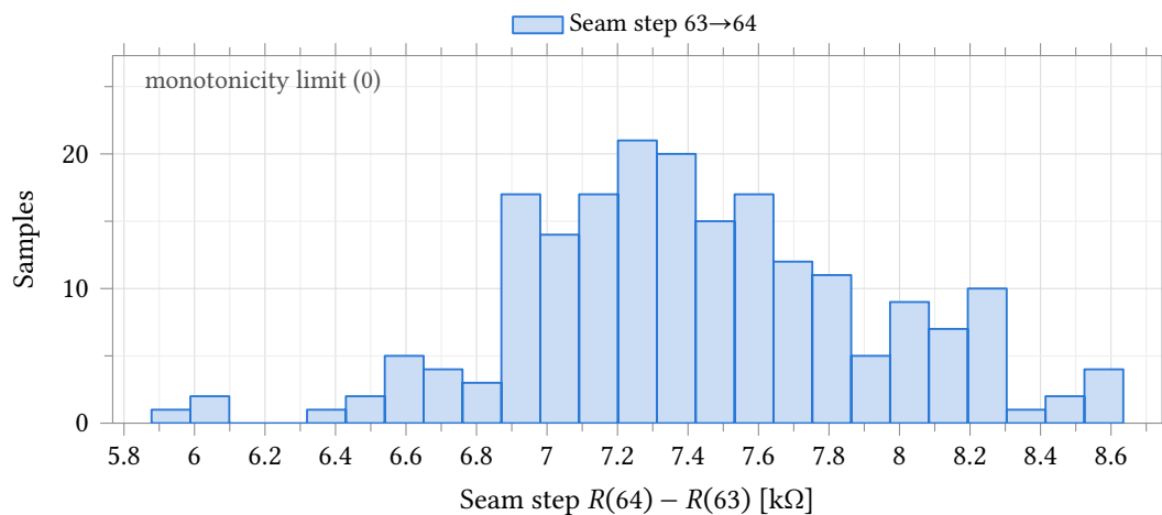
Figure 33.50: Per-sample step across the first thermometer seam (code 63 to 64: one 64-unit segment switches in while all six binary segments switch out), the code transition most exposed to mismatch. Mismatch only , model section castalia_pm_25 , nominal process, 200 samples, seed 12345, low-discrepancy sampling, 25 °C. Mean 7.42 k \Omega , \sigma = 504 \Omega , worst sample 5.88 k \Omega , 14.7\sigma above the monotonicity limit at zero, so no realistic mismatch closes the seam.
