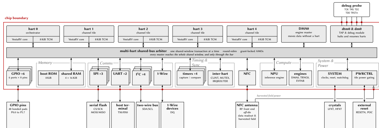
Figure 2.1: Castalia whole-chip diagram: the masters above one mp_arbiter bus bar, every peripheral on one rank below it, and the package boundary in red.
