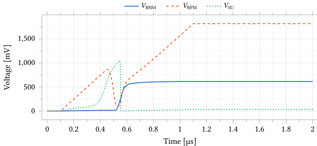
Figure 33.16: Power-up transient at the typical corner. The start-up node V_{SU} pulls the core out of its zero-current state, after which both mirror rails settle to their steady-state values.
