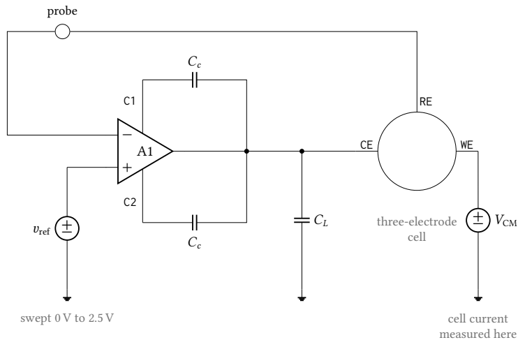
Figure 33.28: Cell-drive bench. The amplifier drives the counter electrode of a three-electrode cell and closes its loop on the reference electrode, with the commanded potential v_{ref} swept over the full 0\text{ V} to 2.5\text{ V} supply range. The working electrode is held at V_{CM} by an ideal source: no load current is injected, so the cell current is set by the sweep against the cell impedance and is measured in that source, and the regulation errors quoted at \pm 10\text{ }\mu\text{A} are read off the sweep at the points where the cell current reaches those values. The probe in the reference-electrode return measures the loop gain with the cell inside the loop; it is not the amplifier's own gain, and the two are tabulated separately. Cell elements are R_{ce} = R_u = 1\text{ k}\Omega and R_{ct} = 10\text{ k}\Omega in parallel with C_{dl} = 1\text{ }\mu\text{F} (Figure 33.1), the load is C_L = 5\text{ pF} , and each external compensation capacitor C_c is 500\text{ fF} .
