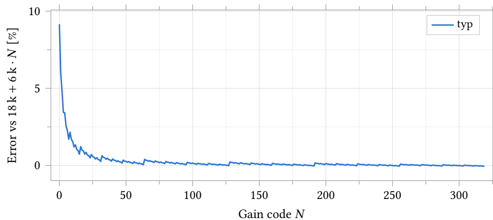
Figure 33.48: Typical-corner deviation from the ideal code law. The +9.2 % at N = 0 is the series resistance of the ten closed bypass switches (1.65 k \Omega , about 165 \Omega each), which decays as 1/R once real ladder segments dominate; by N = 319 the error is -0.063 %. The ripple is the carry structure: at each binary carry and at each thermometer seam the set of closed switches changes, so the R_{on} term steps while the ladder term is exact.
