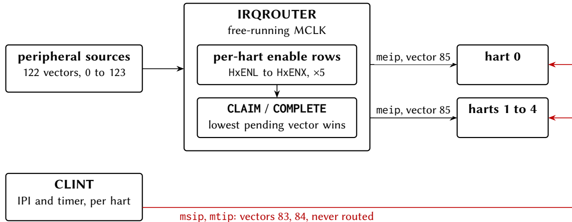
Figure 32.1: The interrupt fabric: peripheral sources, the router’s enable rows and claim/complete stage, the harts, and the CLINT pair in red because it bypasses the router.
