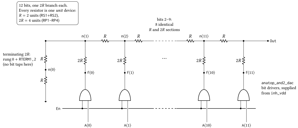
Figure 33.51: The 12-bit voltage-mode R - 2R ladder of anatotp_pixel_dacR2R12 , transcribed from the DacNonLinTB netlist. Bit k drives tap n(k+1) through its own 2R branch, so the twelve taps are n(1) – n(11) plus Out, and the MSB branch lands directly on Out at the top of the ladder; n(0) carries no bit, its rung and R_{TERM1,2} together forming the terminating 2R . Bits 2–9 are elided: eight further sections identical to those drawn sit between n(2) and n(11) . Every element is the same unit resistor, so the network itself is exact and gives \text{Out} = (\text{code}/4096) V_{\text{ref}} ; the reference is the output high level of the anatotp_and2_dac drivers, which sit in series with each 2R branch and bound the ladder in place of the rails: measured zero scale is 20 nV above V_{\text{SS}} and full scale 1.2 \mu\text{V} below the ideal (4095/4096) V_{\text{ref}} on a 2.5 V rail. Device dimensions are proprietary and are not stated.
