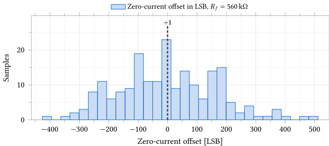
Figure 33.39: Zero-current output offset at R_f = 560\text{ k}\Omega , conditions as Figure 33.38 but at R_{ct} = 10\text{ k}\Omega (the same stiff electrode as the finite-loop-gain demonstration of Table 33.44, NOT the 1 M \Omega operational electrode of Table 33.43). Some samples reach the sweep’s output rails (Table 33.53); the LSB spread here is 14 \times wider than at 35 k \Omega for the same underlying current offset, since the same offset current is multiplied through a 16 \times larger R_f .
