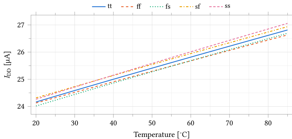
Figure 33.11: Quiescent supply current of the bias generator against temperature over all process corners. The corner separation drawn here is a lower bound: the corner set holds the passive model rows at typical (pinned-passive caveat, page 287).
