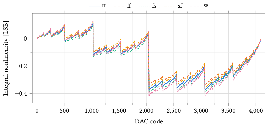
Figure 33.52: Integral nonlinearity against code over five process corners, ladder on an ideal 2.5 V rail, 25 °C, \text{reltol} = 1 \times 10^{-6} . INL is taken from the endpoint line through each corner's own zero- and full-scale outputs, so it is zero at codes 0 and 4095 by construction; the run is the 2026-09-06 five-corner sweep on the tapeout cell, with the custom 2.5 V bit driver anatop_and2_dac . The positive extreme is code 1023 at every corner, +0.10 to +0.13 LSB; the negative extreme is the major carry at code 2048 or 3072, which sit within 0.006 LSB of each other at -0.34 to -0.41 LSB, so which of the two wins flips with the corner while the shape does not. Corner run, no device mismatch: R-2R linearity is a matching property, so this envelope is the systematic term alone.
