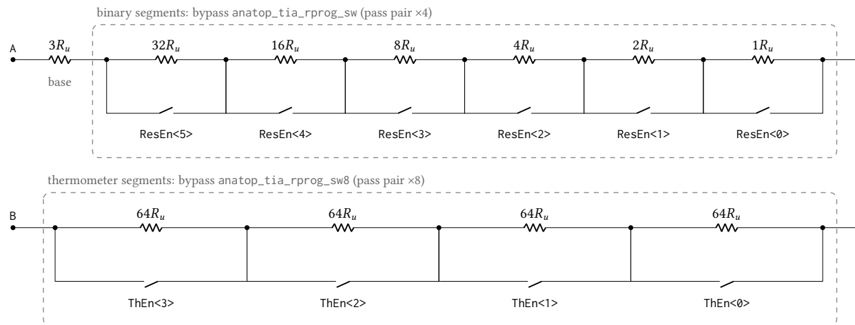
Figure 33.46: Segment and bypass-switch structure of anatop_tia_rprog , transcribed from the executed spec-run netlist. The unit R_u is one series poly resistor; from terminal A the chain runs through the never-switched three-unit base, the six binary-weighted segments of 32 down to 1 unit, and the four identical 64-unit thermometer segments to terminal B. Each switched segment is shunted by a CMOS transmission gate with a local inverter: the control pin EnBar is the ResEn/ThEn bit itself and drives the PMOS pass gate directly and the NMOS pass gate through the inverter, so a bit at 1 turns both pass devices off and inserts the segment. The pass pair has multiplicity 4 in the binary switch ( _sw ) and 8 in the thermometer switch ( _sw8 ), which halves the thermometer gates' on-resistance where up to six binary gates close at a seam. Three grounded dummy units accompany the 322 active units for matching.
