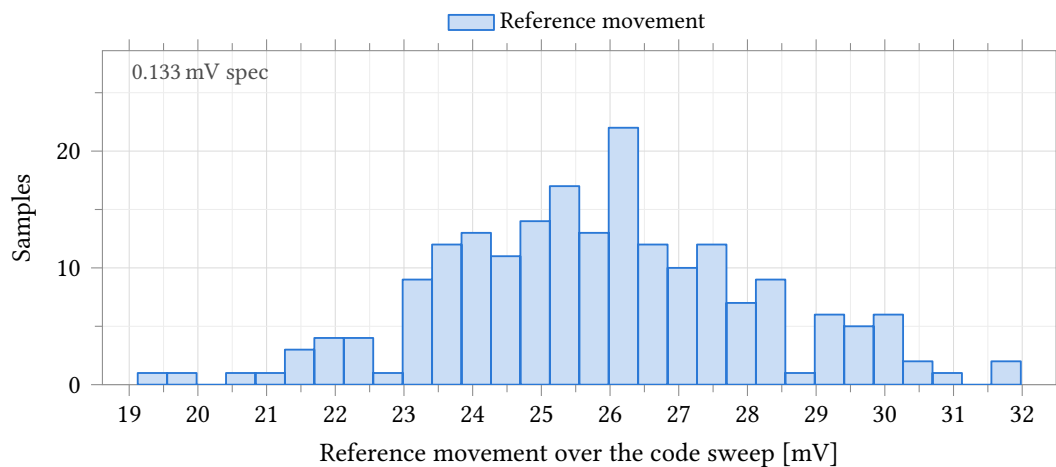
Figure 33.60: Peak-to-peak movement of the DAC reference VddDac across the 4096-code sweep, with the ladder referenced to the on-chip supply block instead of an ideal rail. Process and mismatch , castalia_pm_25, 200 samples, 25 °C, no external load on VddDac. The quarter-LSB budget of 133 \mu\text{V} entered on the test sits about 200 times below the data, so it is annotated at the left axis edge rather than drawn and the distribution is not compressed into a single bar; the closest sample misses it by a factor of 144. Meeting it needs the supply’s output impedance down by a factor of 193, to about 5 \Omega , against 894 \Omega small-signal (Table 33.81) and 1133 \Omega as a 0 \mu\text{A} to 100 \mu\text{A} chord (Table 33.77).
