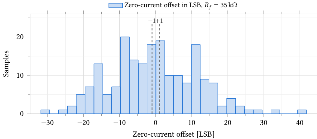
Figure 33.38: Zero-current output offset at R_f = 35\text{ k}\Omega , in nominal 2.441 mV ADC LSB. Mismatch only , 25 °C nominal process, 200 samples, R_{ct} = 10\text{ k}\Omega electrode. The limit shown is the \pm 1 LSB entered on the test in Assembler – comparable in kind across the four gain taps but mechanically harder to meet as R_f rises, since the underlying offset is closer to gain-independent in current (Table 33.53). The converter’s measured step is 1.591 mV, not the nominal 2.441 mV (Table 33.58); multiply the axis and the limit by 1.535 to read them as converter codes. Statistics are in Table 33.53.
