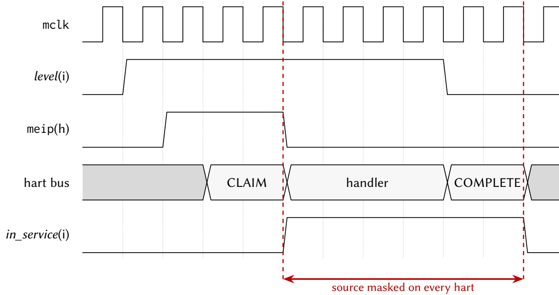
Figure 32.2: Claim/complete delivery of one peripheral interrupt.
