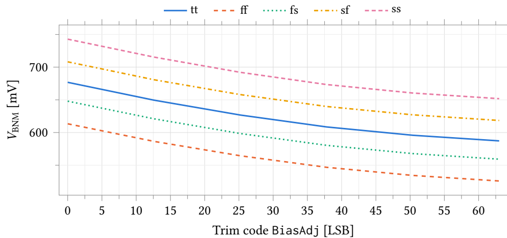
Figure 33.14: Trim characteristic: V_{\text{BNM}} against the BiasAdj word over all process corners. The bench sweeps the trim word as a continuous variable, so only the six codes 0, 12.6, 25.2, 37.8, 50.4 and 63 are sampled: this is the shape of the trim law, not a per-code characterisation. The corner separation drawn here is a lower bound: the corner set holds the passive model rows at typical (pinned-passive caveat, page 287).
