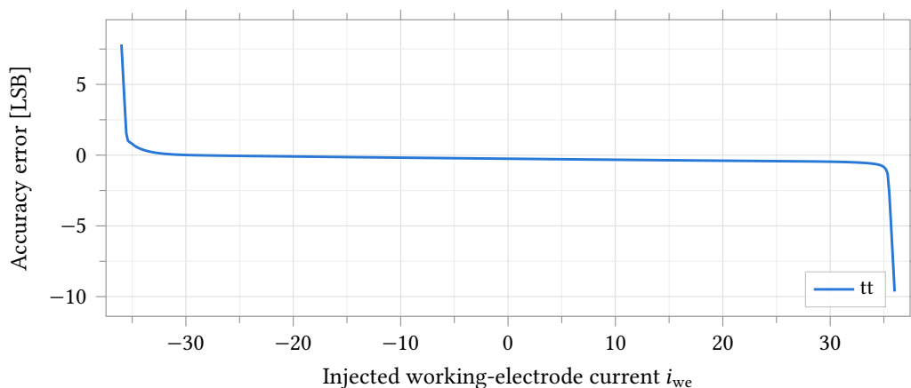
Figure 33.32: Bipolar accuracy error against injected working-electrode current, R_f = 35\text{ k}\Omega , R_{ct} = 10\text{ k}\Omega electrode, typical process point, 37 °C, full \pm 36\text{ }\mu\text{A} sweep (full scale \pm 33\text{ }\mu\text{A} ). The zero crossing is smooth with no kink or discontinuity between the sourcing and sinking halves of the sweep: the error’s slope through zero is -1/T exactly (Table 33.42) and the same single anatop_tia_amp_ab TIA feedback path serves both current directions, unlike the rev-1 PMOS-only mirror it replaces. The error axis is referred to the nominal 2.441 mV step; the converter’s measured step is 1.591 mV (Table 33.58), so multiply by 1.535 to read it as converter codes.
