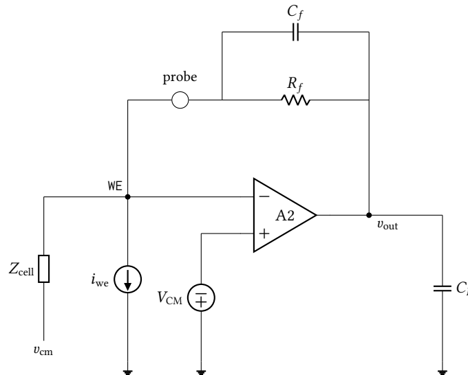
Figure 39: The closed transimpedance loop bench, the only one in this section that closes feedback around the electrode. R_f \parallel C_f returns the output to the working electrode through a current probe, i_{we} is the test source, and Z_{cell} is the Randles cell of Figure 13, returned to v_{cm} . The loop gain, phase margin and crossover are measured through the probe; the DC accuracy, closed-loop transfer and noise figures come from the same wiring.
