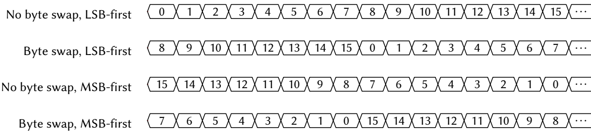
Figure 51: SPI Bit Ordering (16-bit transfer)
