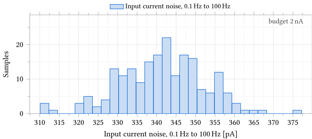
Figure 44: Input-referred current noise integrated 0.1 Hz to 100 Hz, conditions as Figure 42. Output noise divided by R_f , from a noise analysis that runs 0.1 Hz to 10 kHz at 20 points per decade. The 2 nA budget entered on the test is about six times the measured value and is annotated at the axis edge rather than drawn, so that the 310 pA to 377 pA spread stays legible. The figure scales inversely with the selected gain tap.
