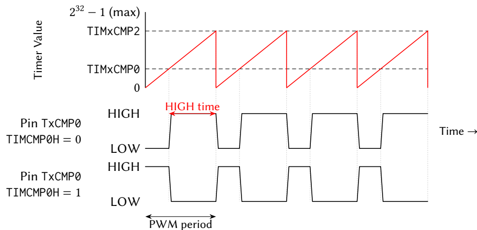
Figure 56: Timer Output Compare and PWM Operation
