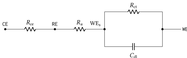
Figure 9: Three-electrode cell model randles_cell, the load the potentiostat actually drives. R_{ce} is the solution resistance from the counter to the reference electrode and R_u the uncompensated resistance from the reference to the working-electrode surface; the interface itself is the charge-transfer resistance R_{ct} in parallel with the double-layer capacitance C_{dl} . Values are given in Table 8. The model is lumped, linear and frequency-independent — no Warburg diffusion term and no potential dependence — so it represents small-signal behaviour about a bias point rather than a full electrochemical response.
