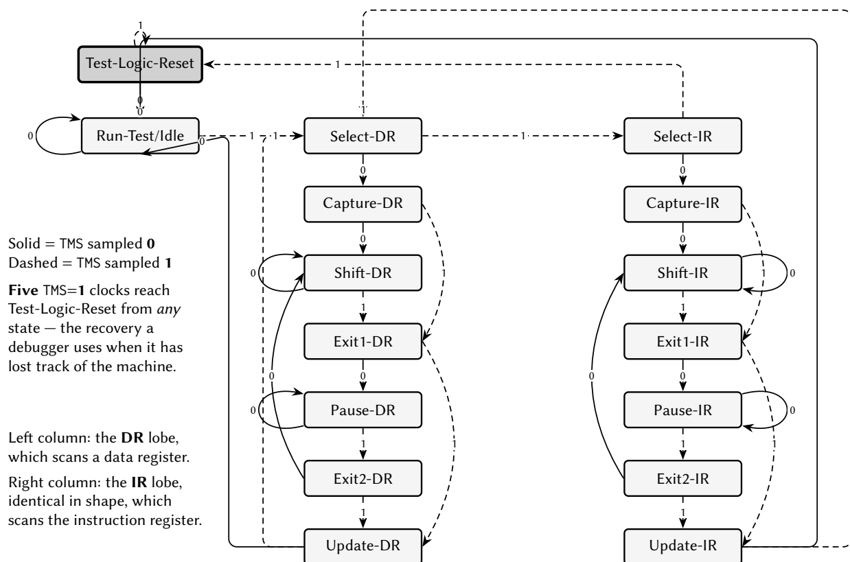
Figure 6: The sixteen-state JTAG test access port. Solid arrows are taken when TMS is sampled low, dashed when it is sampled high; the two lobes are identical in shape, one scanning a data register and one the instruction register. Note that five consecutive high samples reach Test-Logic-Reset from every state in the graph, which is the recovery a debugger uses when it does not know where the machine is.
