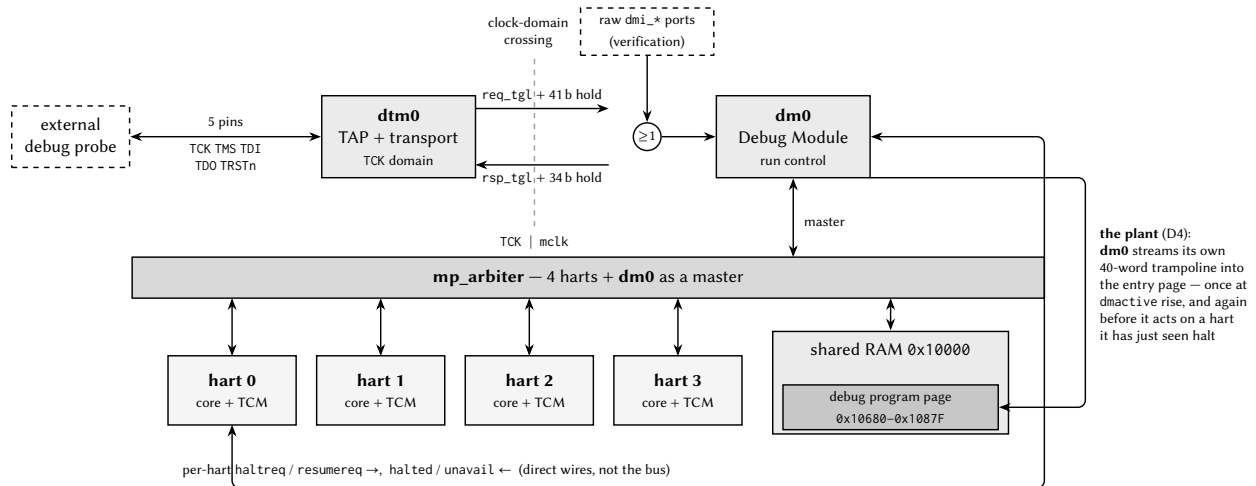
Figure 8: The debug path, from the probe to a hart, in a configuration built with debug support. The transport and the Debug Module sit in different clock domains , and the boundary between them is crossed by exactly two signals — one toggle each way, each carrying a payload that is held still while the toggle is in flight. Everything else in the picture is ordinary chip fabric: the Debug Module reaches memory as one more master on the same arbiter the harts use, and reaches the harts themselves over a small number of direct wires. The count of hart tiles follows this configuration.
