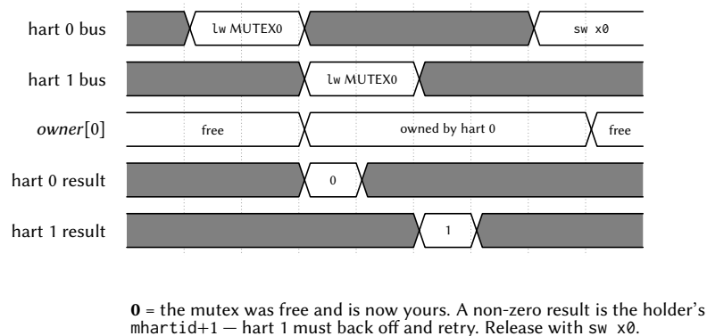
Figure 17: Two harts racing for the same mutex. The arbiter serializes the two claim reads, so the return-old-and-claim happens atomically with no retry loop: hart 0 reads 0 and thereby owns the mutex, and hart 1 reads hart 0's marker and must back off.
