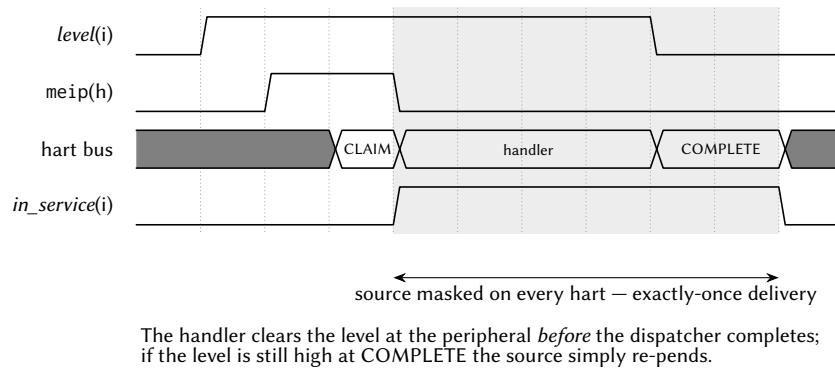
Figure 18: Claim/complete delivery of one peripheral interrupt. The router raises meip while the source is pending and enabled; the CLAIM read marks it under service, which hides it from every hart until the completing write. That masking window is what makes delivery exactly-once even when several harts enable the same source.
