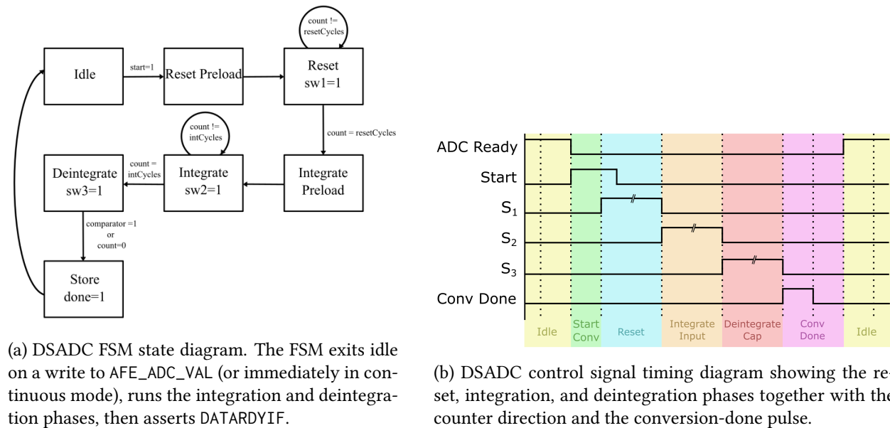
Figure 17: DSADC finite state machine and timing signals.
