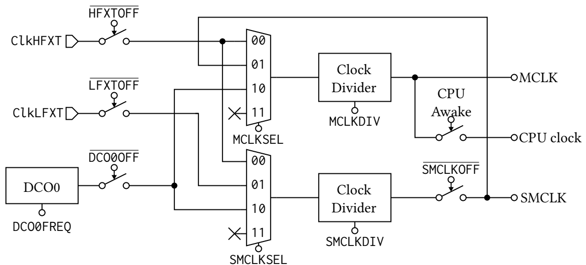
Figure 13: MCU Clock System
