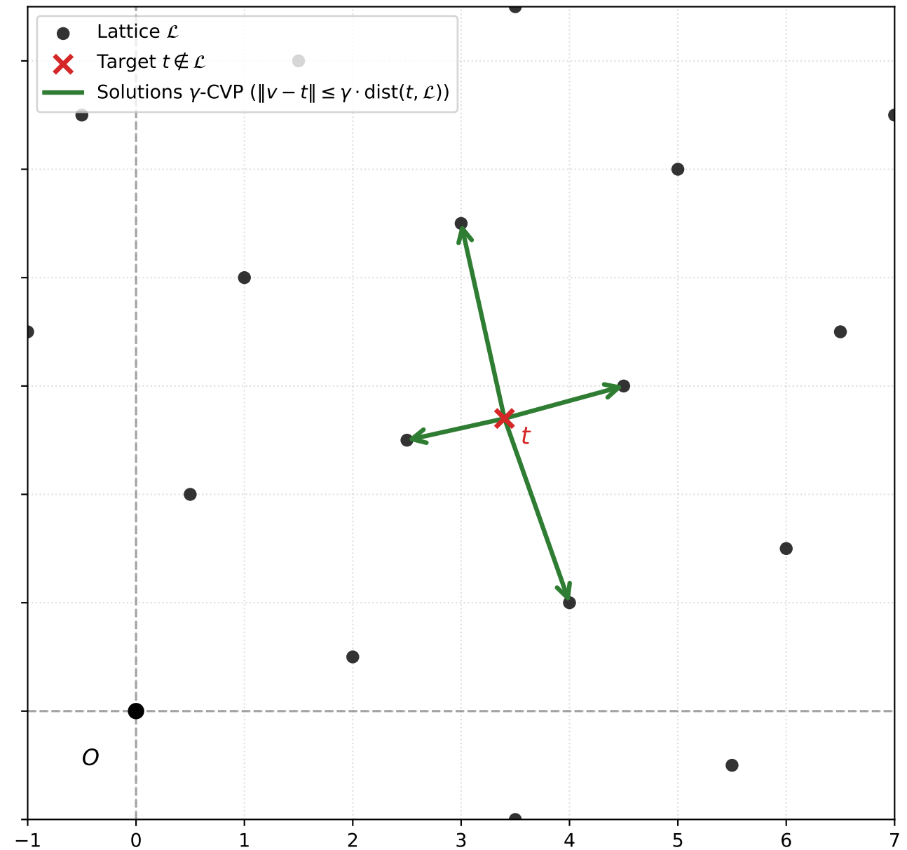
apprCVP Solution (Approximate)
