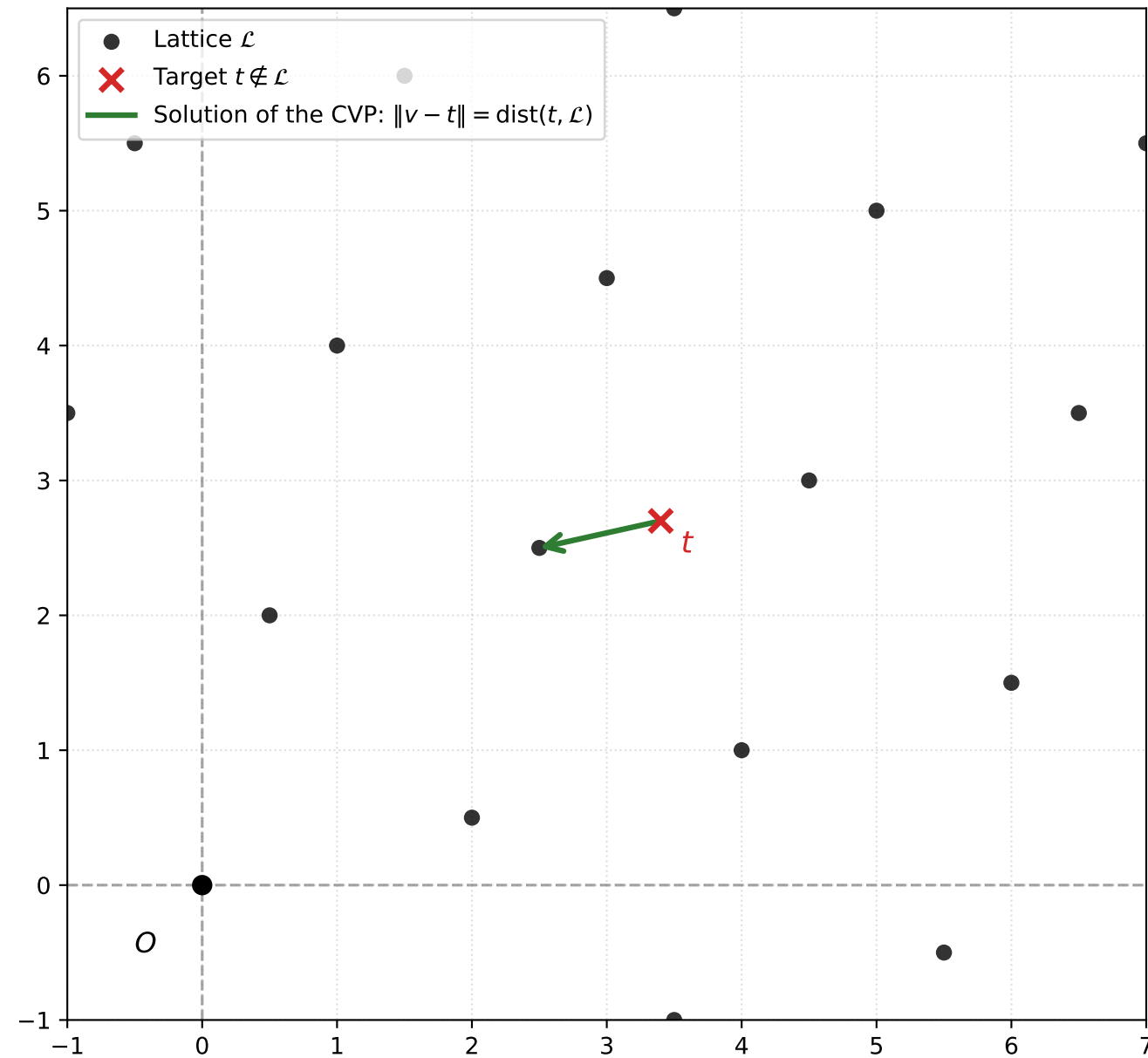
CVP Solution (Exact)
