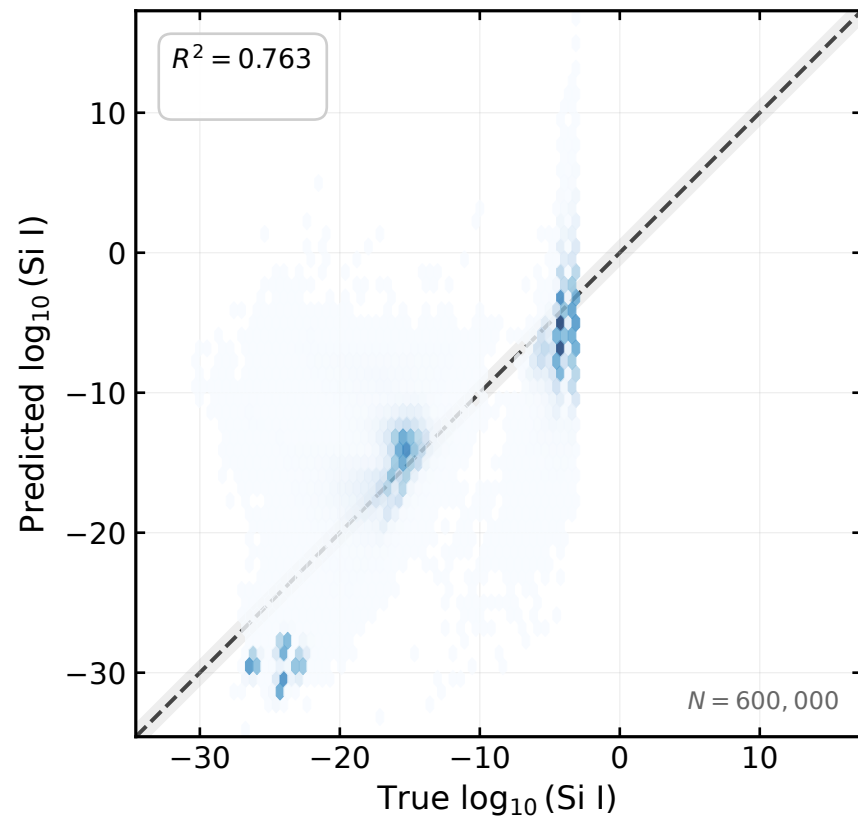
Ridge (LOSO median R^2=0.754 )
