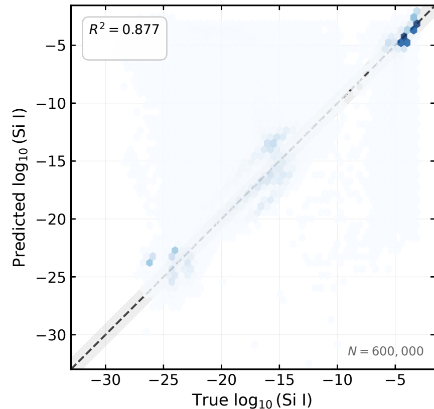
Neural Network (LOSO median R^2=0.846 )
