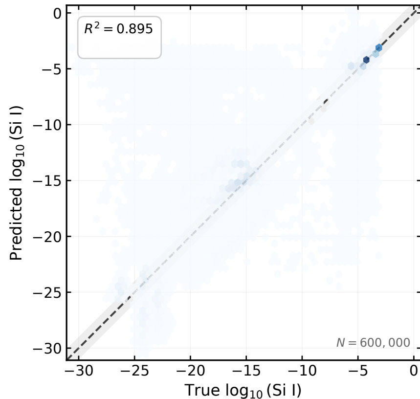
Gradient Boosting (LOSO median R^2=0.879 )
