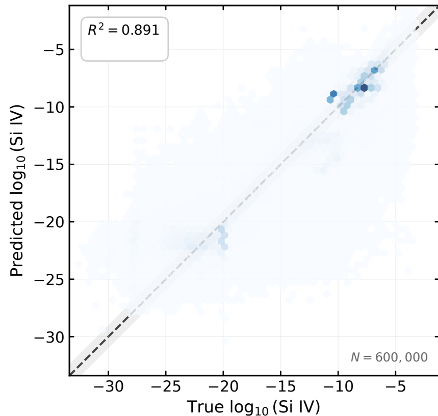
Gradient Boosting (LOSO median R^2=0.867 )
