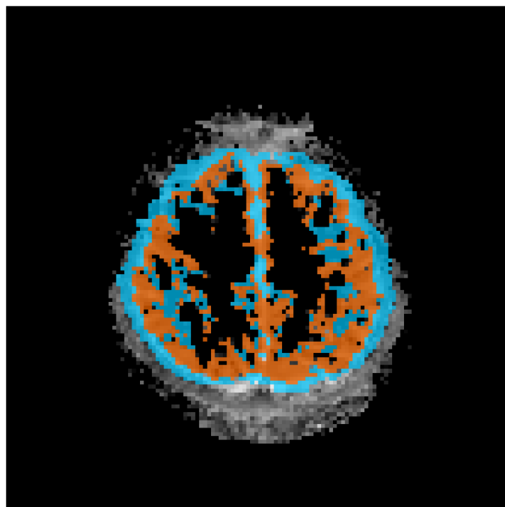
Segmentation overlay
