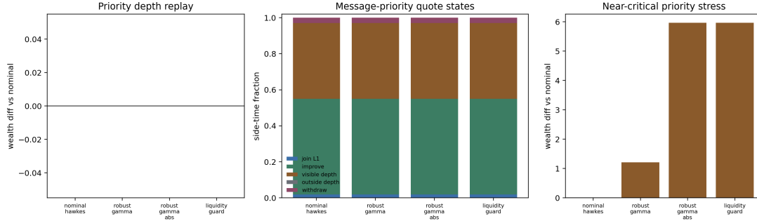
Figure 9: Residual-volume priority-aware level-10 LOBSTER quote replay. Same-price orders arriving after the synthetic quote are tracked behind it, queued fills require residual execution volume after displayed queue-ahead depletion, and partial fills are credited by residual lots.
