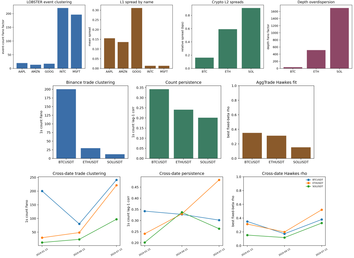
Figure 16: Public-data sanity figures, including Binance aggregate-trade event clustering, fixed-beta Hawkes diagnostics, and cross-date robustness.
