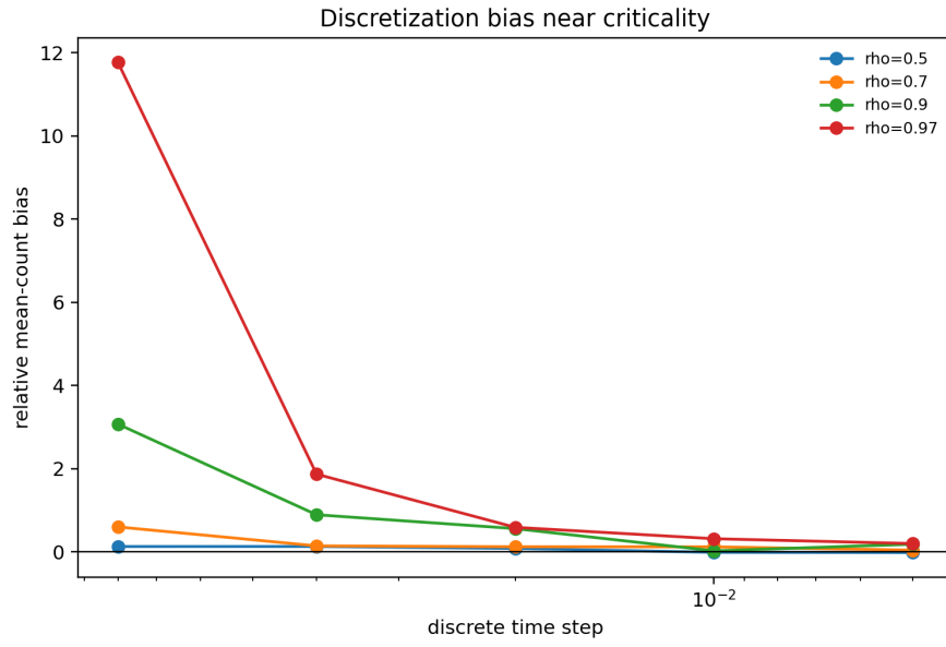
Figure 12: Time-discretization bias grows sharply near criticality.
