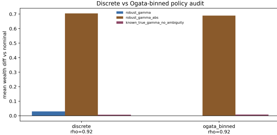
Figure 4: Focused policy audit under fast discrete arrivals and Ogata-binned event arrivals.
