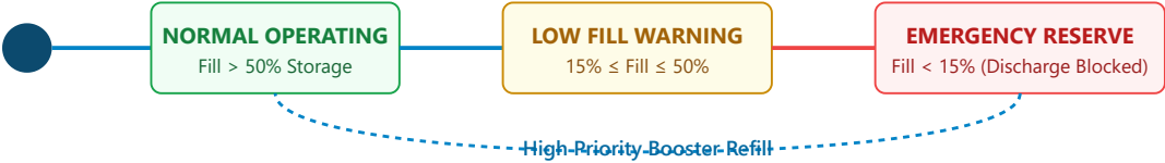
Figure 8.5: Reservoir State Machine Lifecycle Transition Diagram
