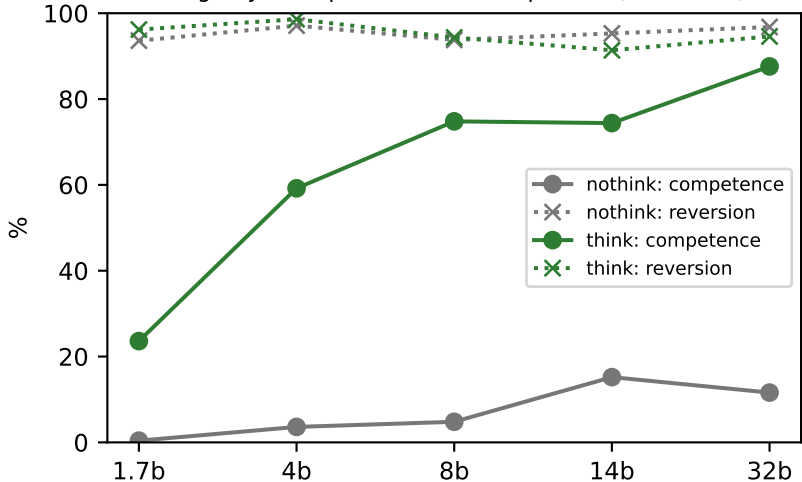
Reasoning buys competence, not compliance (contour, Qwen3)
