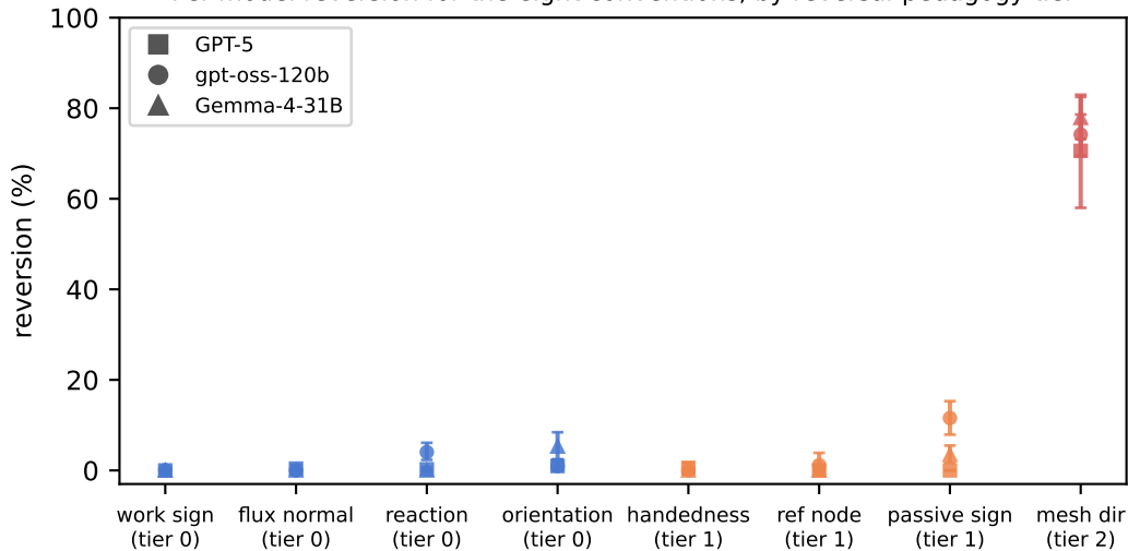
Per-model reversion for the eight conventions, by reversal-pedagogy tier
