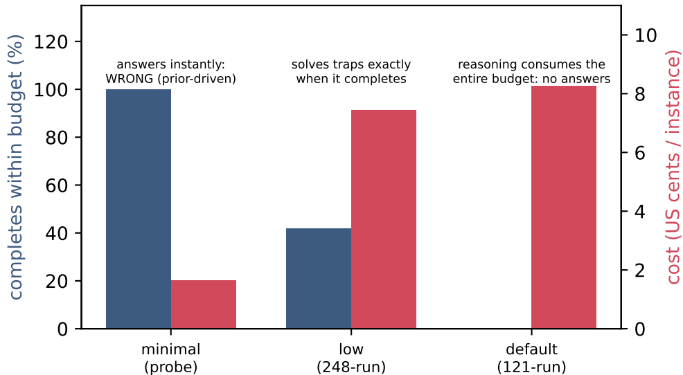
GPT-5 reasoning-effort ladder on CircuChain v2
