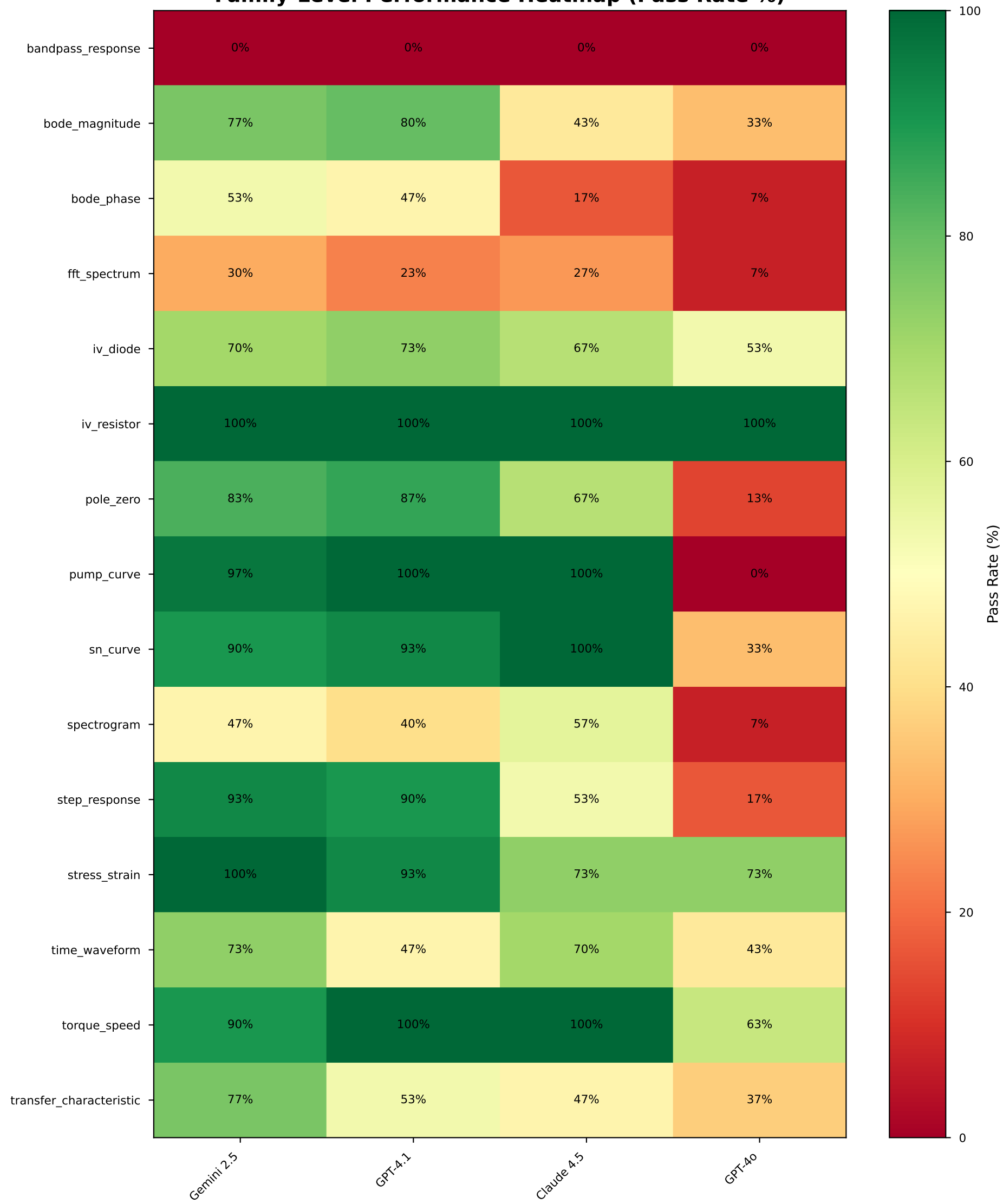
Family-Level Performance Heatmap (Pass Rate %)
