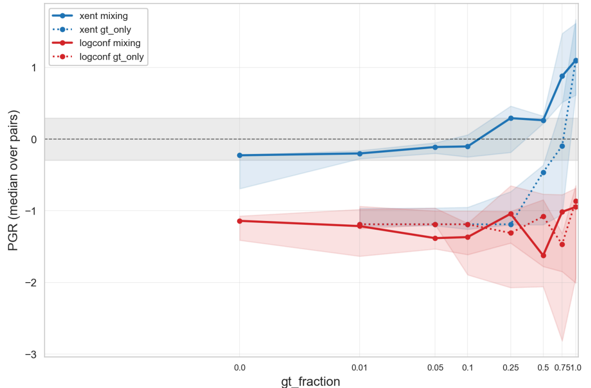
Phase 1 — Supervision scaling: PGR vs gt_fraction (3-seed, BoolQ) solid=mixing, dotted=GT-only, blue=xent, red=logconf; shaded=seed range, gray=noise floor
